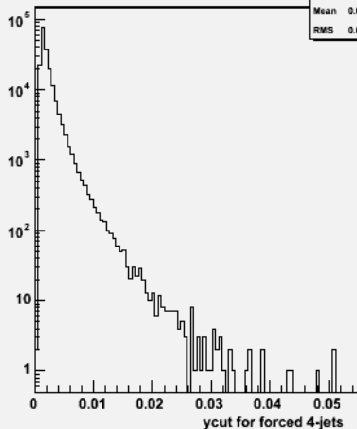
Ycut for 4-jets :w102789 aa_dd_o
