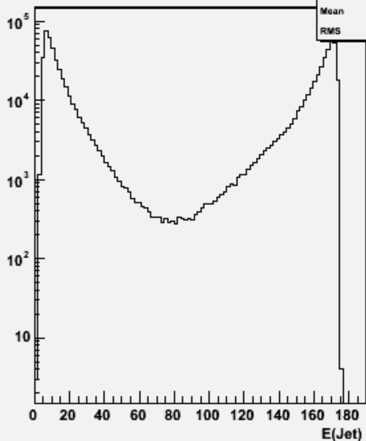
Jet energies(All jets)w102789 aa_dd_o
