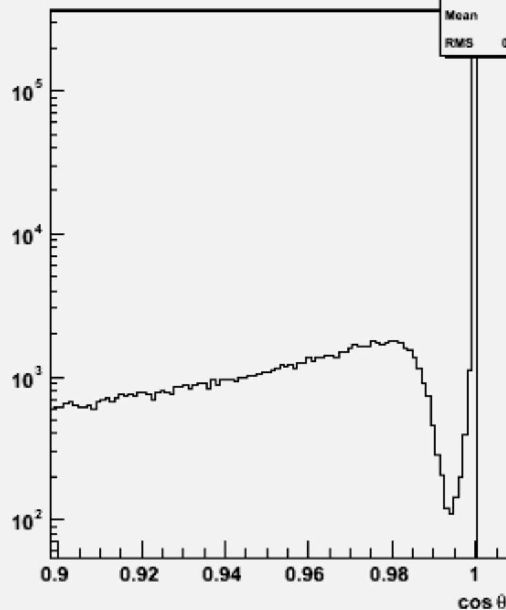
Jet cos \theta (All jets)w102789 aa_dd_o
