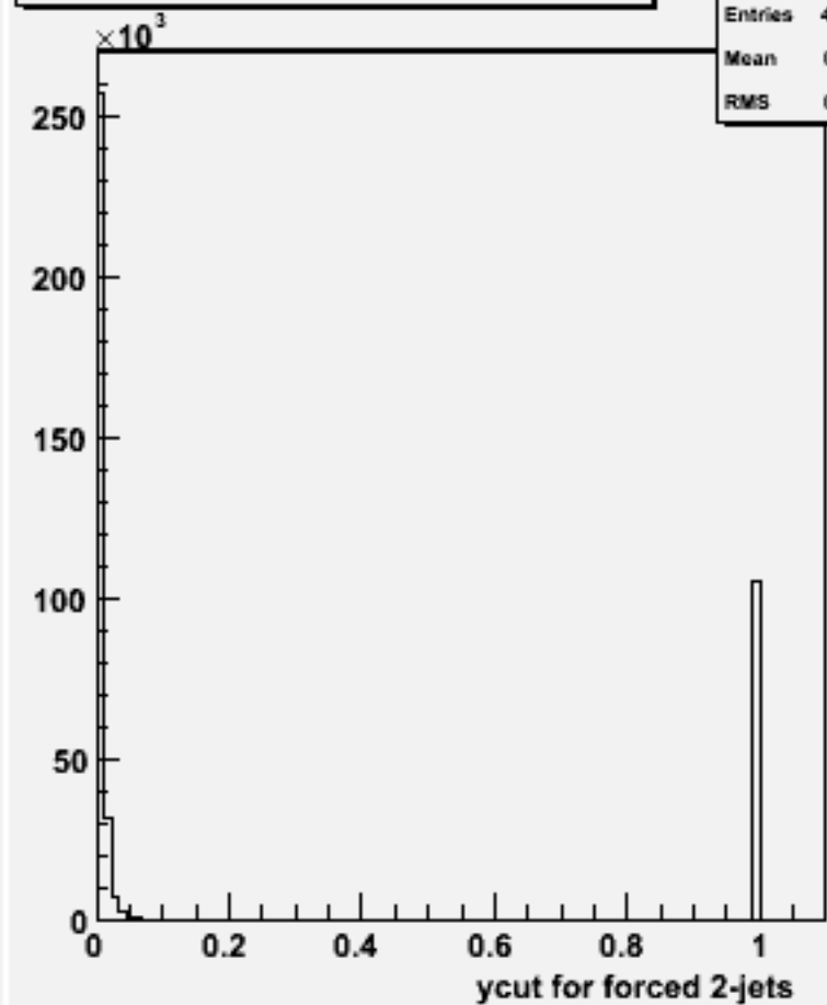
Ycut for 2-jets :w102789 aa_dd_o
