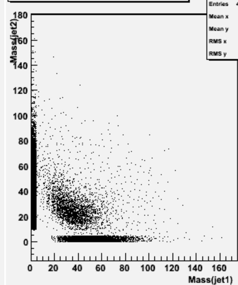
Jet mass for forced 2-jets : w102789 aa_dd_o
