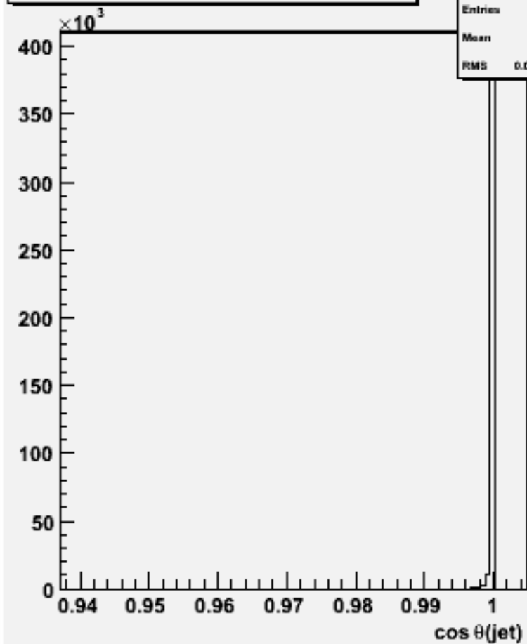
cos \theta for 2-jets :w102789 aa_dd_o
