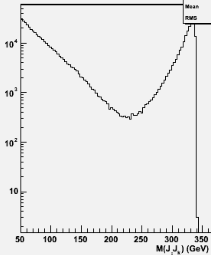
2jets mass(All comb)w102789 aa_dd_o
