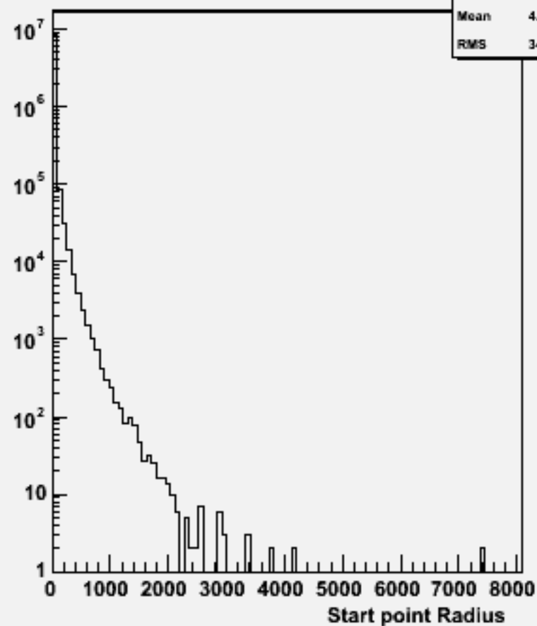
Start point R : w102789 aa_dd_o
