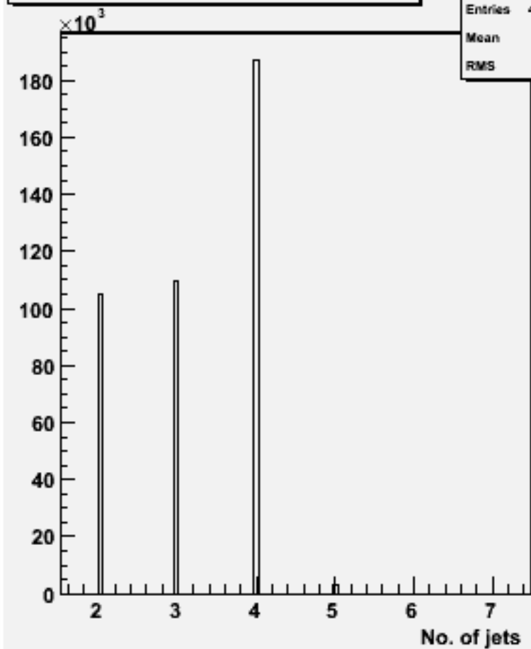
No. jets (ycut=0.001) : w102789 aa_dd_o
