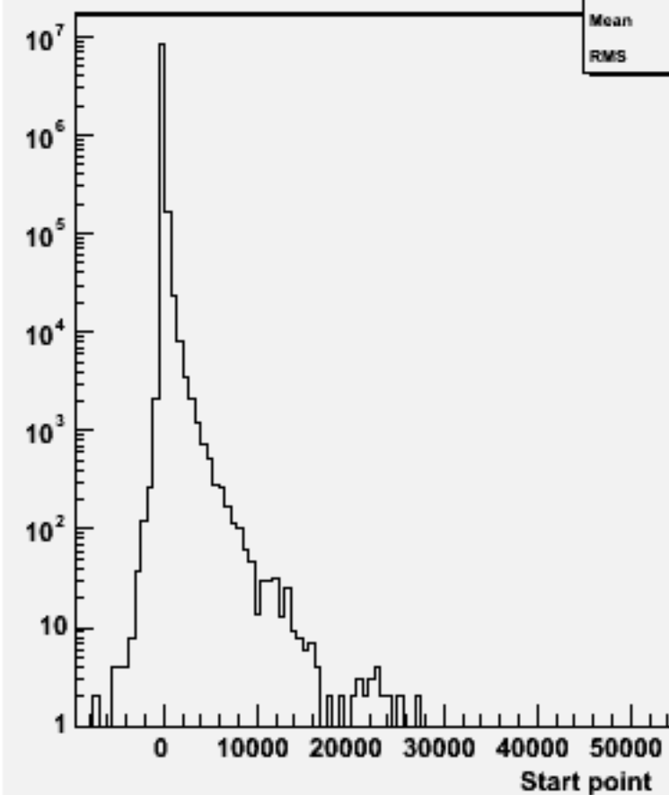
Start point Z : w102789 aa_dd_o
