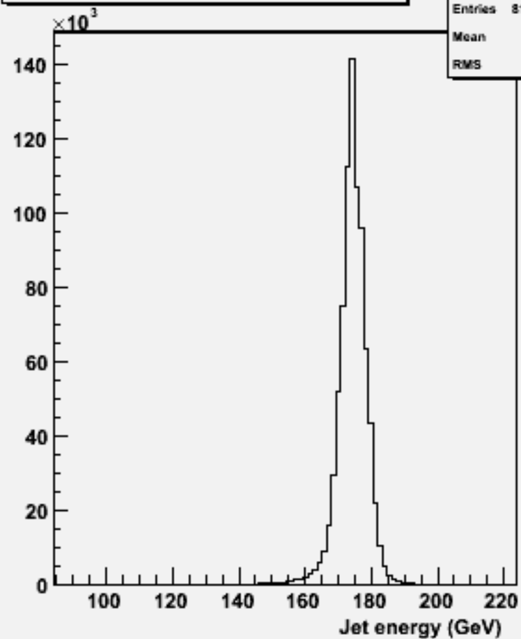
energy for 2-jets :w102789 aa_dd_o
