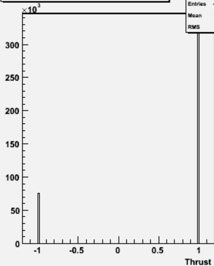
cos \Theta (thrust) w102789 aa_dd_o
