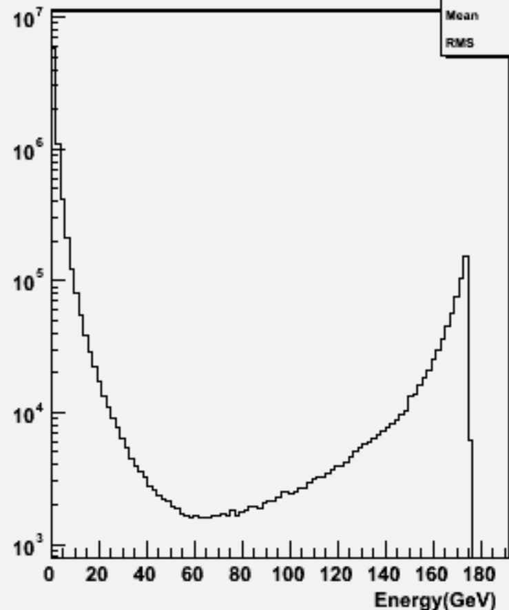
Particle Energy : w102789 aa_dd_o
