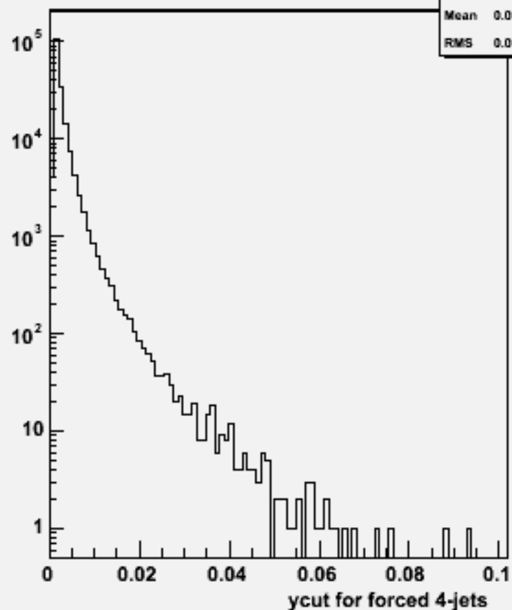
Ycut for 4-jets :w102788 aa_dd_o
