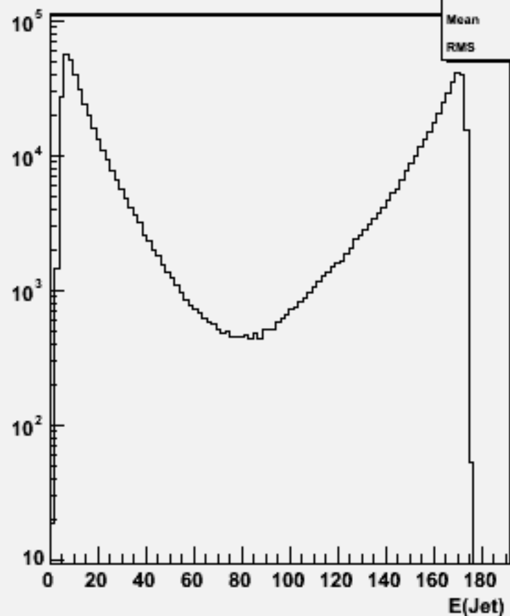
Jet energies(All jets)w102788 aa_dd_o
