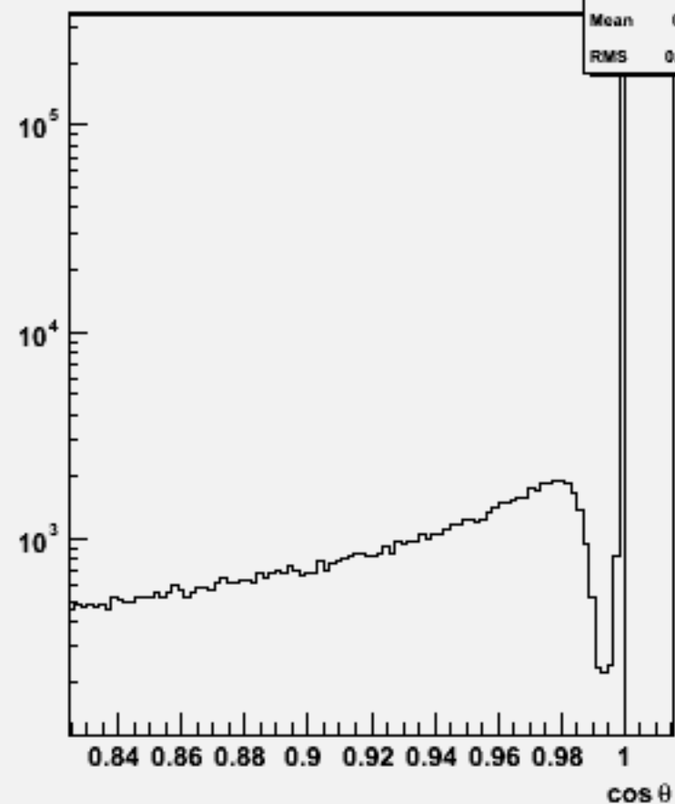
Jet cos \theta (All jets)w102788 aa_dd_o
