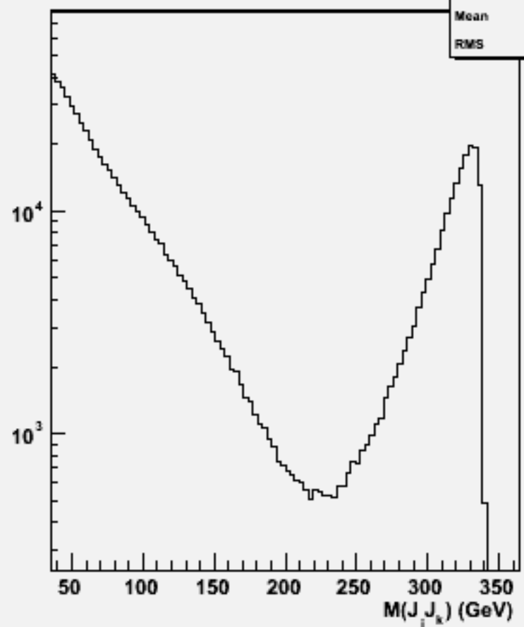
2jets mass(All comb)w102788 aa_dd_o
