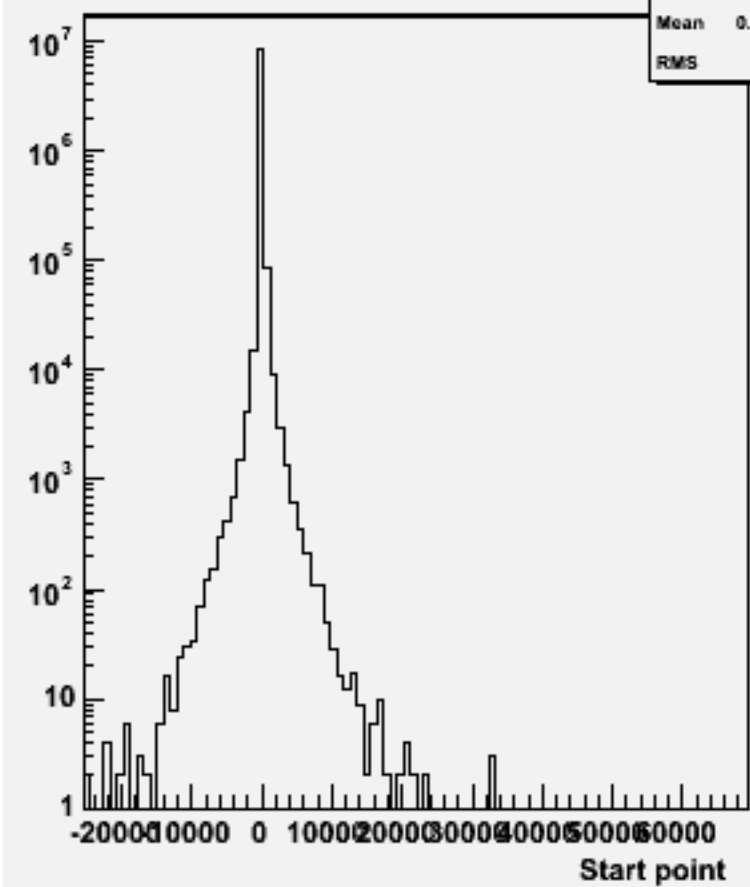
Start point Z : w102788 aa_dd_o
