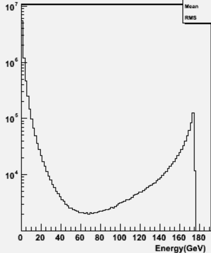
Particle Energy : w102788 aa_dd_o
