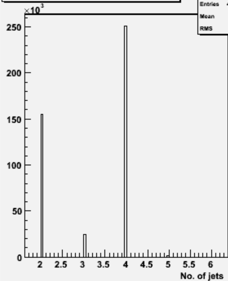
No. jets (ycut=0.001) : w102787 aa_uu_o
