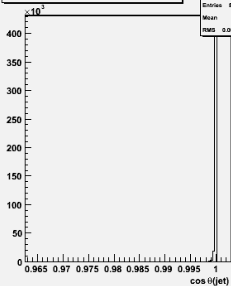
cos \theta for 2-jets :w102787 aa_uu_o
