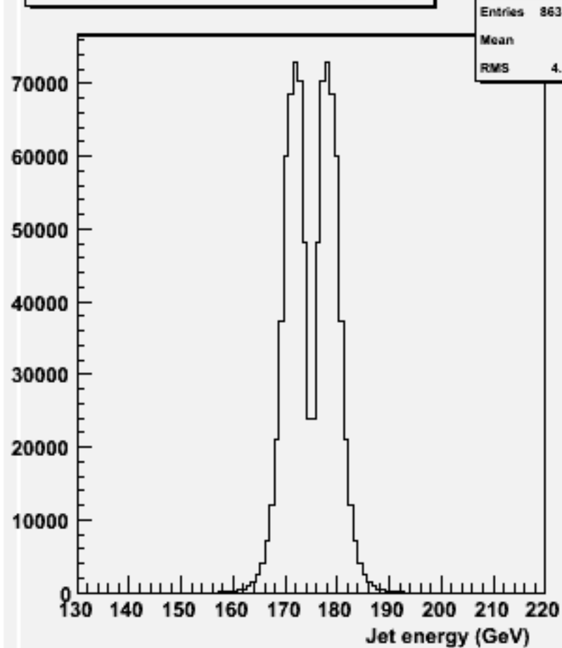
energy for 2-jets :w102787 aa_uu_o
