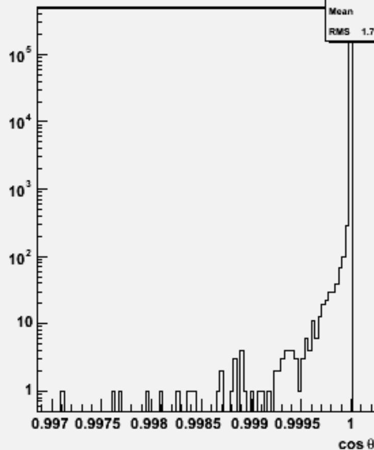
Jet cos \theta (All jets)w102787 aa_uu_o
