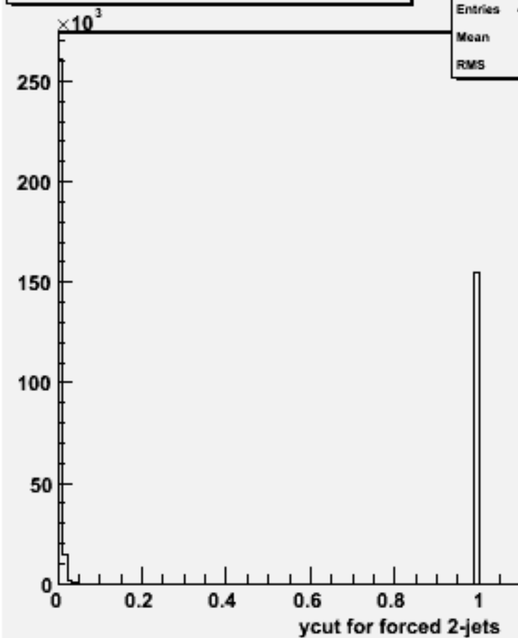
Ycut for 2-jets :w102787 aa_uu_o
