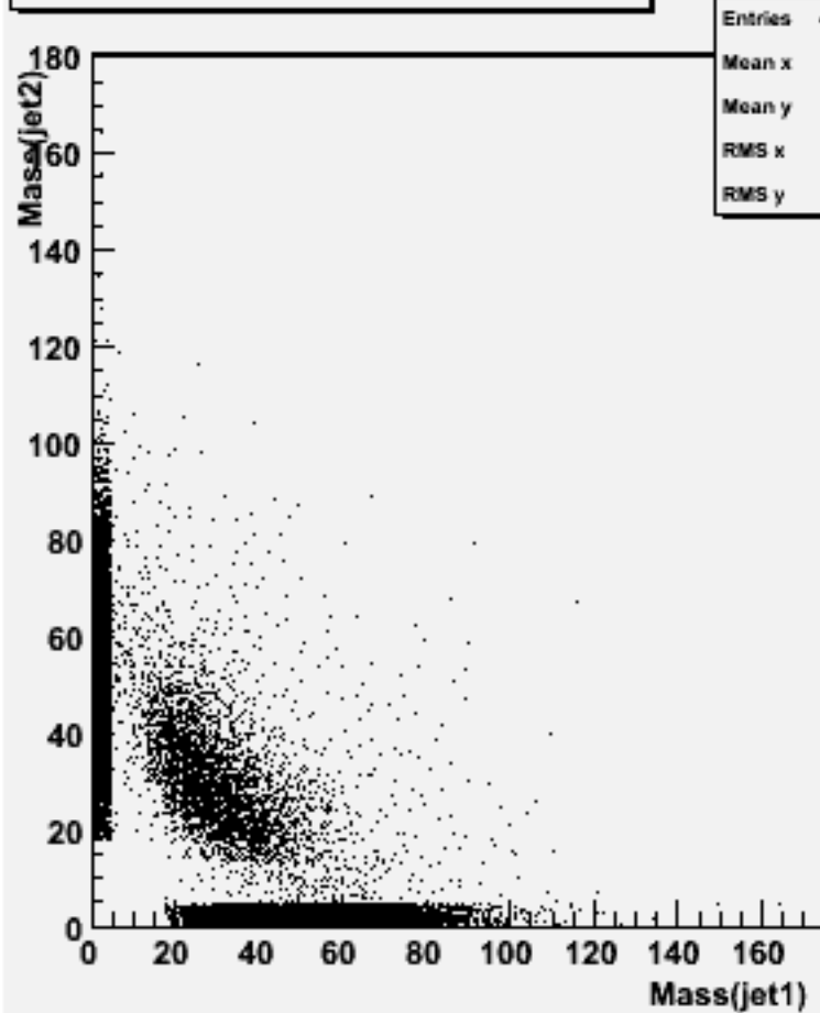
Jet mass for forced 2-jets : w102787 aa_uu_o
