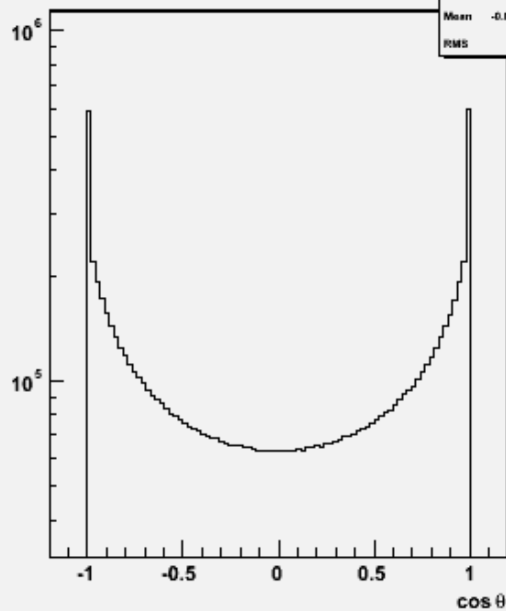
Particle cosθ : w102787 aa_uu_o
