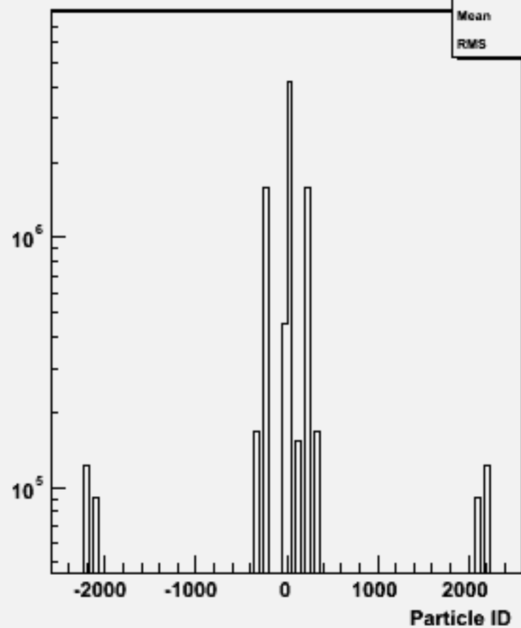
Particle ID : w102787 aa_uu_o
