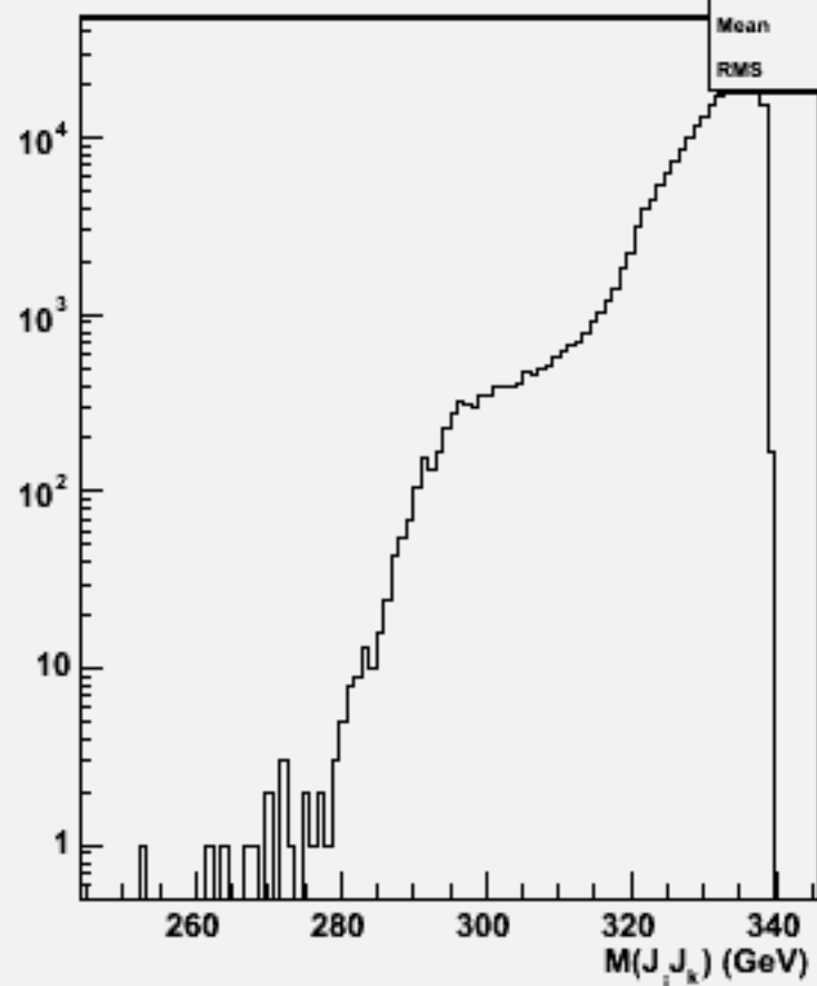
2jets mass(All comb)w102787 aa_uu_o
