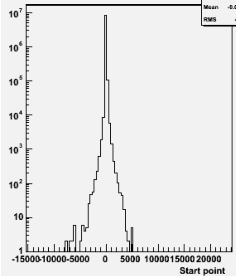
Start point Z : w102787 aa_uu_o
