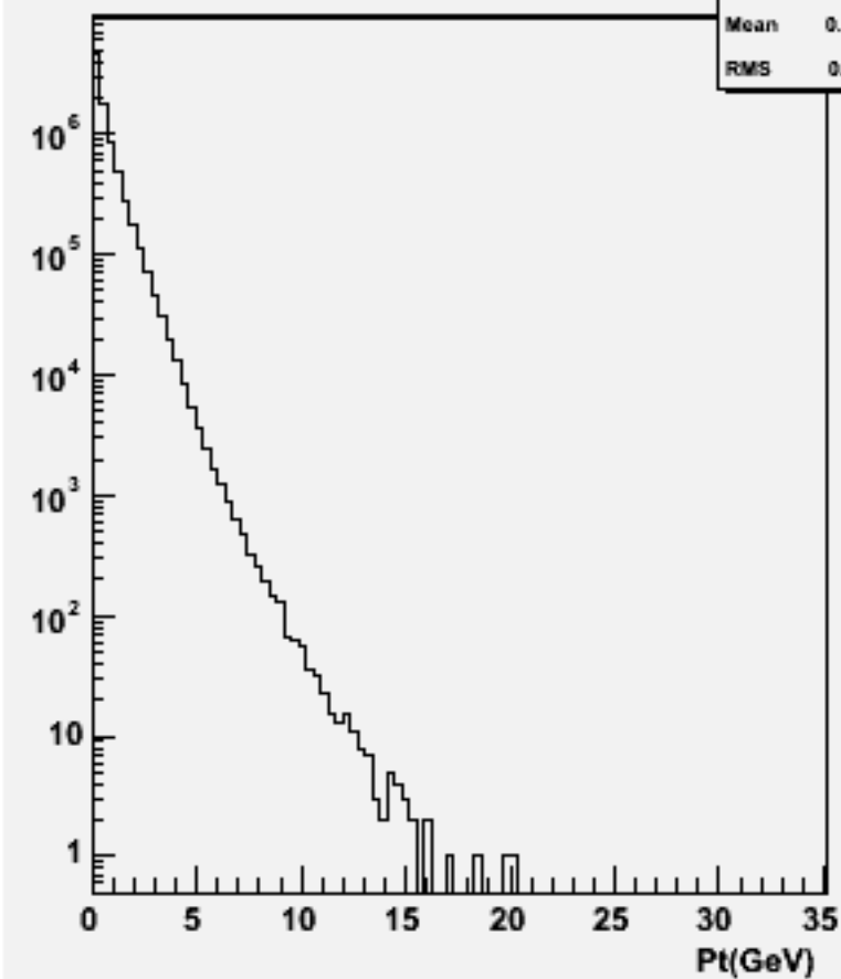
Particle Pt : w102787 aa_uu_o
