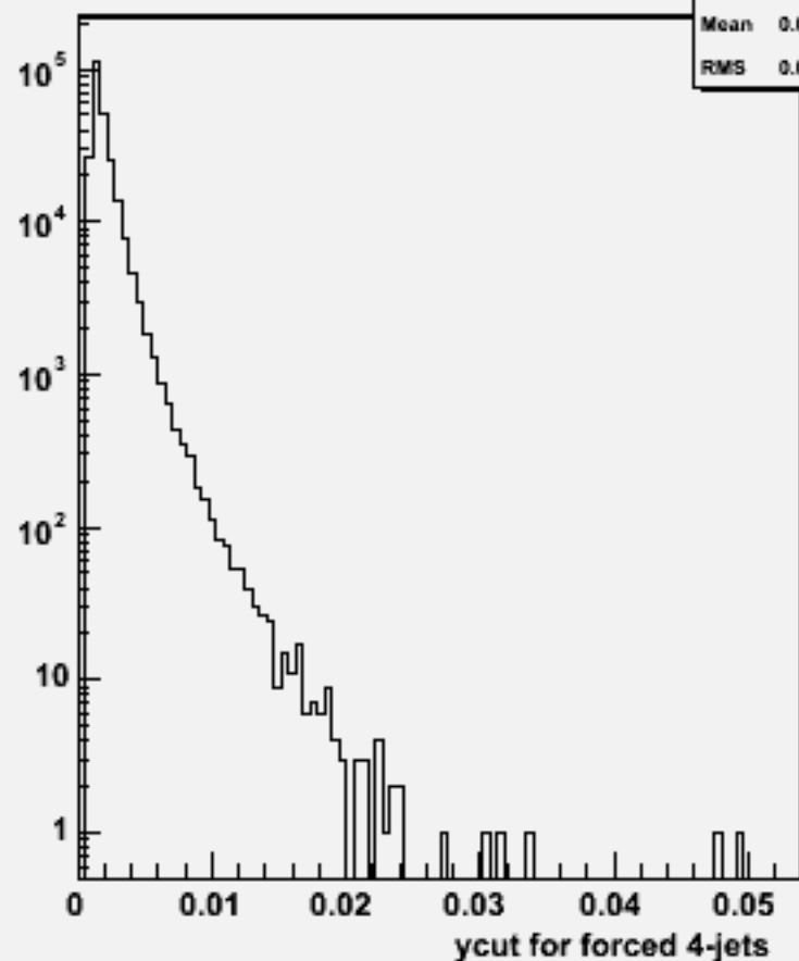
Ycut for 4-jets :w102787 aa_uu_o
