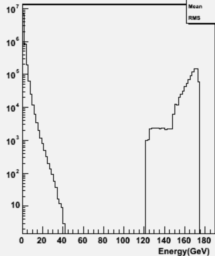
Particle Energy : w102787 aa_uu_o
