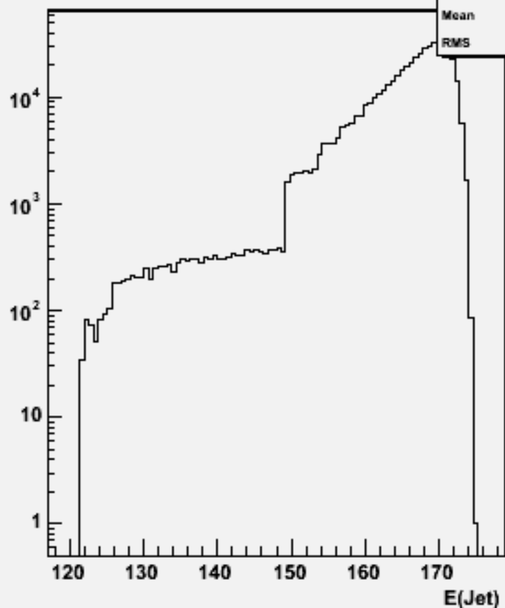
Jet energies(All jets)w102787 aa_uu_o
