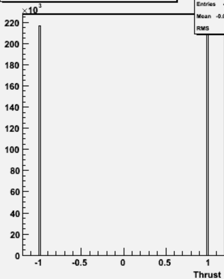
cos \Theta (thrust) w102787 aa_uu_o
