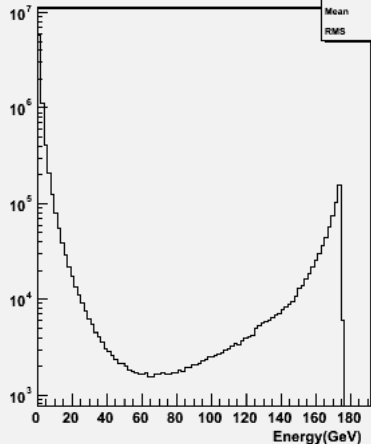
Particle Energy : w102785 aa_uu_o
