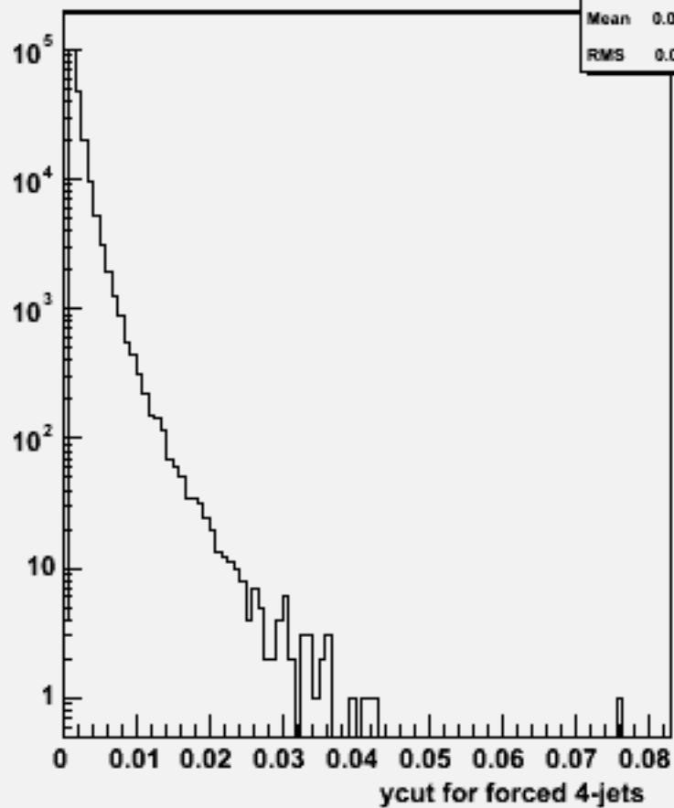
Ycut for 4-jets :w102785 aa_uu_o
