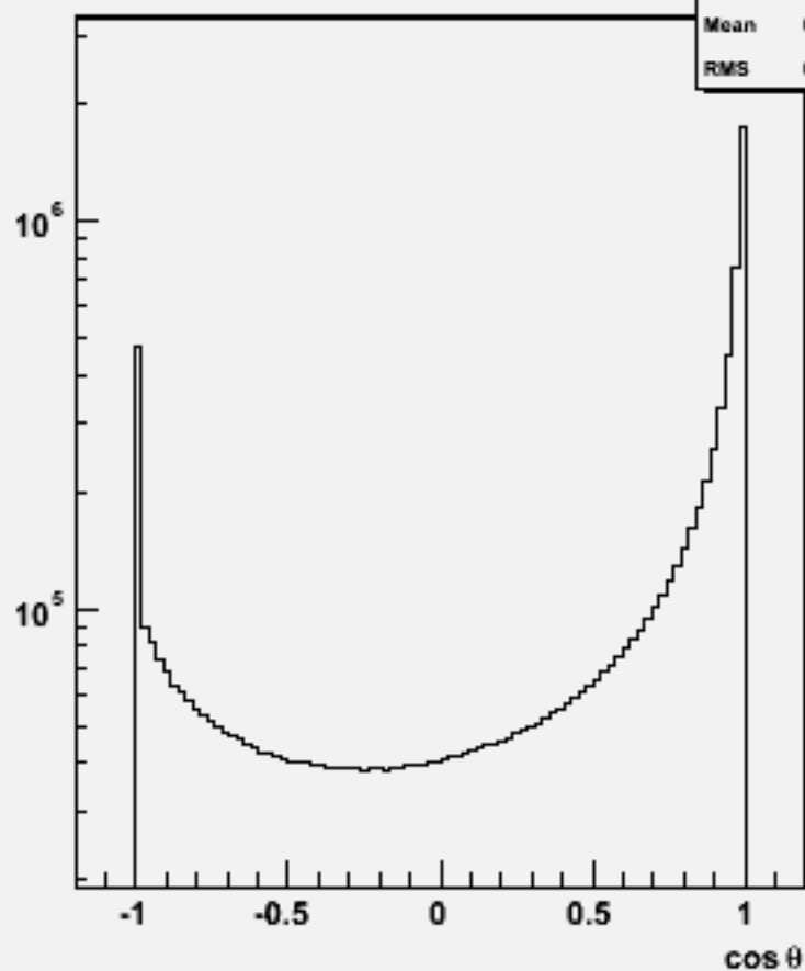
Particle cosθ : w102785 aa_uu_o
