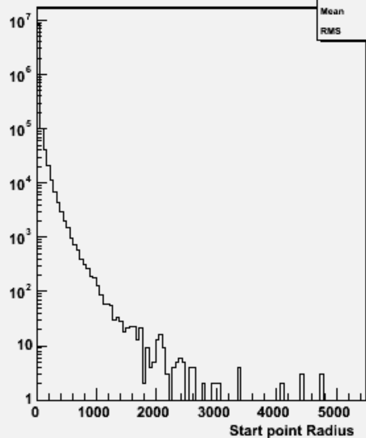
Start point R : w102785 aa_uu_o
