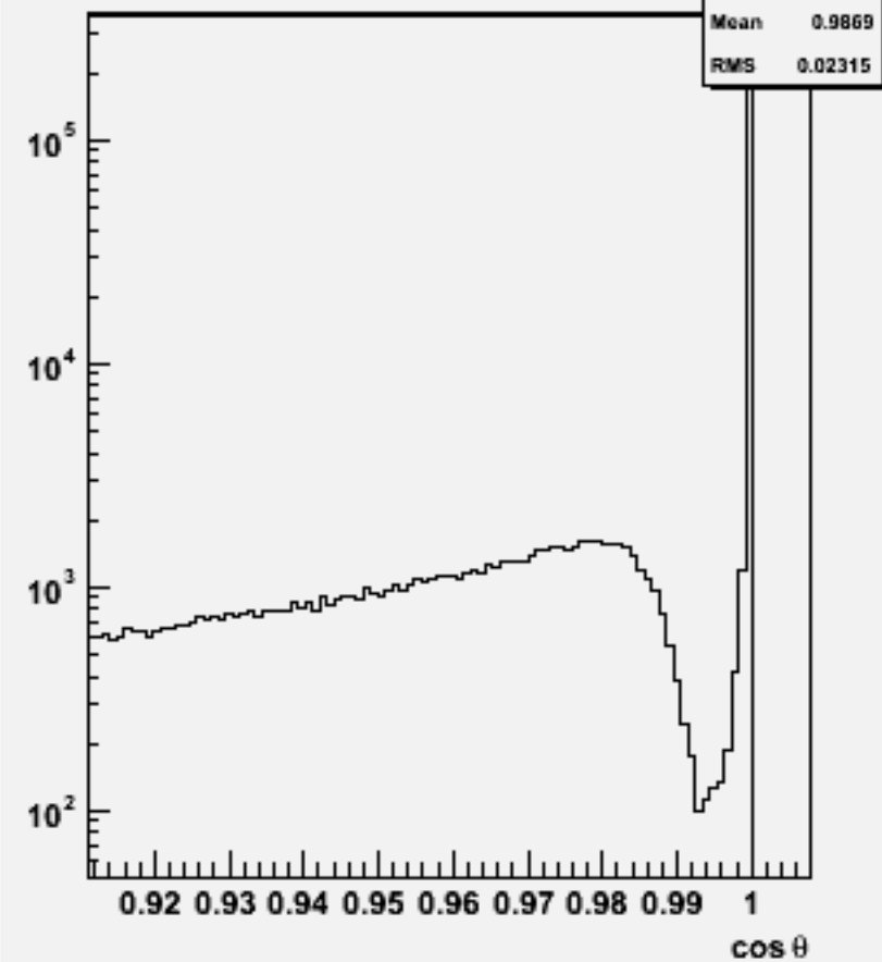
Jet cosθ (All jets)w102785 aa_uu_o
