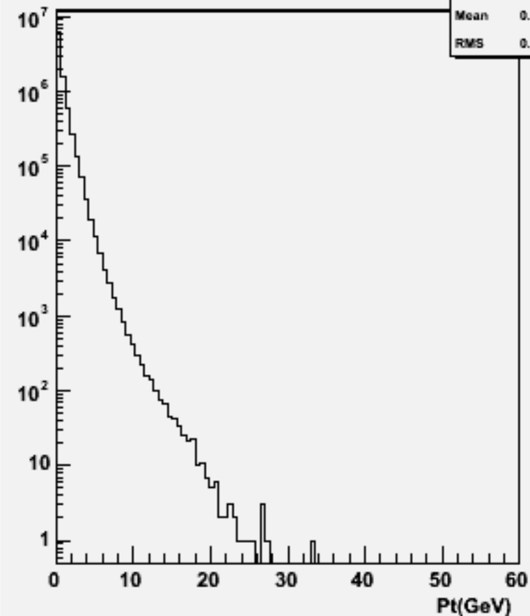
Particle Pt : w102785 aa_uu_o
