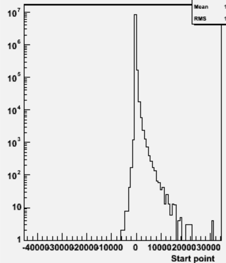
Start point Z : w102785 aa_uu_o
