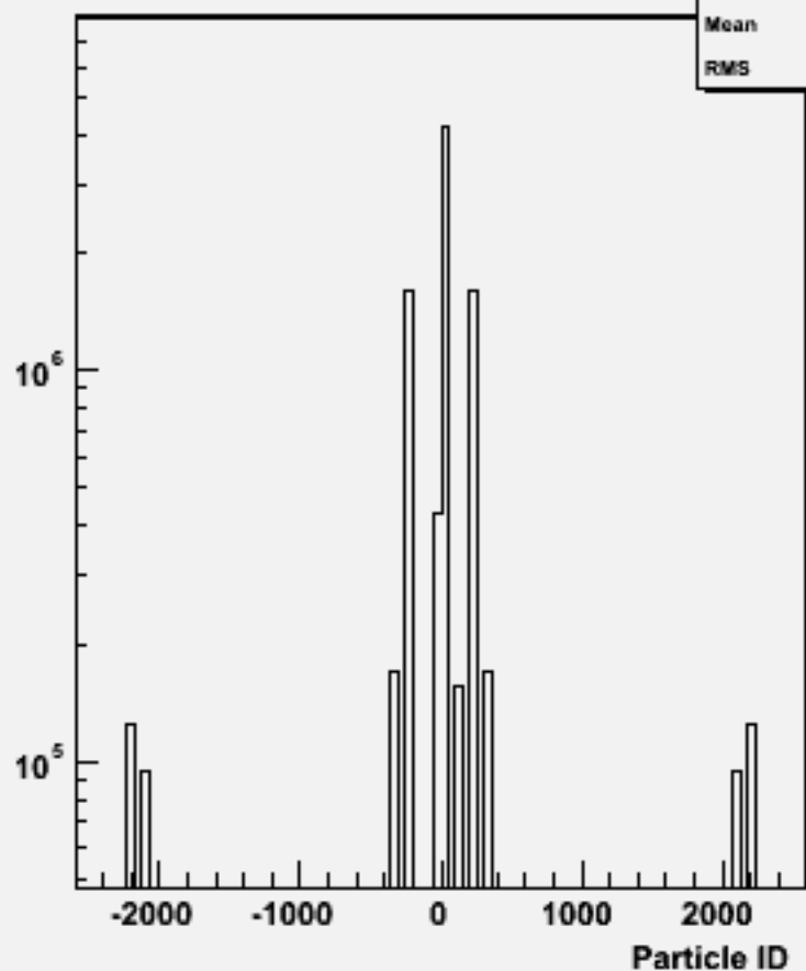
Particle ID : w102785 aa_uu_o
