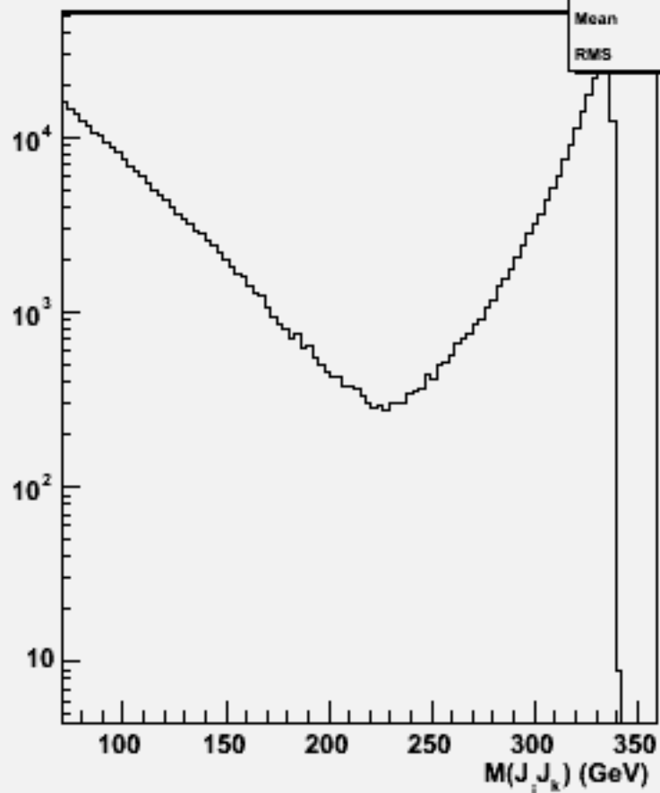
2jets mass(All comb)w102785 aa_uu_o
