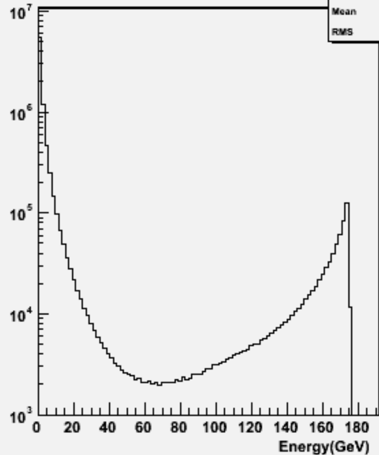
Particle Energy : w102784 aa_uu_o
