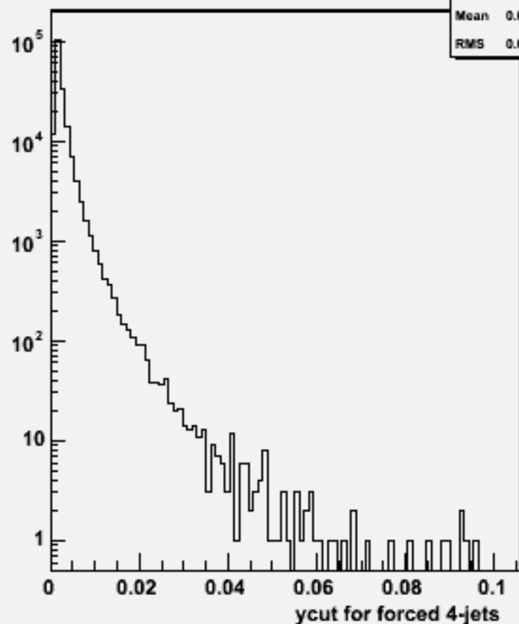
Ycut for 4-jets :w102784 aa_uu_o
