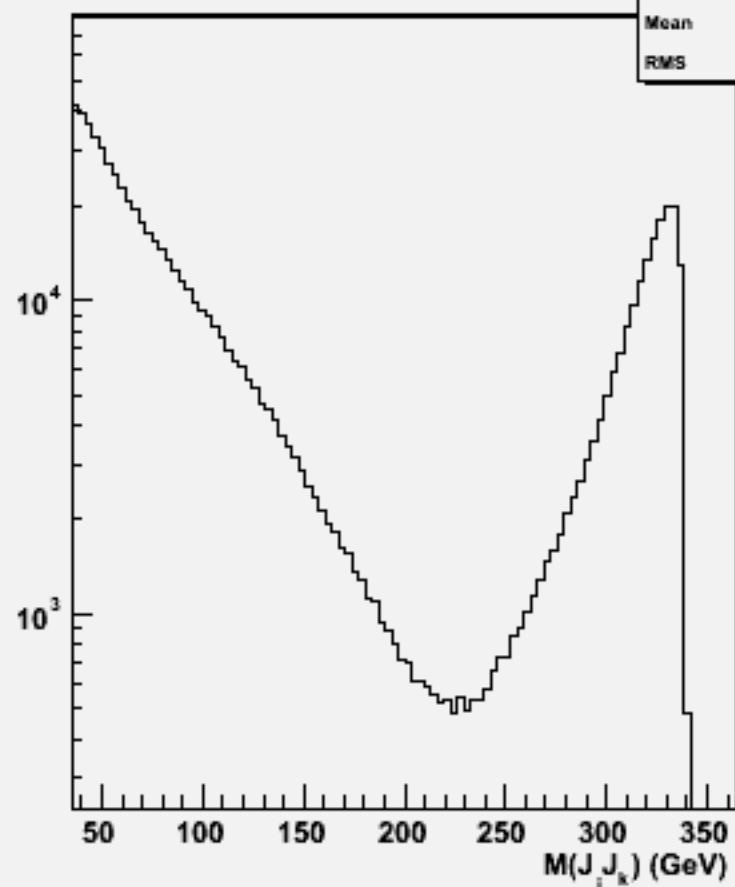
2jets mass(All comb)w102784 aa_uu_o
