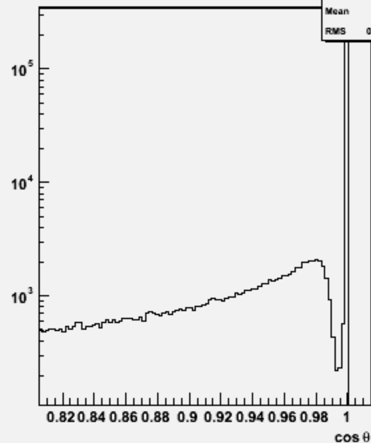
Jet cosθ (All jets)w102784 aa_uu_o
