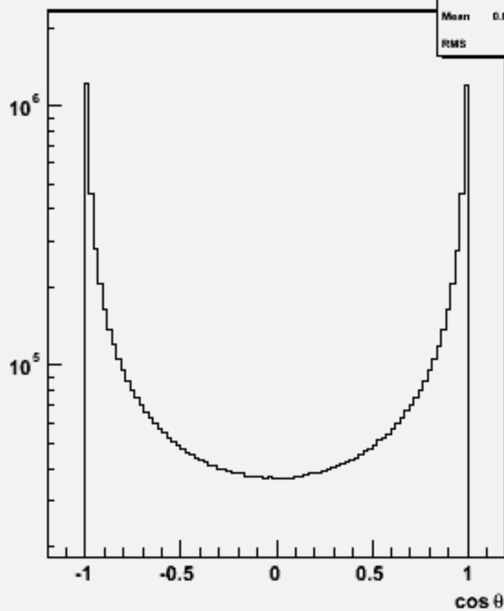
Particle cosθ : w102784 aa_uu_o
