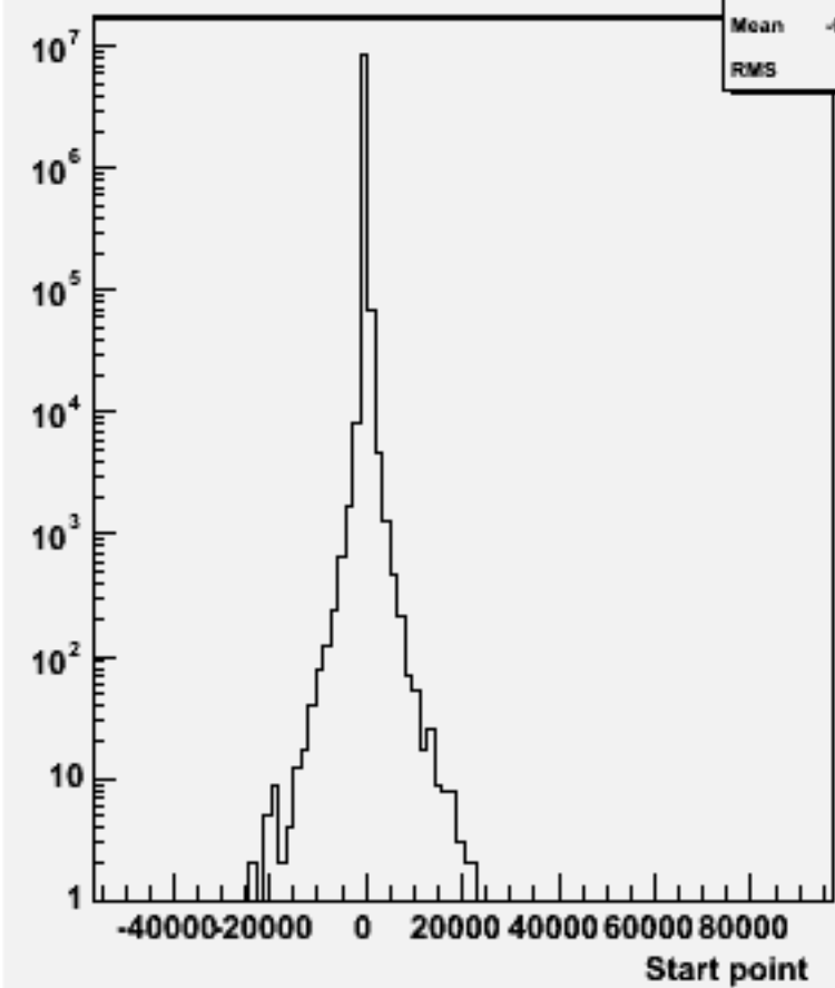
Start point Z : w102784 aa_uu_o
