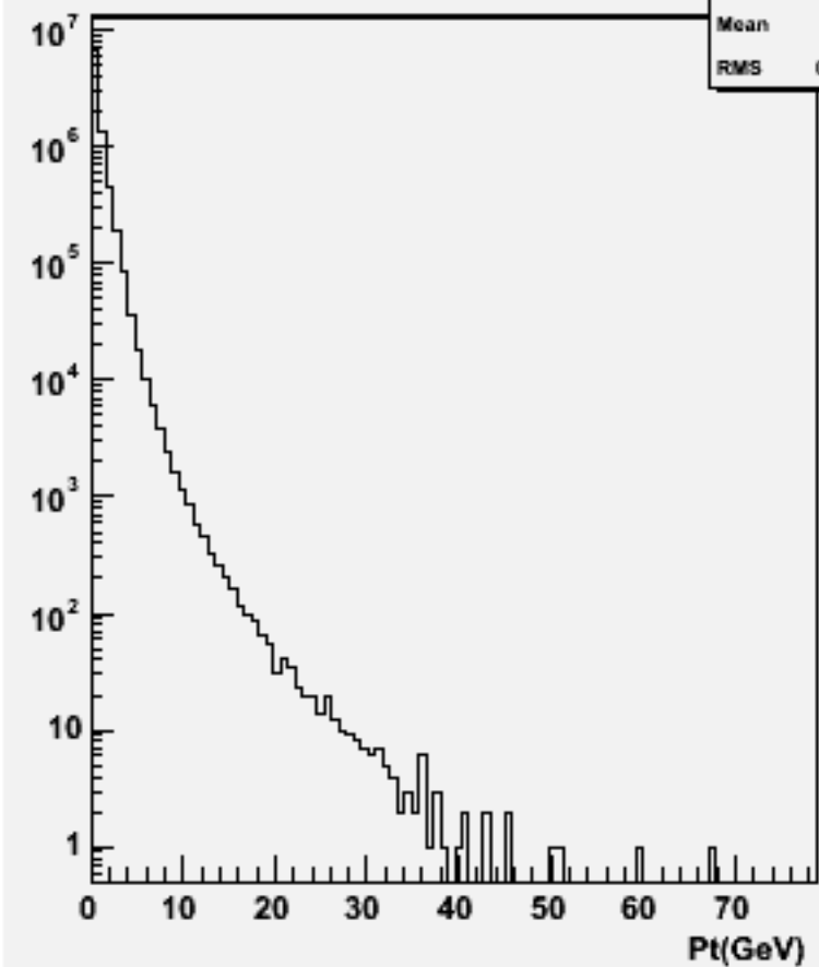
Particle Pt : w102784 aa_uu_o
