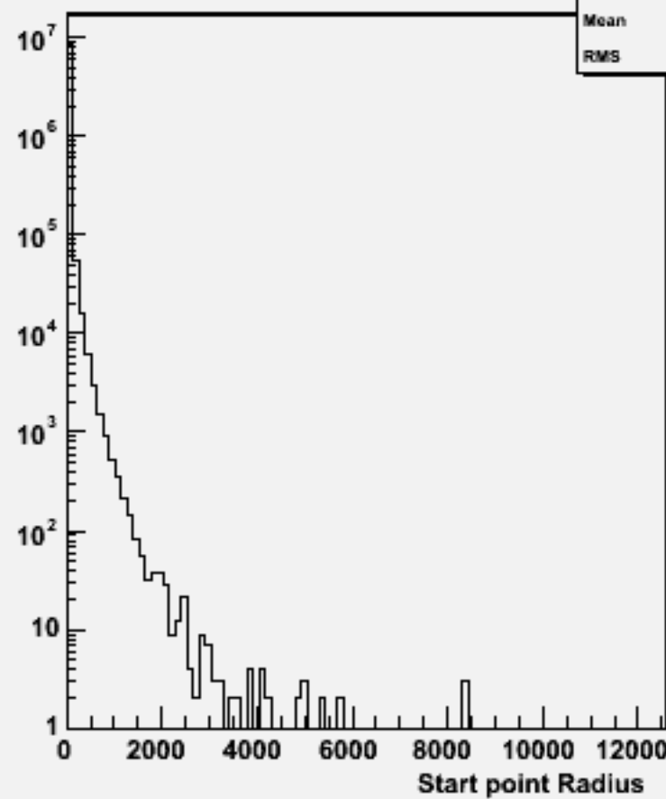
Start point R : w102784 aa_uu_o
