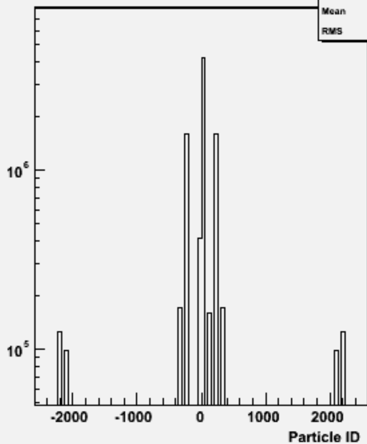
Particle ID : w102784 aa_uu_o
