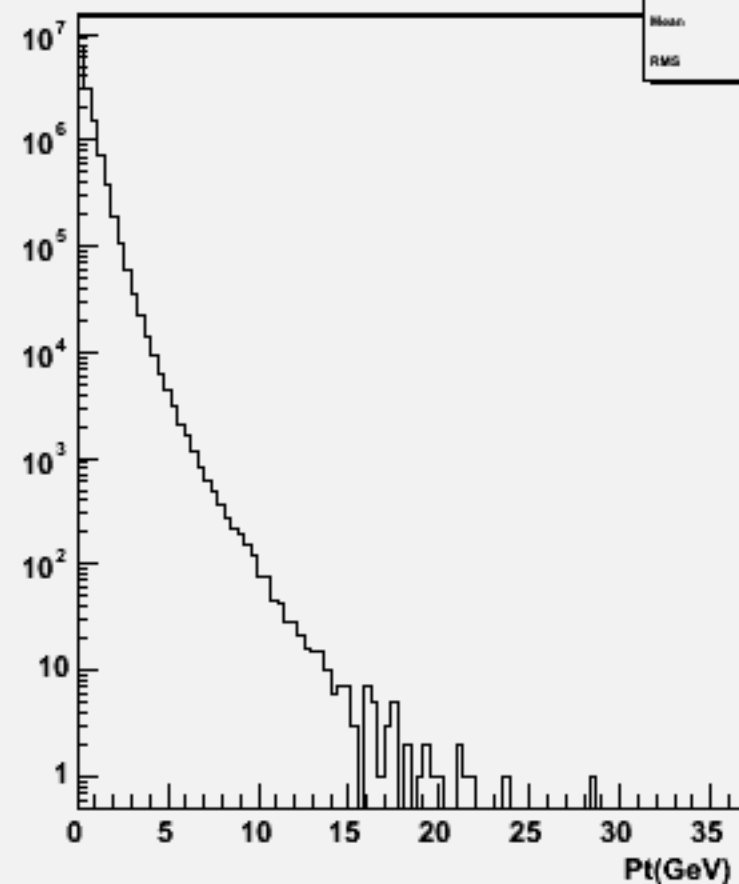
Particle Pt : w102783 aa_e3e3_o
