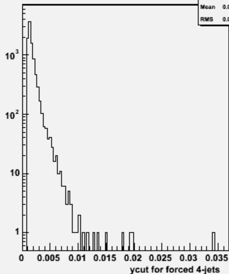
Ycut for 4-jets :w102783 aa_e3e3_o
