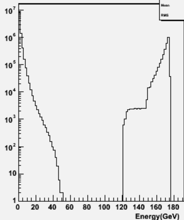
Particle Energy : w102783 aa_e3e3_o
