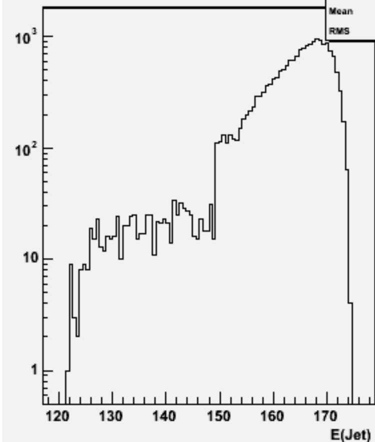
Jet energies(All jets)w102783 aa_e3e3_o
