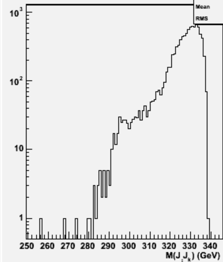
2jets mass(All comb)w102783 aa_e3e3_o
