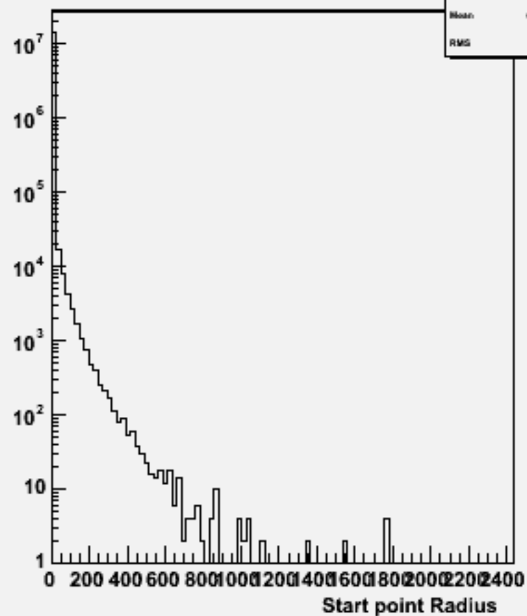
Start point R : w102783 aa_e3e3_o
