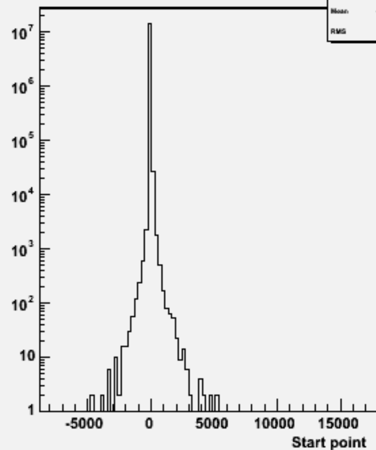
Start point Z : w102783 aa_e3e3_o
