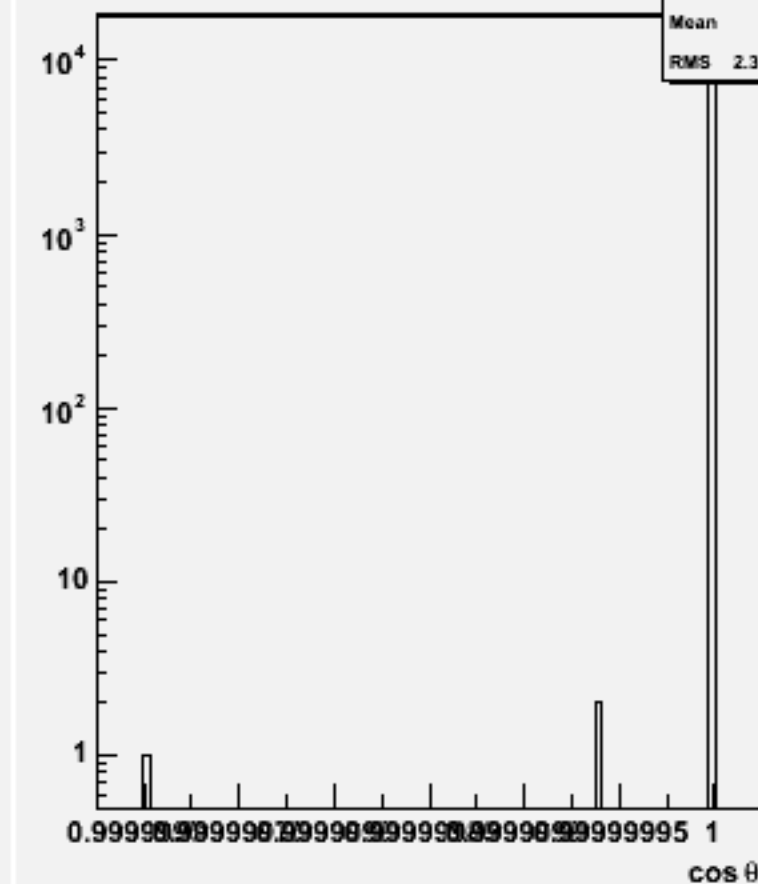
Jet cos \theta (All jets)w102783 aa_e3e3_o
