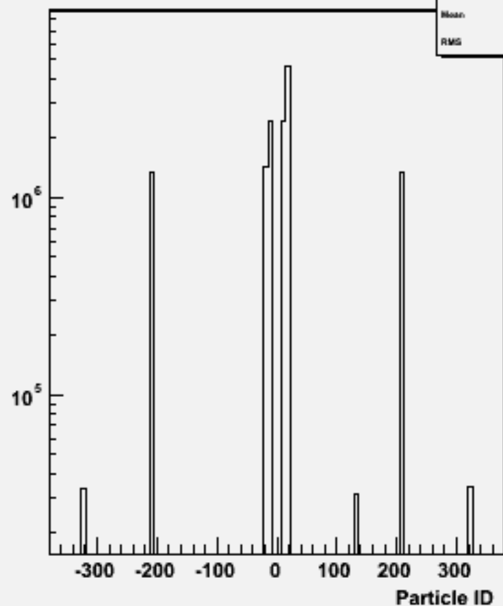
Particle ID : w102783 aa_e3e3_o
