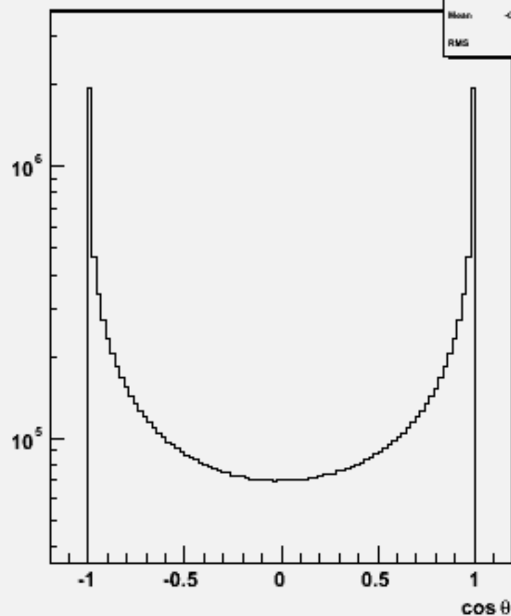
Particle cos \theta : w102783 aa_e3e3_o
