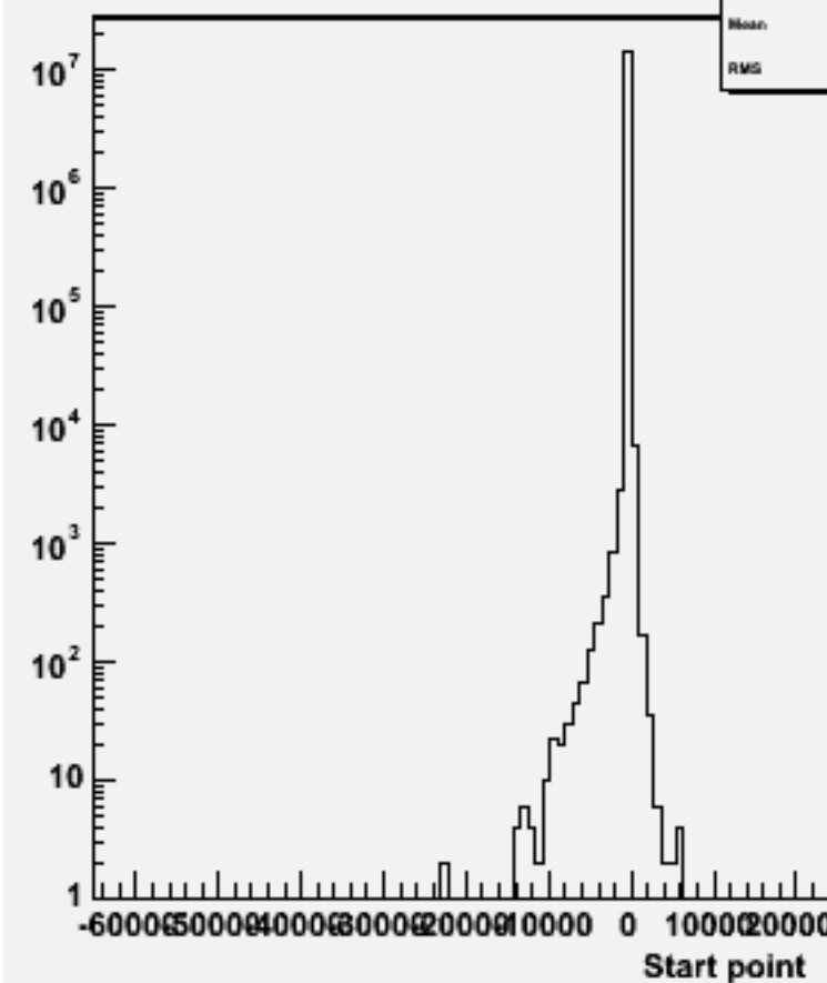
Start point Z : w102782 aa_e3e3_o
