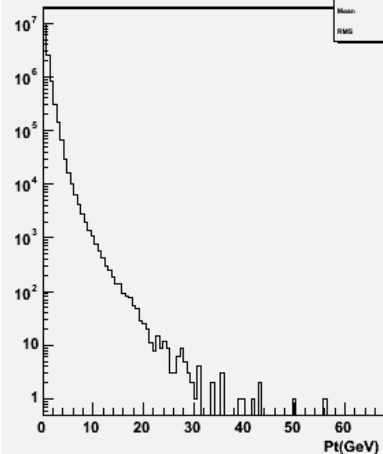
Particle Pt : w102782 aa_e3e3_o
