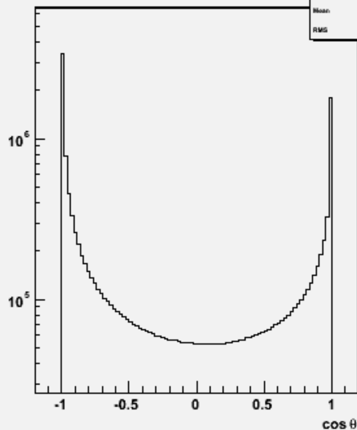
Particle cosθ : w102782 aa_e3e3_o
