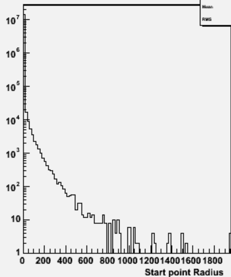
Start point R : w102782 aa_e3e3_o
