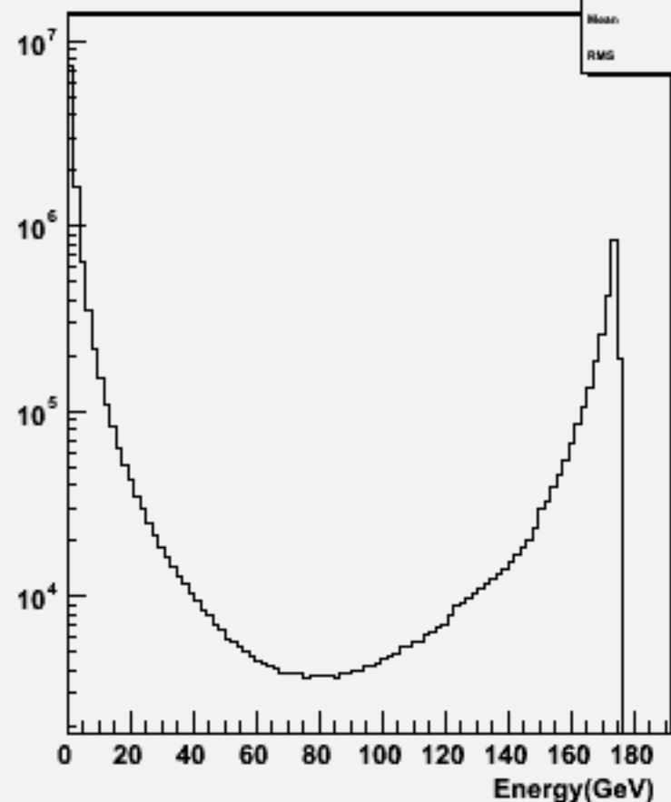
Particle Energy : w102782 aa_e3e3_o
