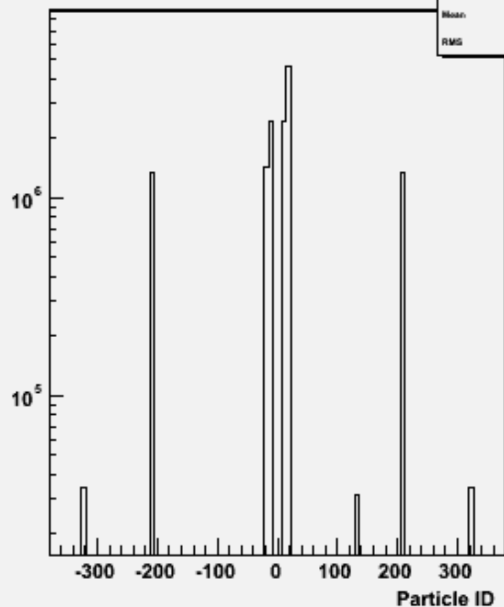
Particle ID : w102782 aa_e3e3_o
