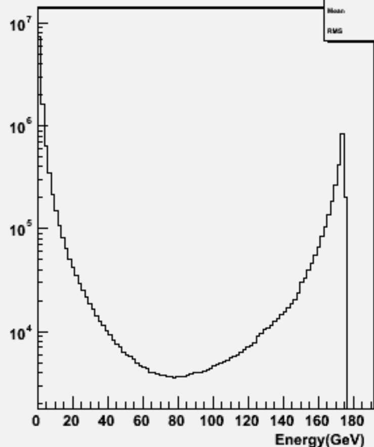
Particle Energy : w102781 aa_e3e3_o
