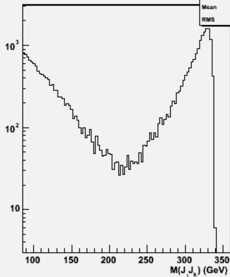
2jets mass(All comb)w102781 aa_e3e3_o
