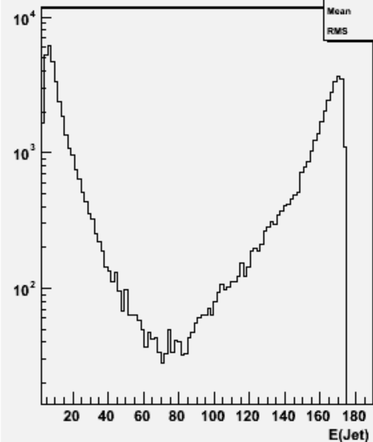
Jet energies(All jets)w102781 aa_e3e3_o
