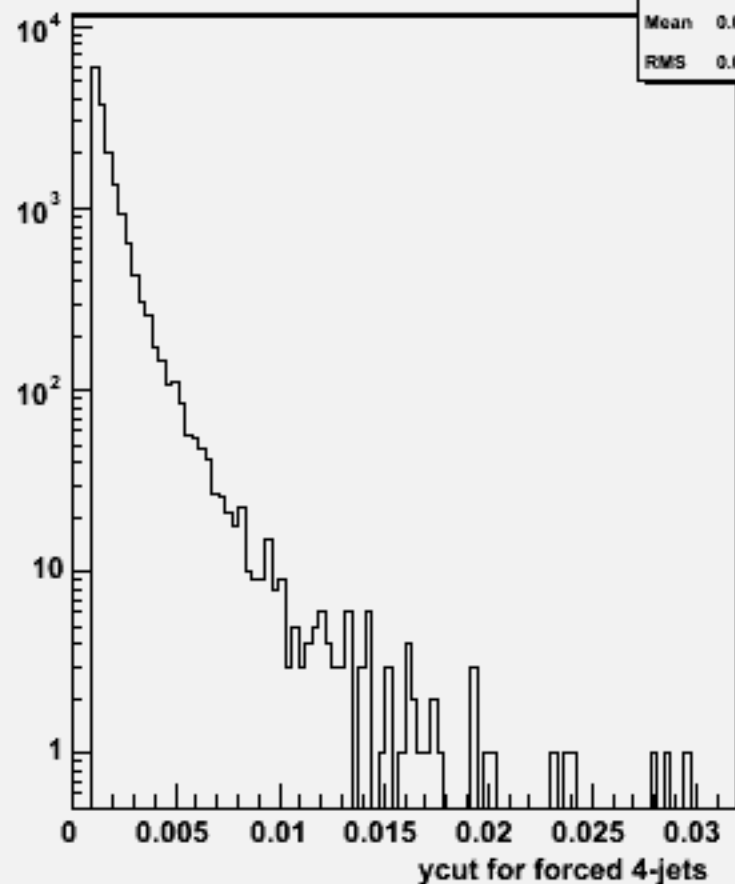
Ycut for 4-jets :w102781 aa_e3e3_o
