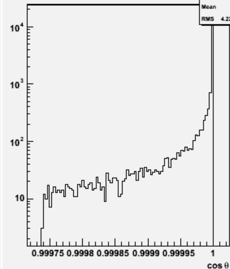
Jet cos \theta (All jets)w102781 aa_e3e3_o
