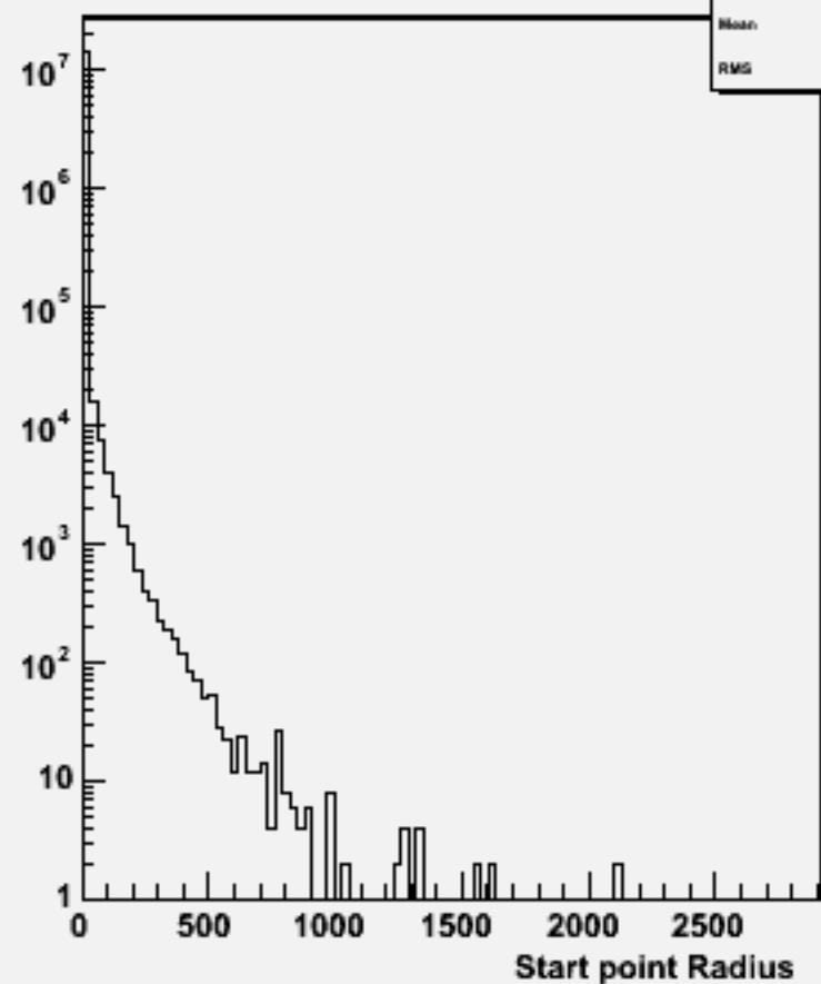
Start point R : w102781 aa_e3e3_o
