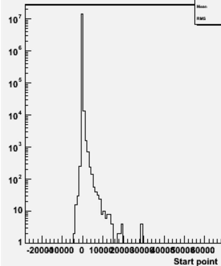
Start point Z : w102781 aa_e3e3_o
