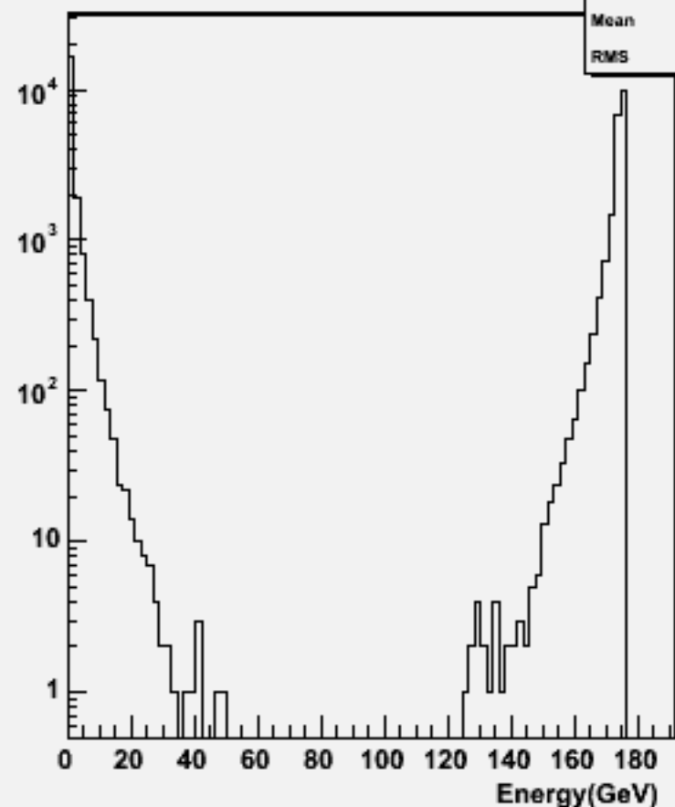
Particle Energy : w102779 aa_e2e2_o
