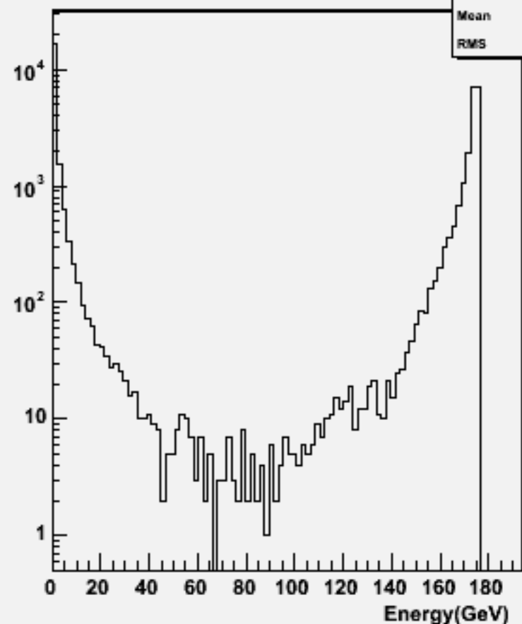
Particle Energy : w102776 aa_e2e2_o
