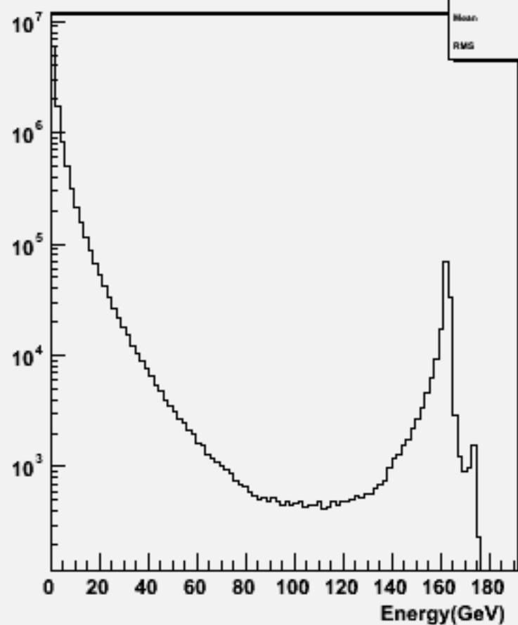
Particle Energy : w102770 bb_o
