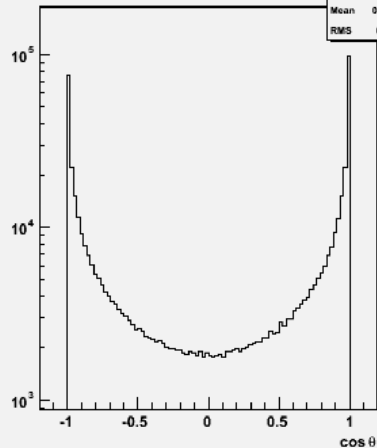
Jet cosθ (All jets)w102770 bb_o
