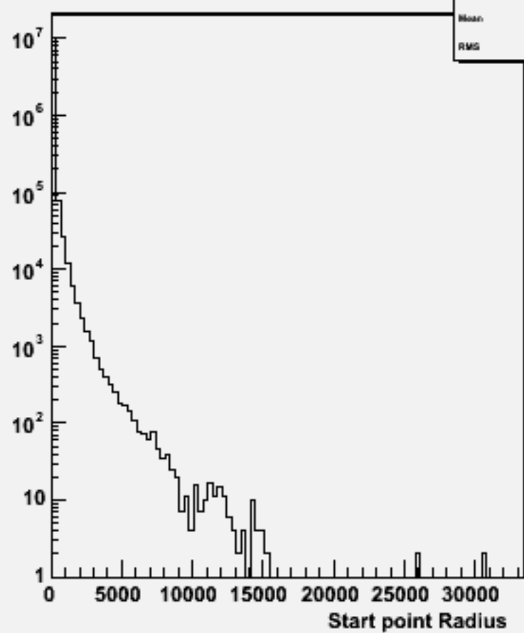
Start point R : w102770 bb_o
