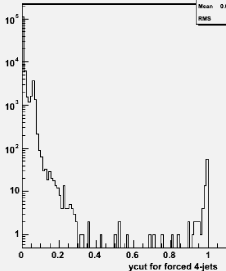
Ycut for 4-jets :w102770 bb_o
