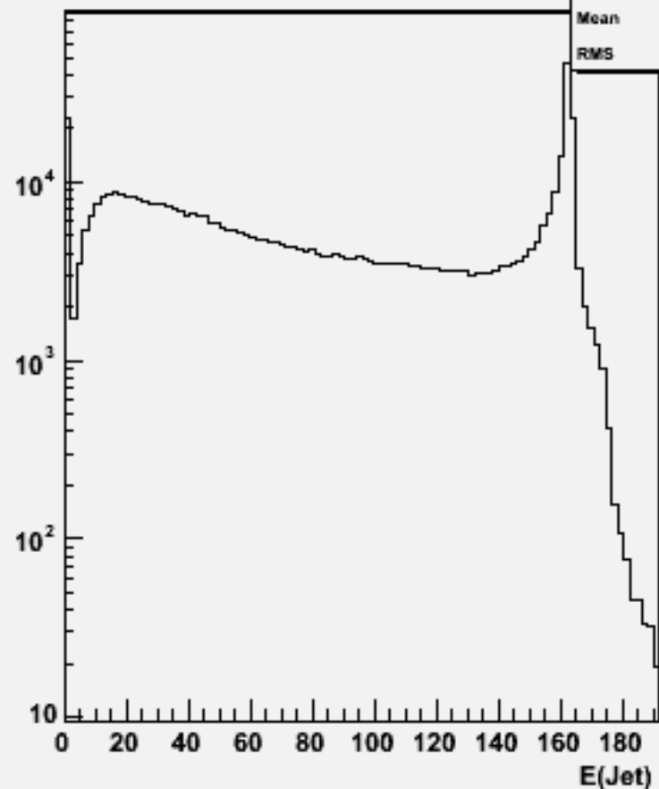
Jet energies(All jets)w102770 bb_o
