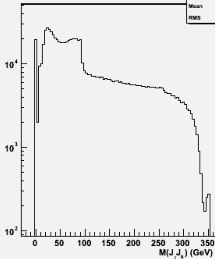
2jets mass(All comb)w102770 bb_o
