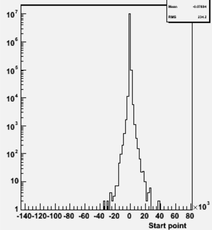
Start point Z : w102770 bb_o
