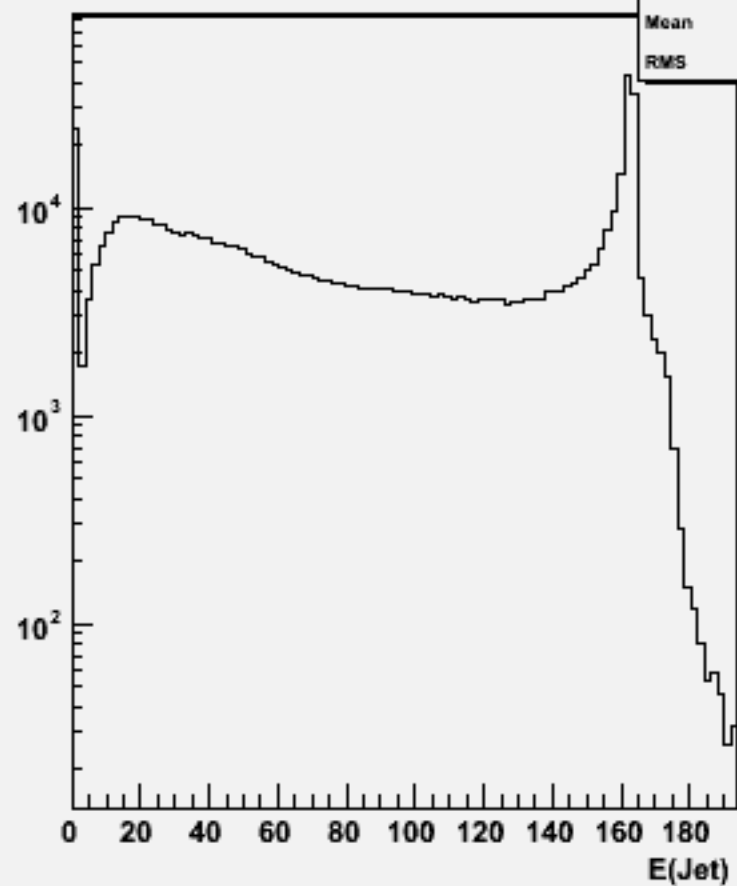
Jet energies(All jets)w102766 ss_o
