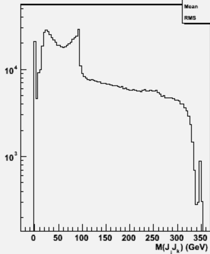
2jets mass(All comb)w102766 ss_o
