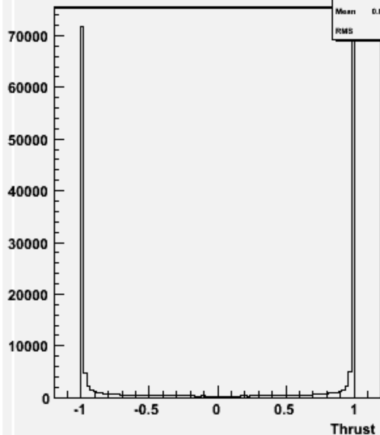
cos \Theta (thrust) w102766 ss_o
