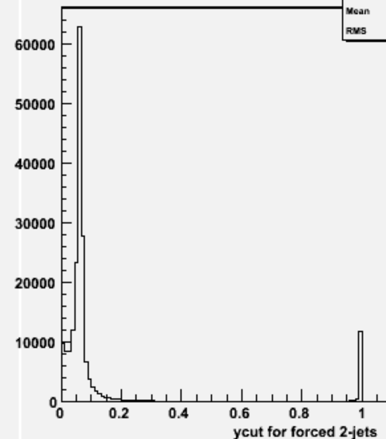
Ycut for 2-jets :w102766 ss_o
