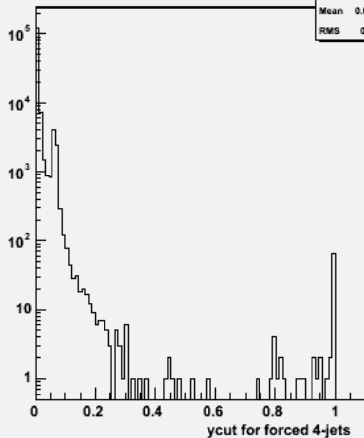
Ycut for 4-jets :w102766 ss_o
