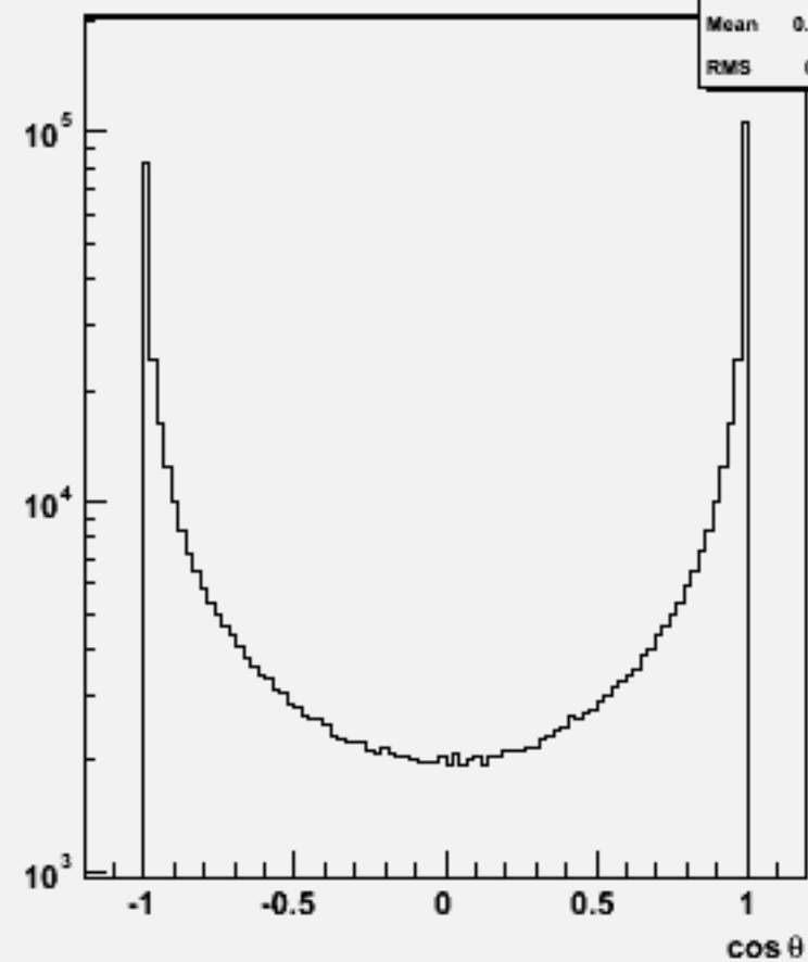
Jet cos \theta (All jets)w102766 ss_o
