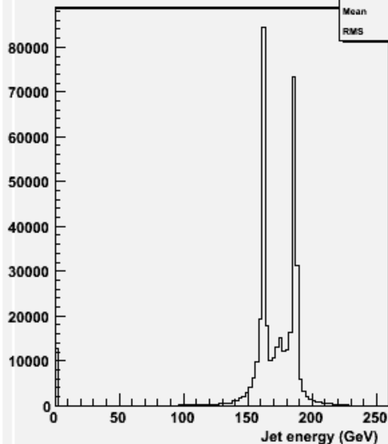
energy for 2-jets :w102766 ss_o
