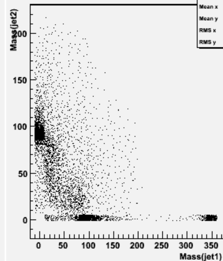
Jet mass for forced 2-jets : w102766 ss_o
