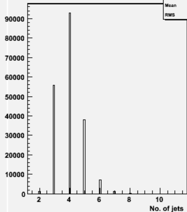
No. jets (ycut=0.001) : w102766 ss_o
