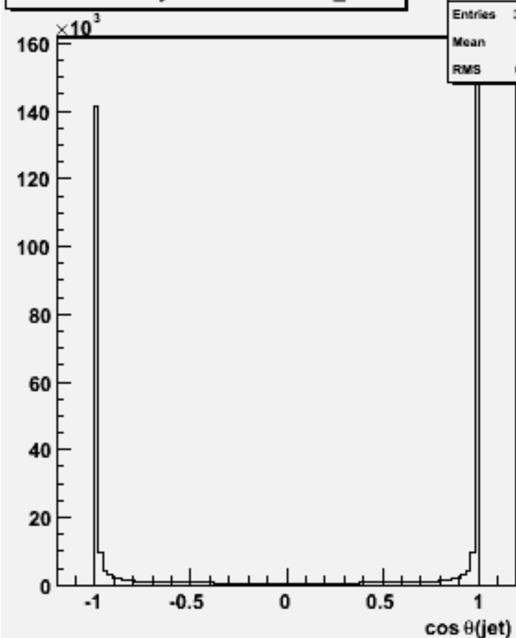
cos \Theta for 2-jets :w102766 ss_o
