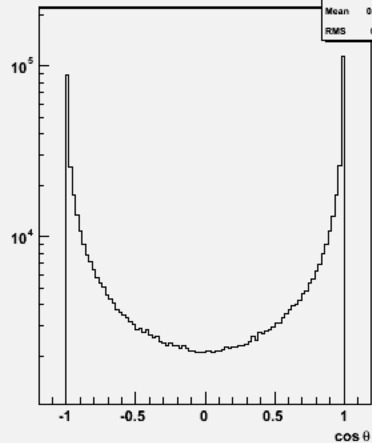
Jet cos \theta (All jets)w102762 dd_o
