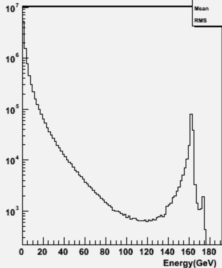
Particle Energy : w102762 dd_o
