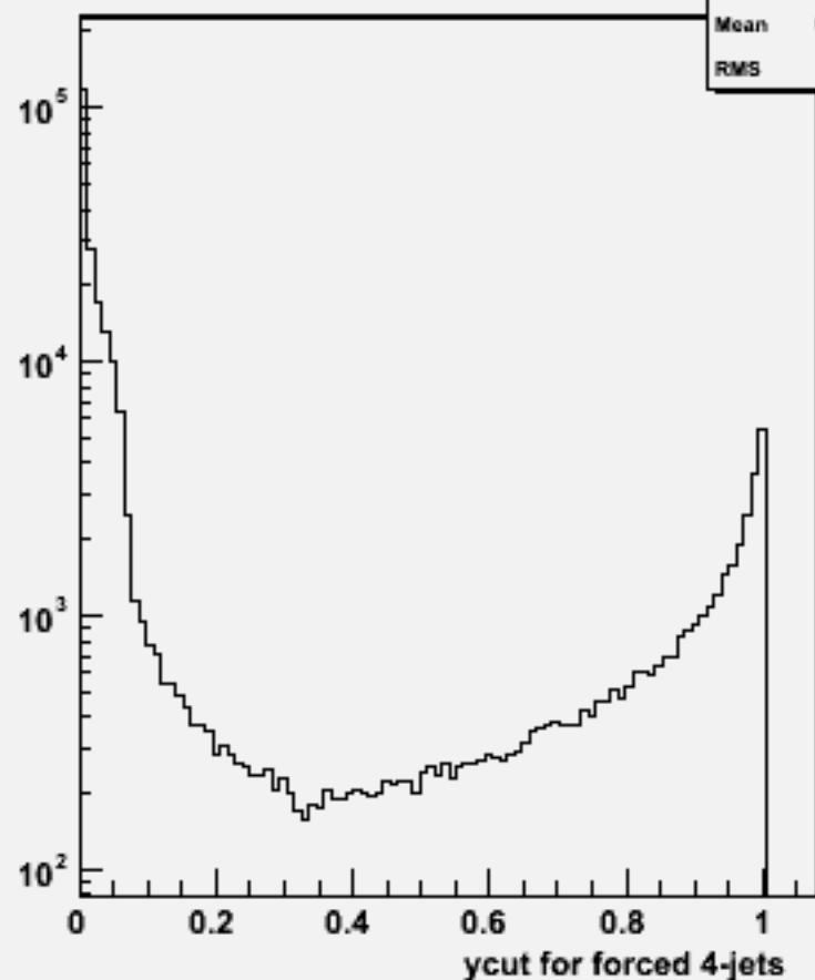
Ycut for 4-jets :w102757 e3e3_o
