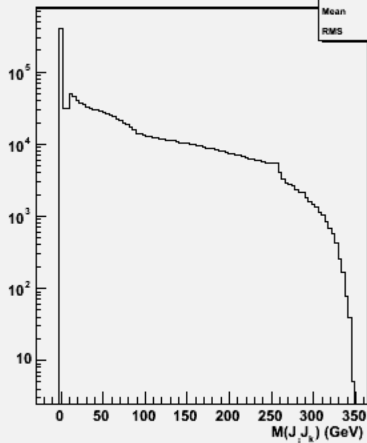
2jets mass(All comb)w102757 e3e3_o
