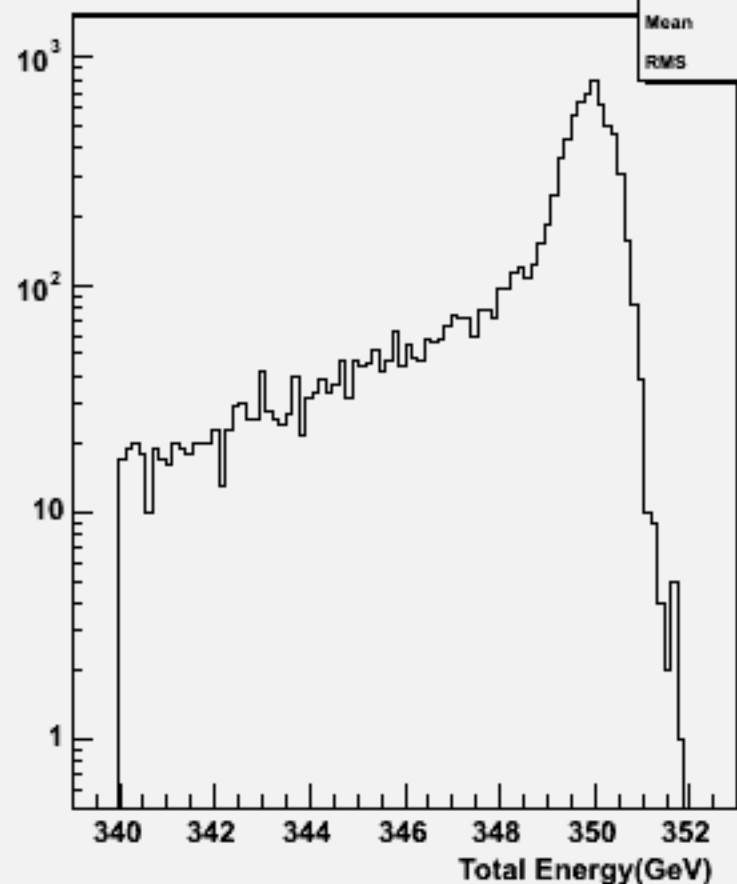
Total Energy (inc. \nu ): w102749 e1e1_o
