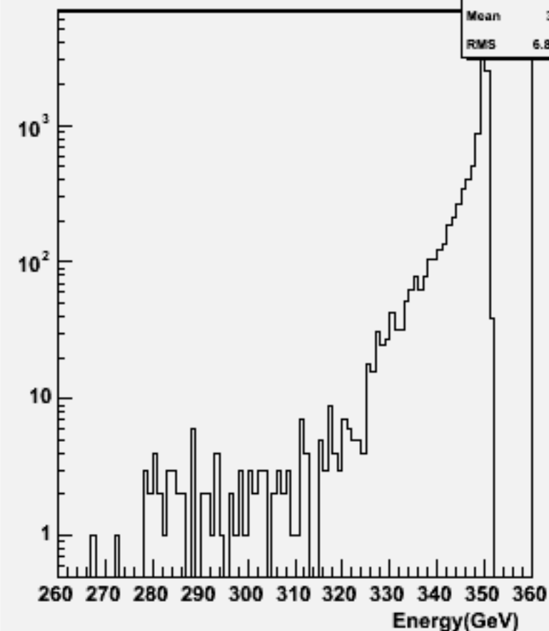
Total Energy (w/o \nu ): w102749 e1e1_o
