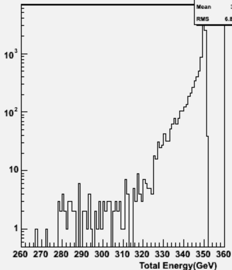
Total Energy (inc. \nu ): w102749 e1e1_o
