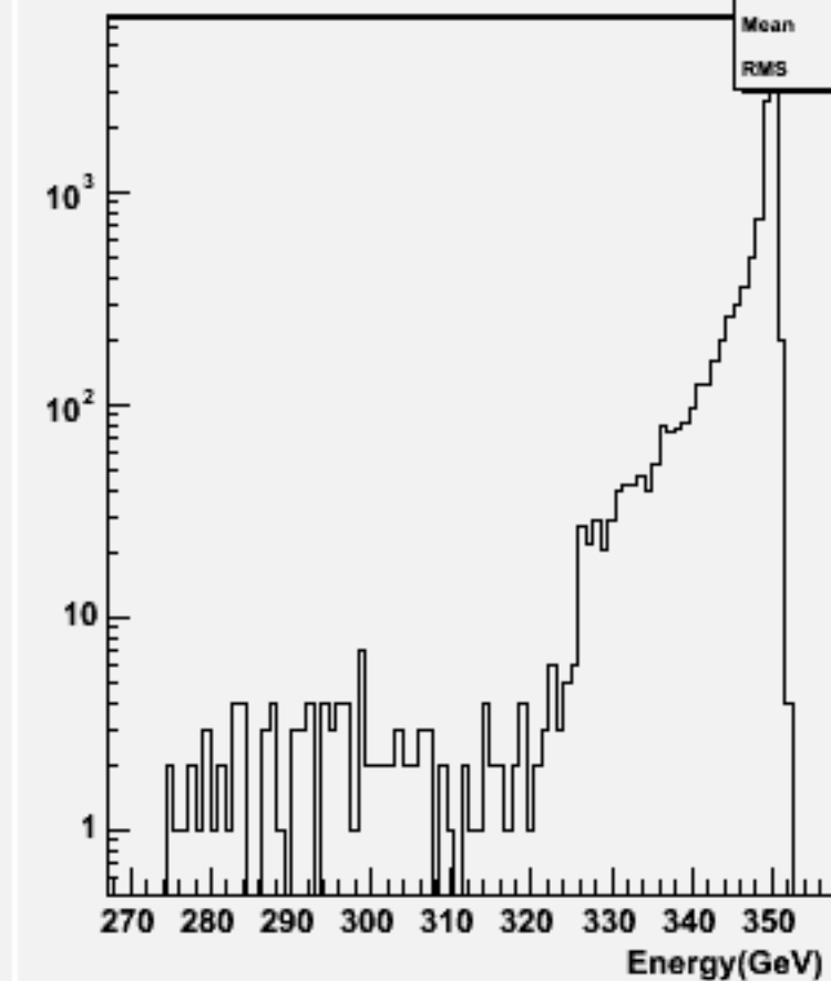
Total Energy (w/o \nu ): w102748 e1e1_o
