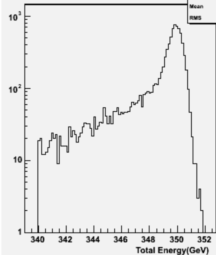
Total Energy (inc. \nu ): w102748 e1e1_o
