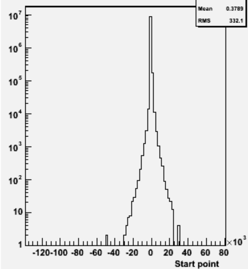
Start point Z : w102746 cc_o
