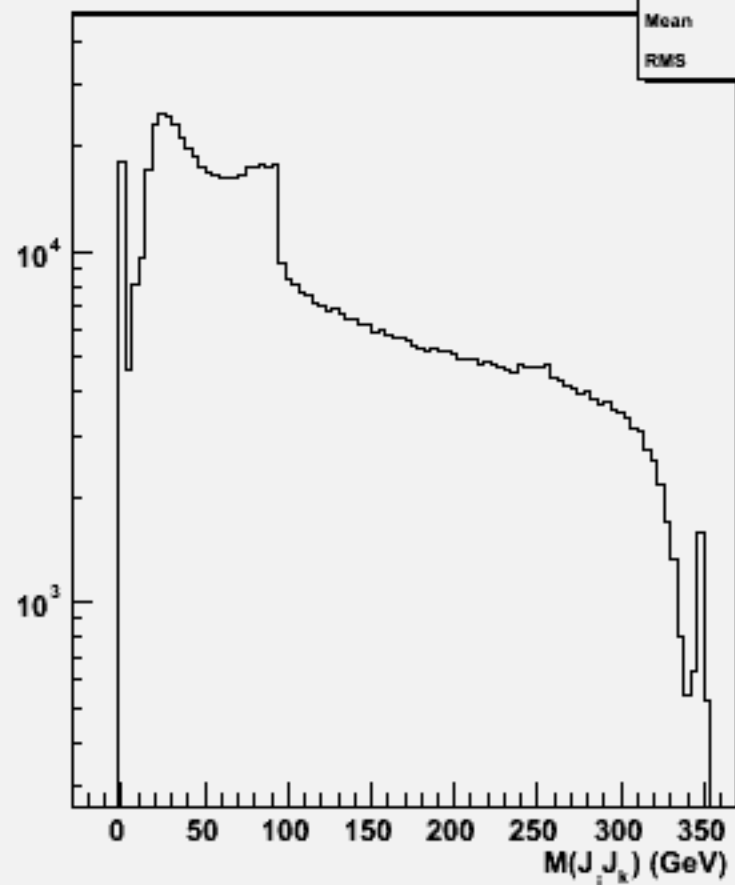
2jets mass(All comb)w102746 cc_o
