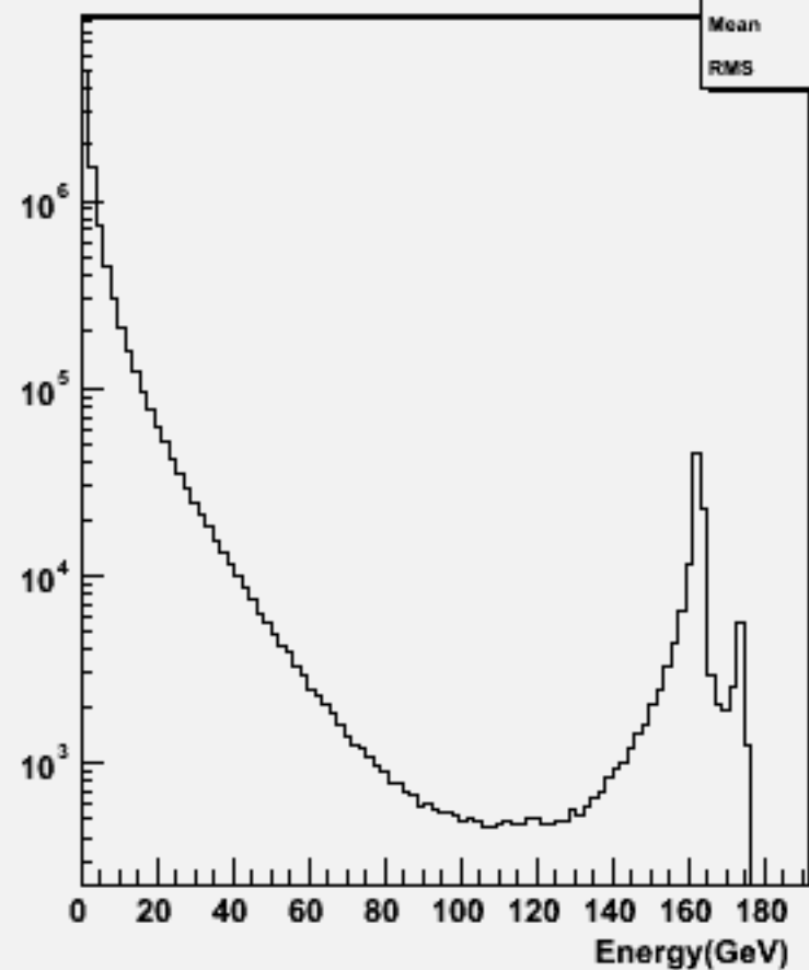
Particle Energy : w102746 cc_o
