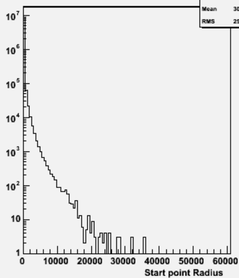
Start point R : w102746 cc_o
