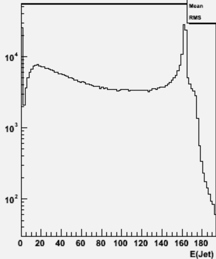
Jet energies(All jets)w102746 cc_o
