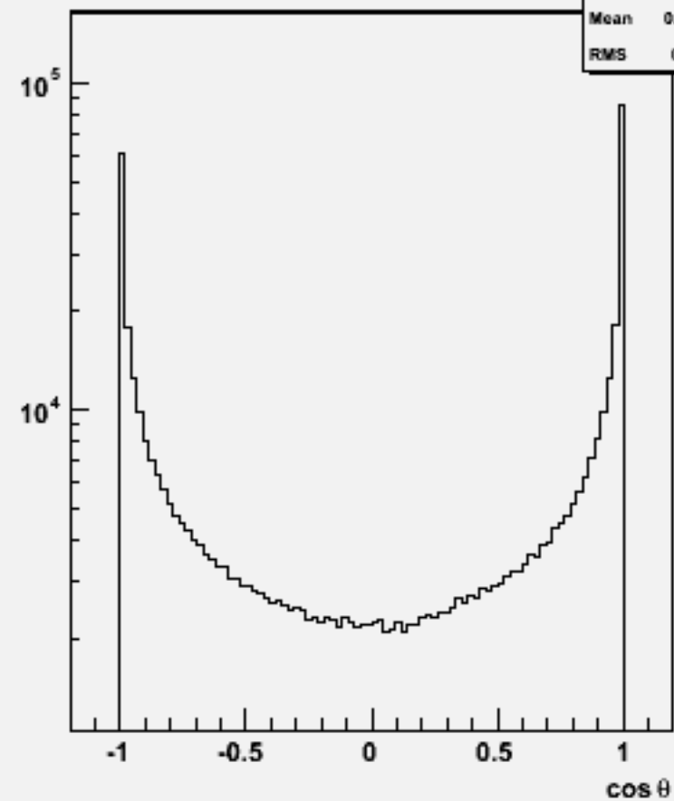
Jet cos \theta (All jets)w102746 cc_o
