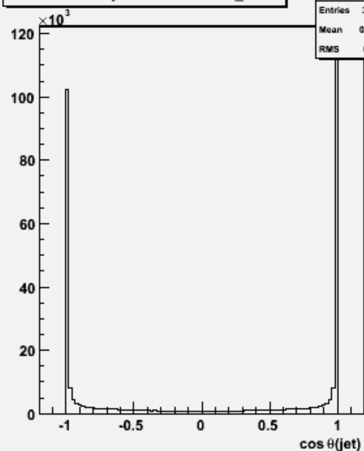
cos \Theta for 2-jets :w102746 cc_o
