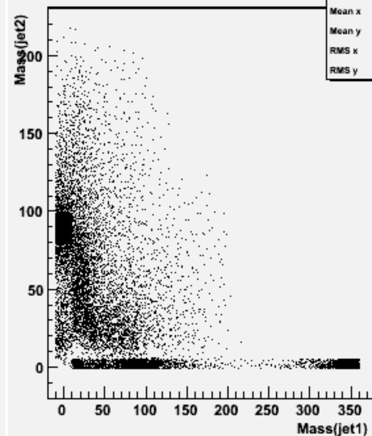
Jet mass for forced 2-jets : w102746 cc_o
