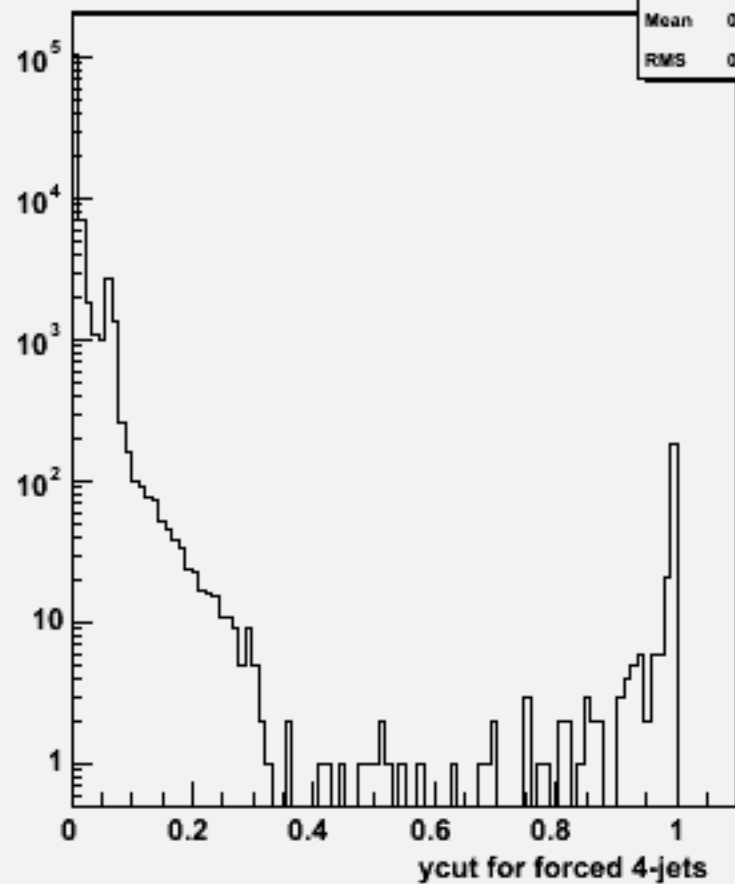
Ycut for 4-jets :w102746 cc_o
