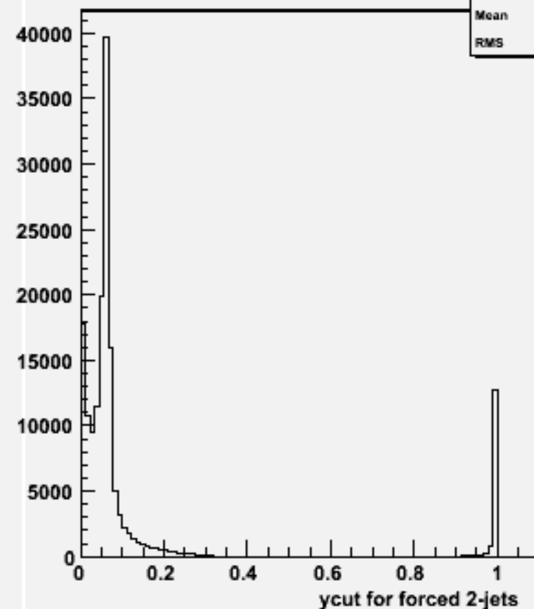
Ycut for 2-jets :w102746 cc_o
