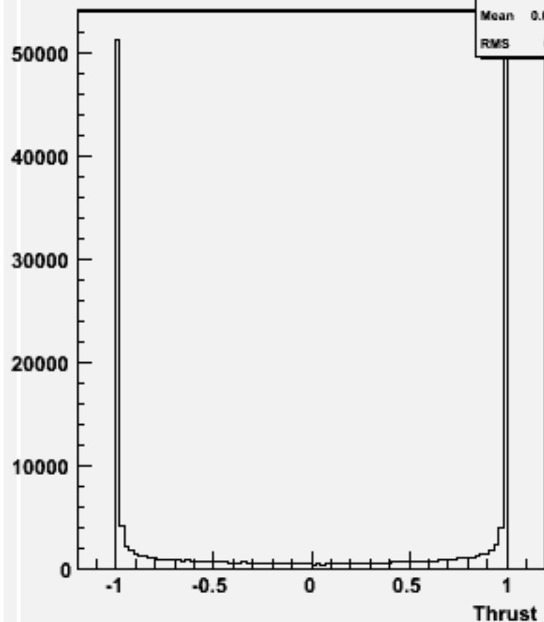
cos \Theta (thrust) w102746 cc_o
