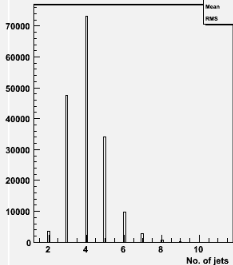
No. jets (ycut=0.001) : w102746 cc_o
