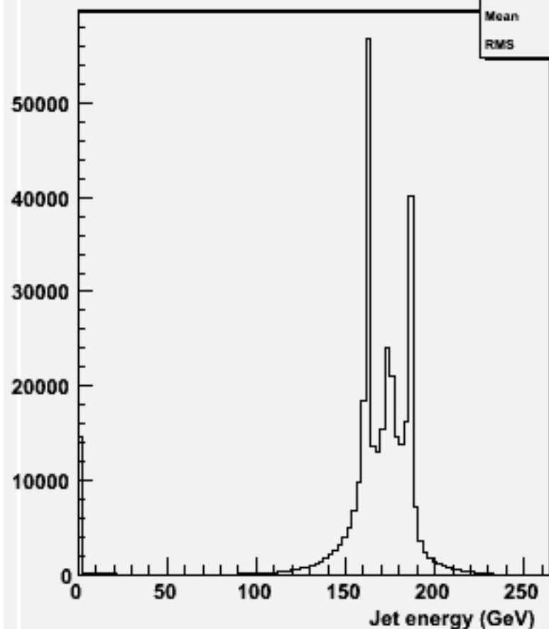
energy for 2-jets :w102746 cc_o
