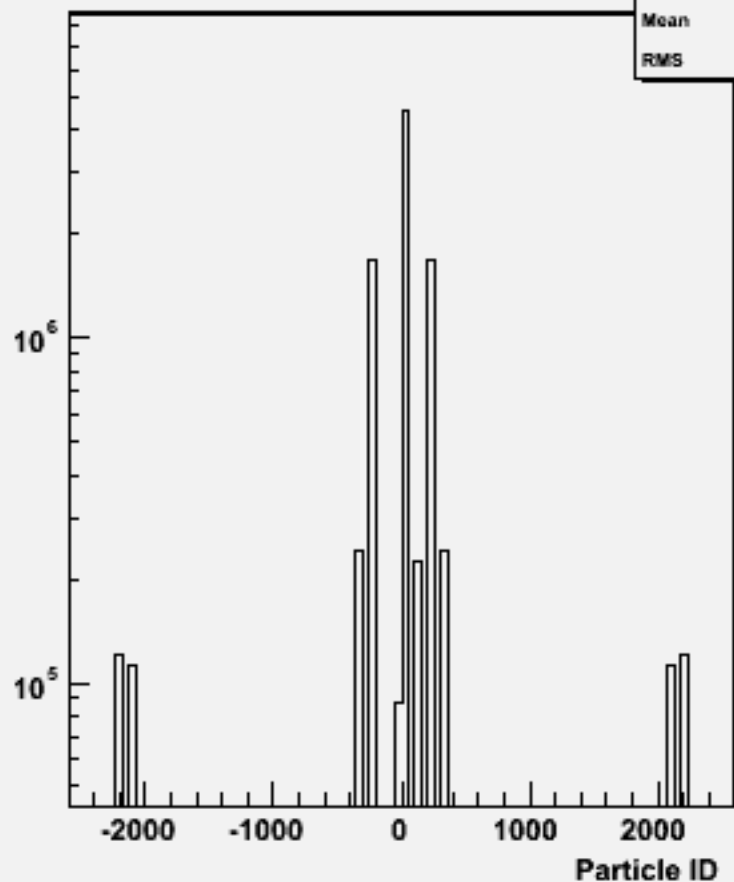
Particle ID : w102745 cc_o
