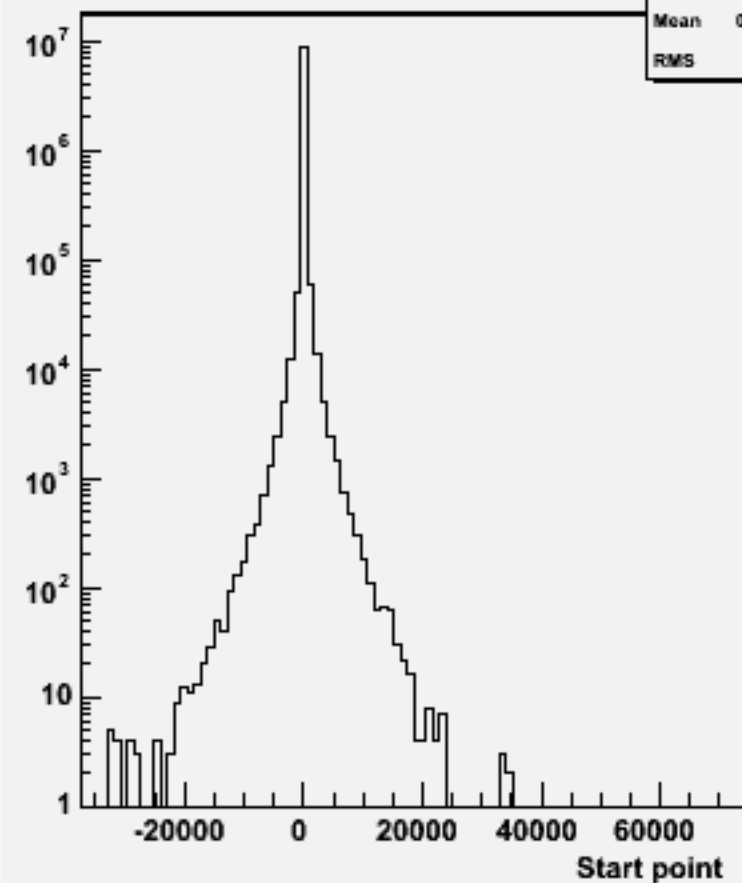
Start point Z : w102745 cc_o
