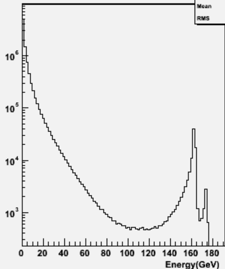
Particle Energy : w102745 cc_o
