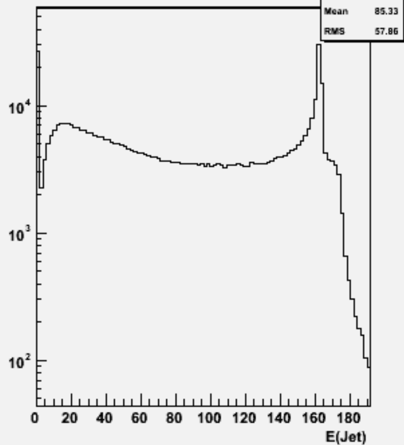
Jet energies(All jets)w102745 cc_o
