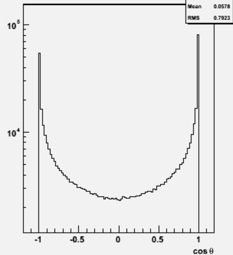
Jet cosθ (All jets)w102745 cc_o
