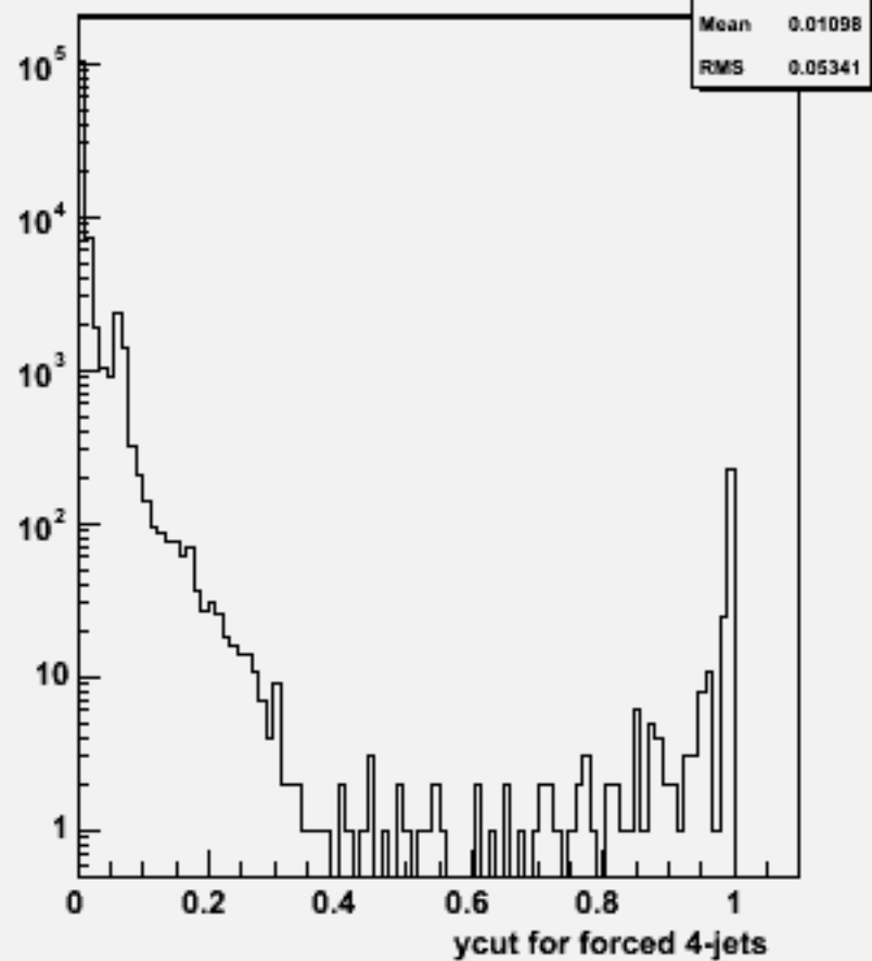
Ycut for 4-jets :w102745 cc_o
