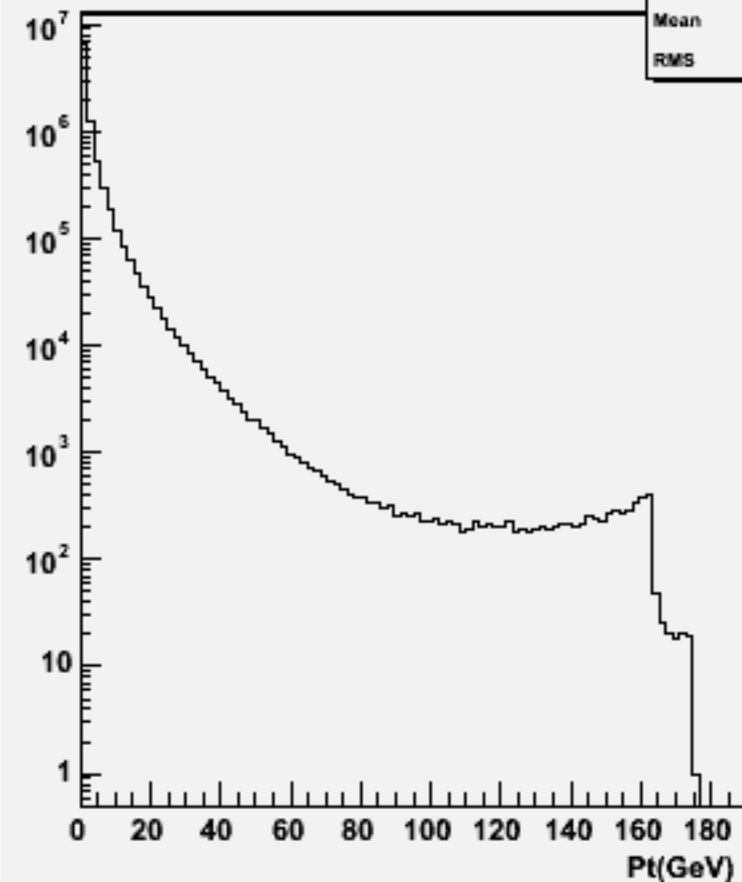
Particle Pt : w102745 cc_o
