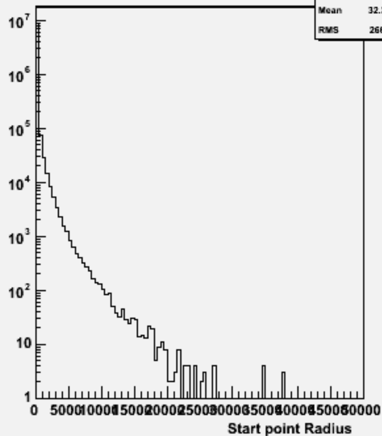
Start point R : w102745 cc_o
