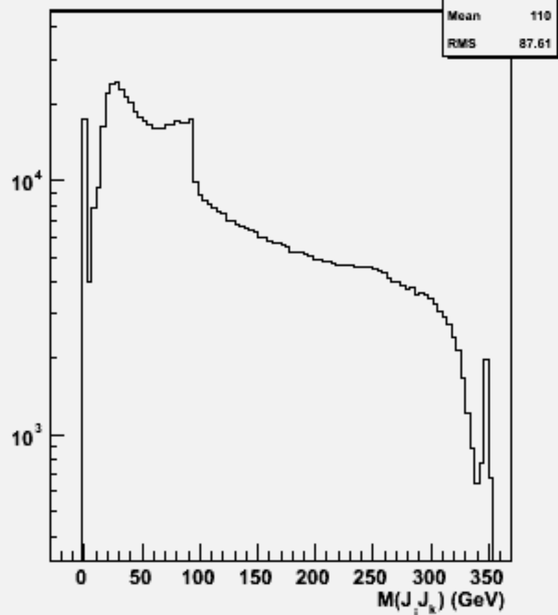
2jets mass(All comb)w102745 cc_o
