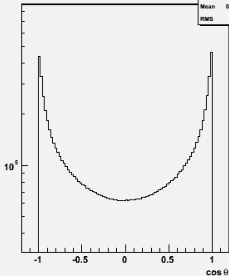
Particle cosθ : w102745 cc_o
