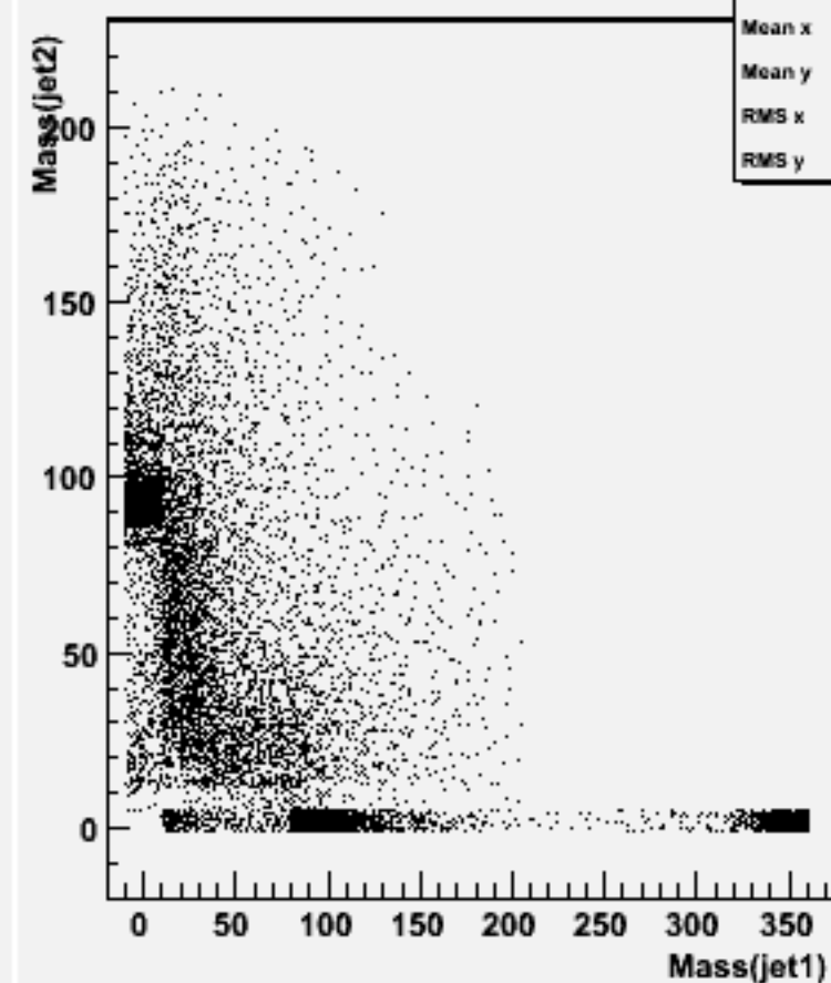
Jet mass for forced 2-jets : w102741 uu_o
