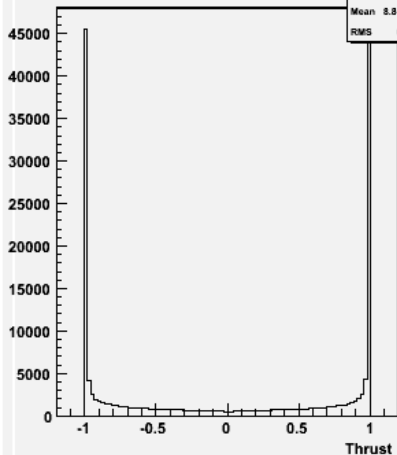
cos \Theta (thrust) w102741 uu_o
