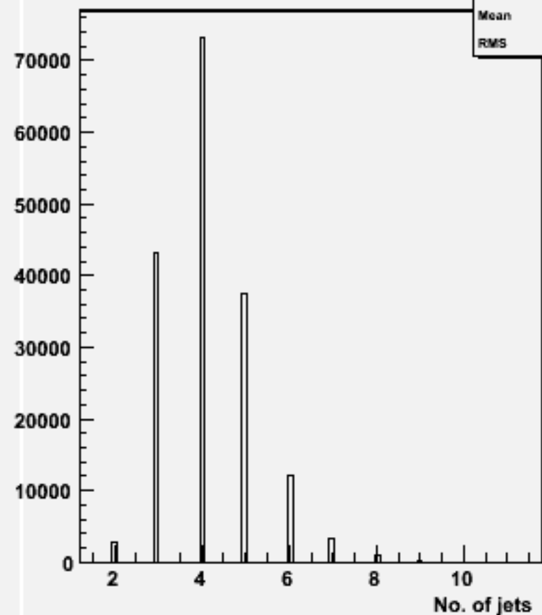
No. jets (ycut=0.001) : w102741 uu_o
