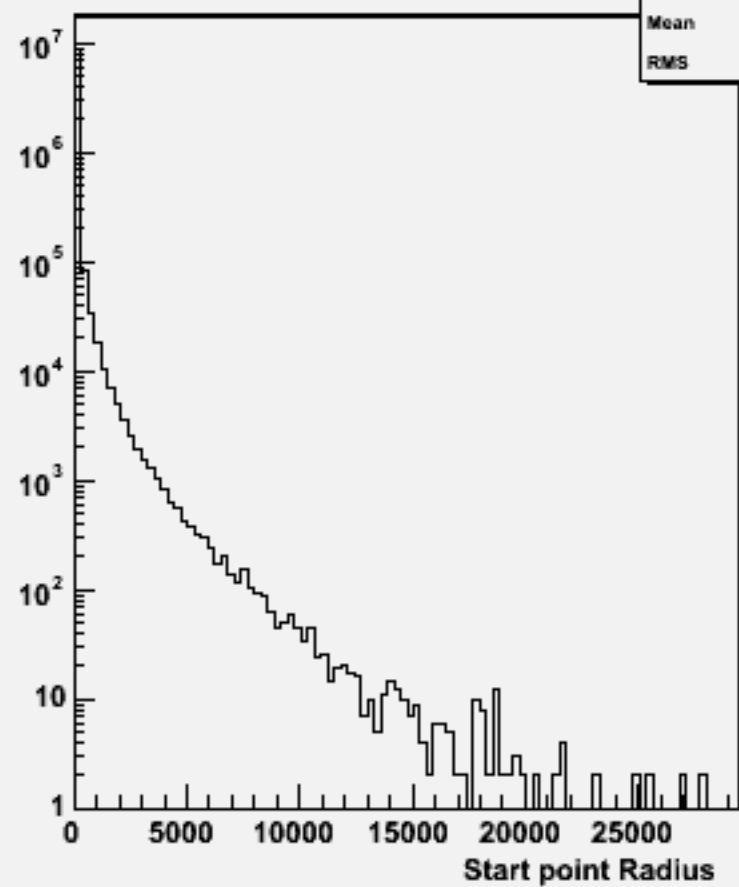
Start point R : w102741 uu_o
