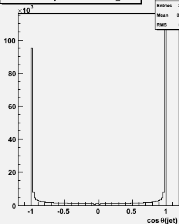
cos \Theta for 2-jets :w102741 uu_o
