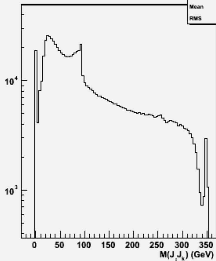
2jets mass(All comb)w102741 uu_o
