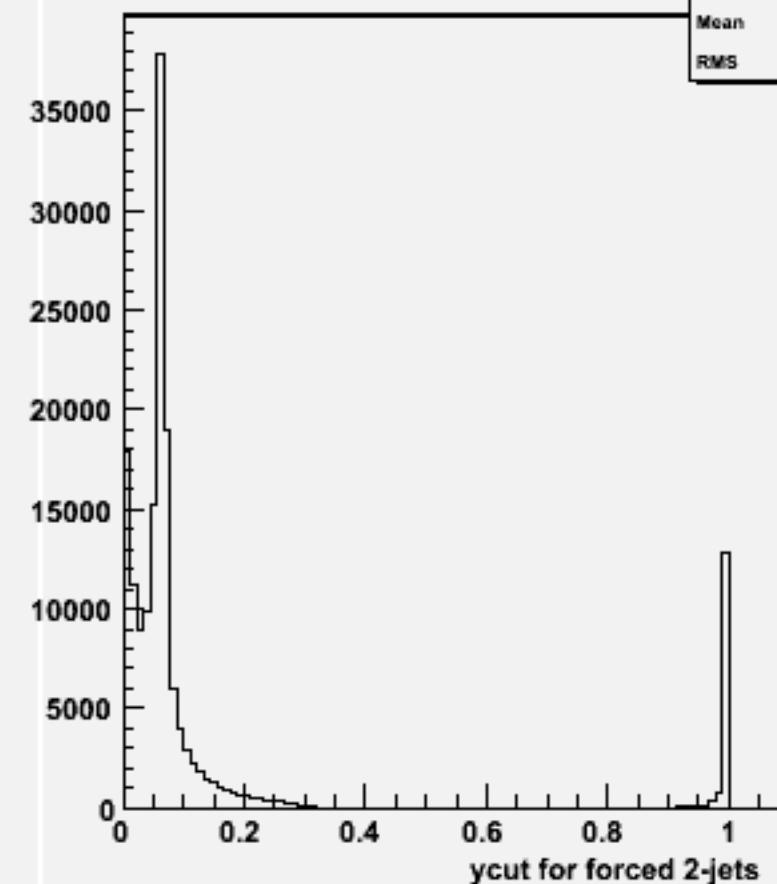
Ycut for 2-jets :w102741 uu_o
