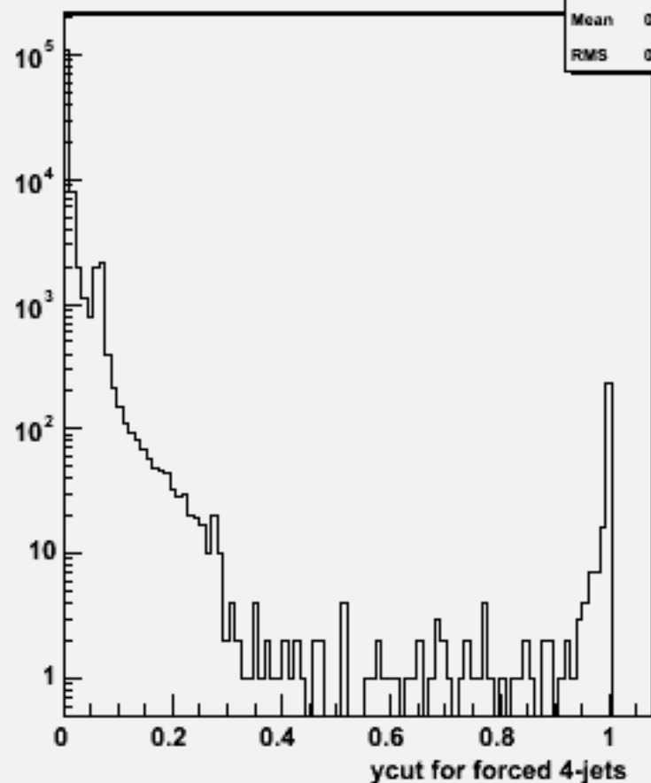
Ycut for 4-jets :w102741 uu_o
