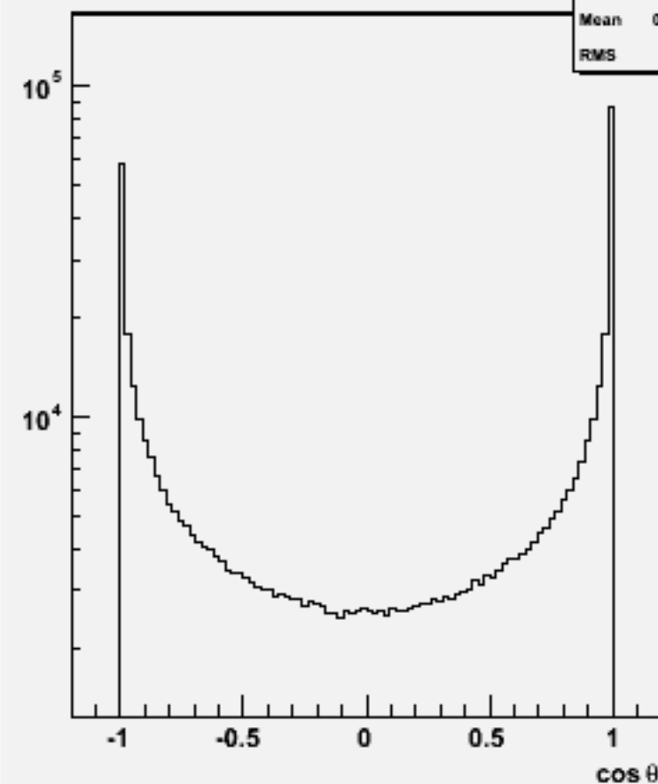
Jet cos \theta (All jets)w102741 uu_o
