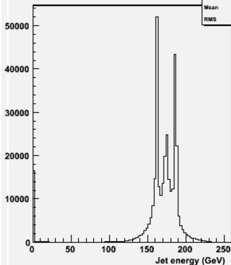
energy for 2-jets :w102741 uu_o
