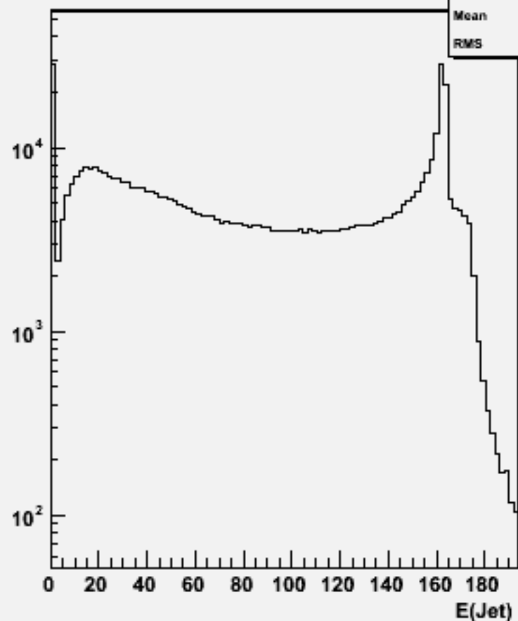
Jet energies(All jets)w102741 uu_o
