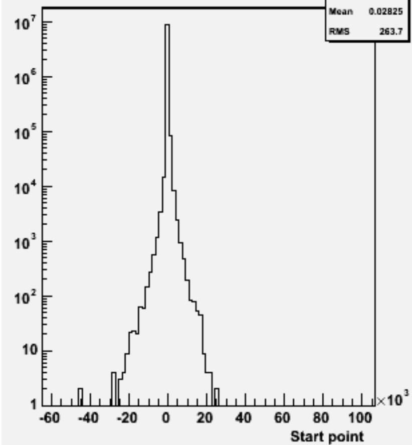
Start point Z : w102741 uu_o
