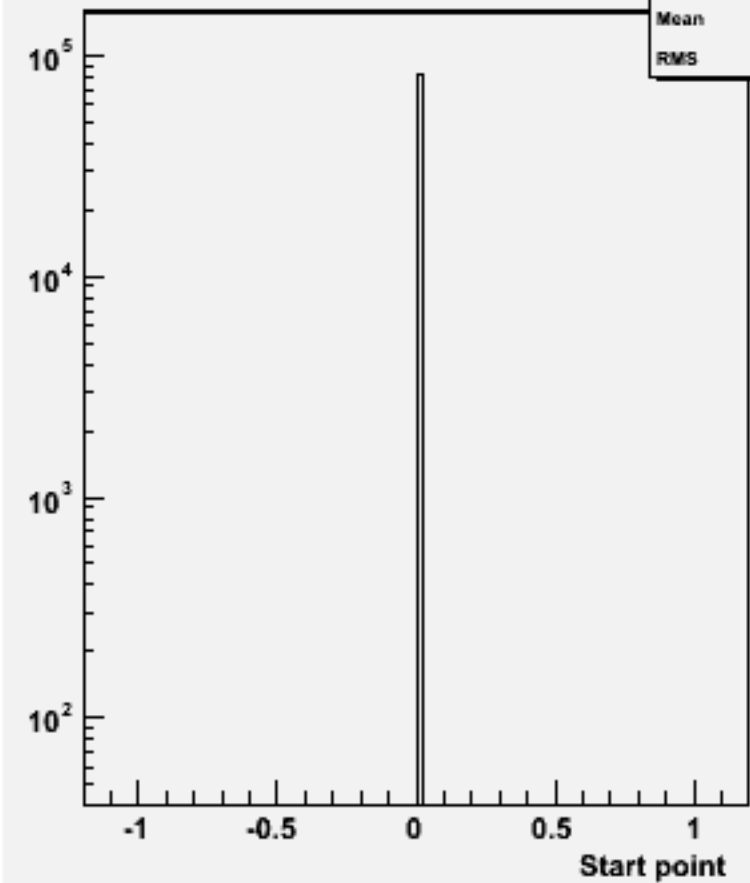
Start point Z : w102738 n3n3aaa_o
