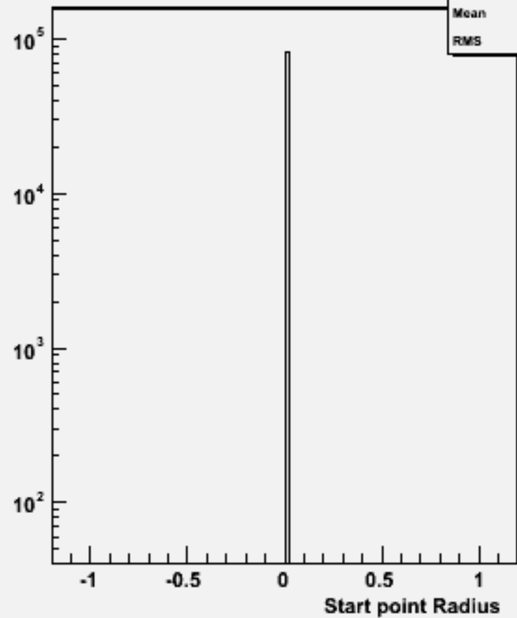
Start point R : w102738 n3n3aaa_o
