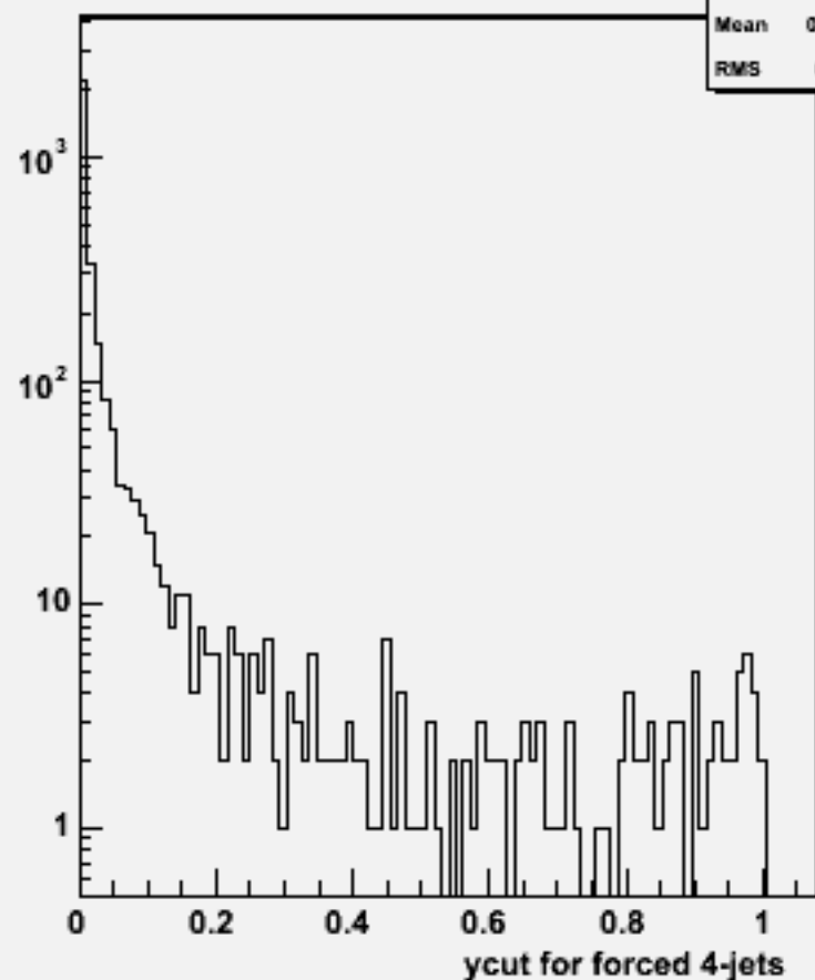
Ycut for 4-jets :w102738 n3n3aaa_o
