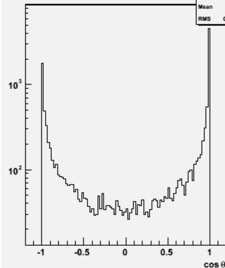
Jet cos \theta (All jets)w102738 n3n3aaa_o
