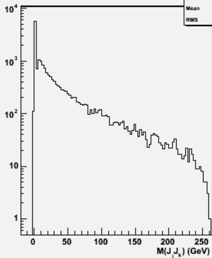
2jets mass(All comb)w102738 n3n3aaa_o
