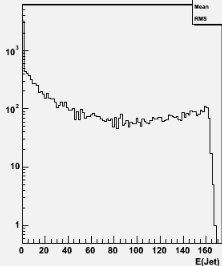
Jet energies(All jets)w102738 n3n3aaa_o
