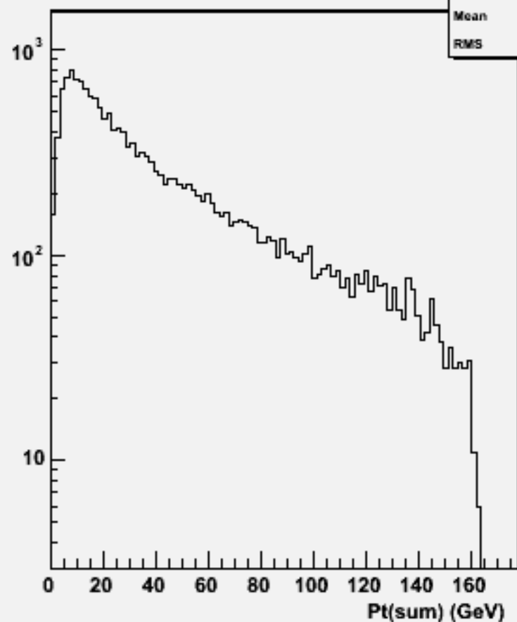
Pt Sum: w102733 n2n2aaa_o
