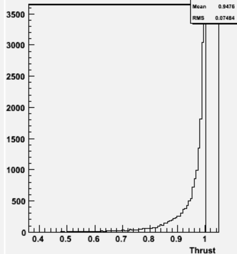
Thrust w102733 n2n2aaa_o
