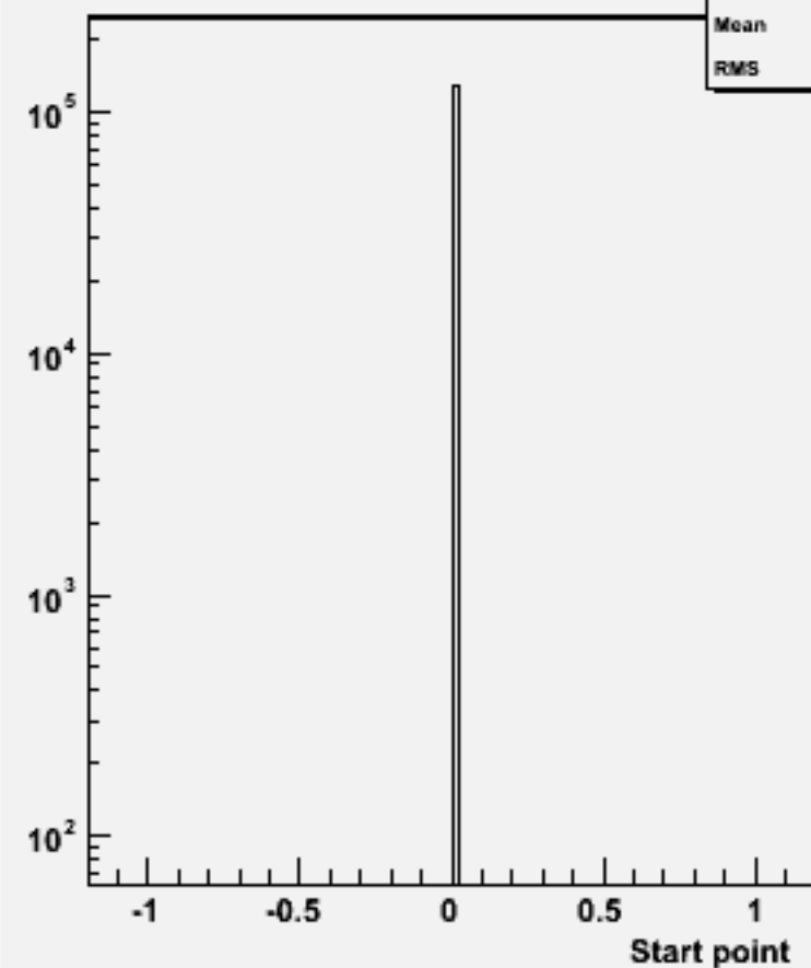
Start point Z : w102733 n2n2aaa_o
