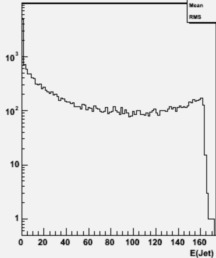
Jet energies(All jets)w102733 n2n2aaa_o
