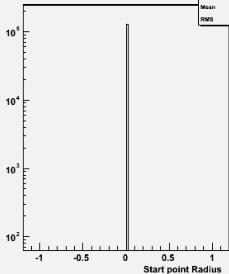
Start point R : w102733 n2n2aaa_o
