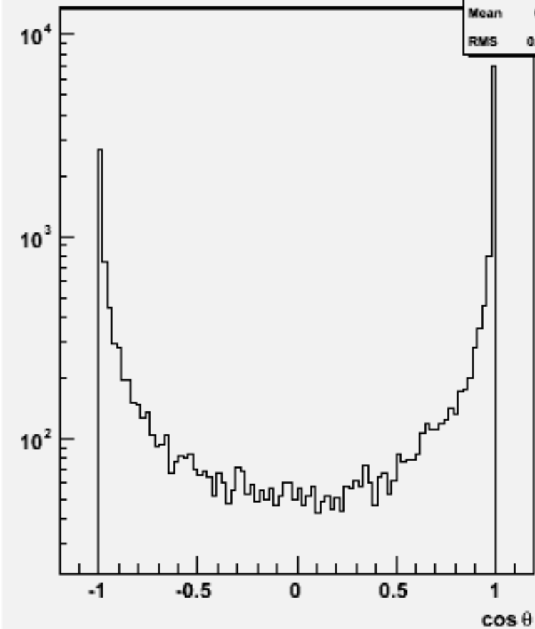
Jet cos \theta (All jets)w102733 n2n2aaa_o
