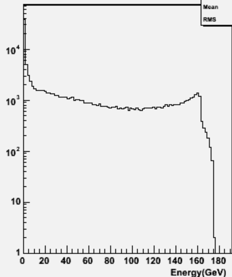
Particle Energy : w102733 n2n2aaa_o
