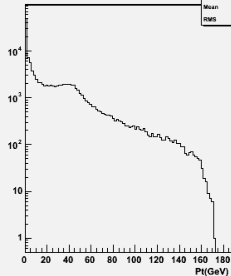
Particle Pt : w102733 n2n2aaa_o
