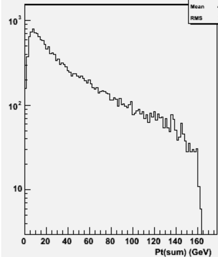
Pt Sum: w102733 n2n2aaa_o
