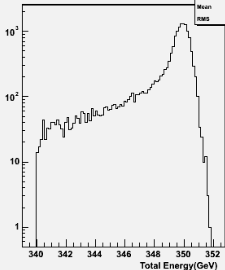
Total Energy (inc. \nu ): w102733 n2n2aaa_o
