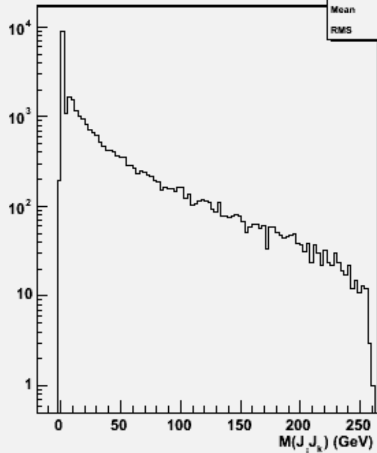
2jets mass(All comb)w102733 n2n2aaa_o
