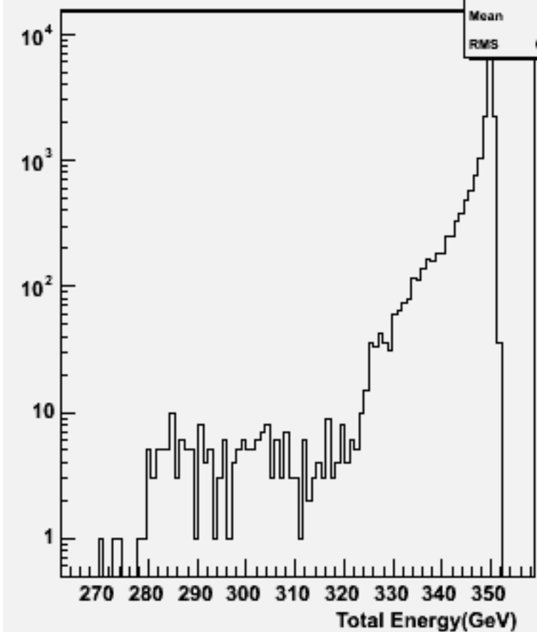
Total Energy (inc. \nu ): w102733 n2n2aaa_o
