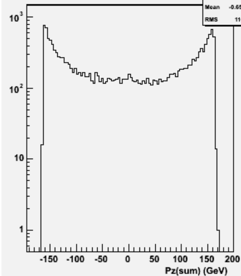
Pz Sum: w102733 n2n2aaa_o
