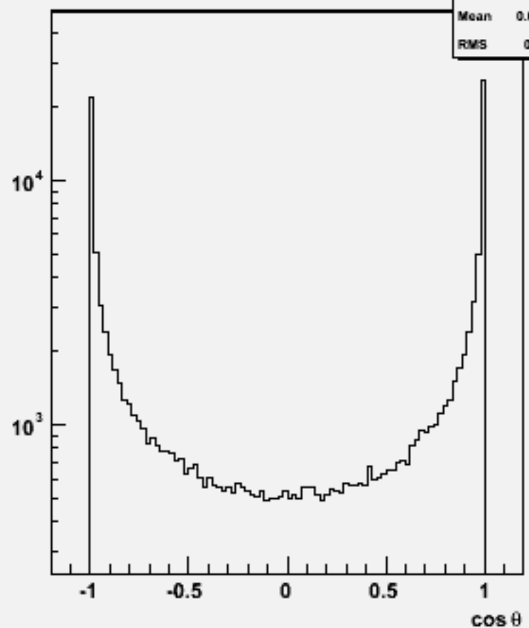
Particle \cos\theta : w102733 n2n2aaa_o
