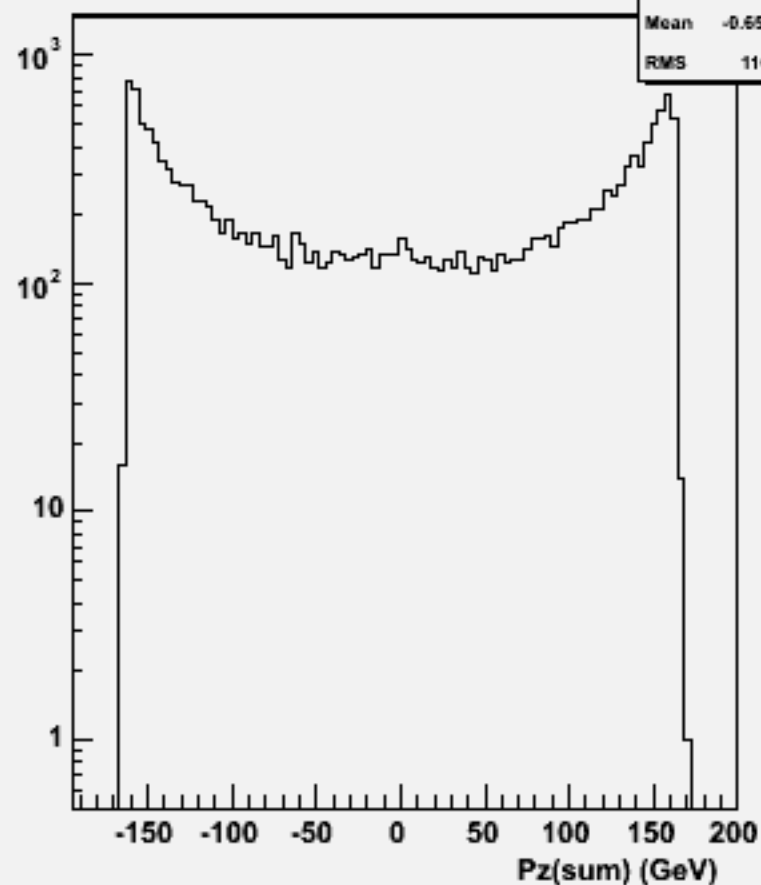
Pz Sum: w102733 n2n2aaa_o
