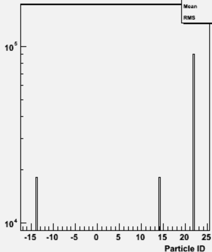
Particle ID : w102733 n2n2aaa_o
