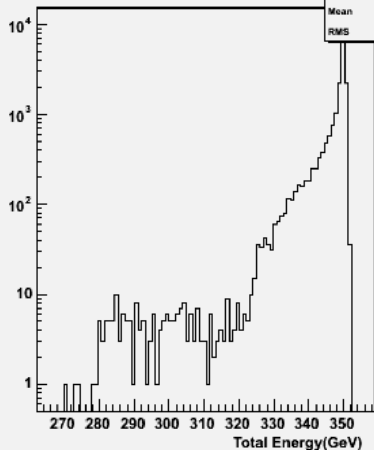
Total Energy (inc. \nu ): w102733 n2n2aaa_o
