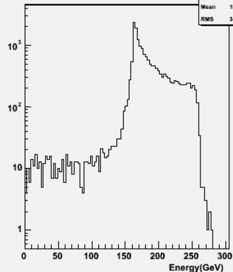
Total Energy (w/o \nu ): w102733 n2n2aaa_o
