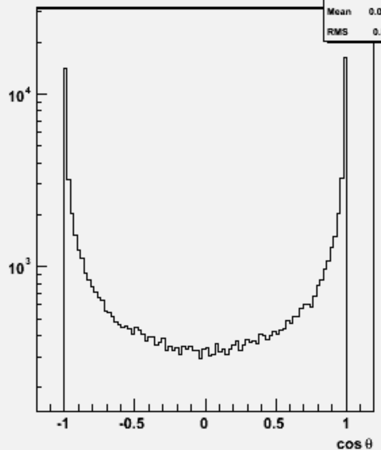
Particle \cos\theta : w102730 n1n1aaa_o
