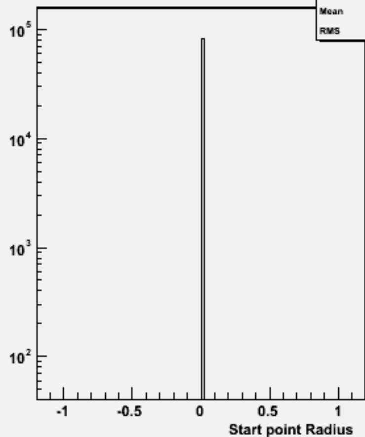
Start point R : w102730 n1n1aaa_o
