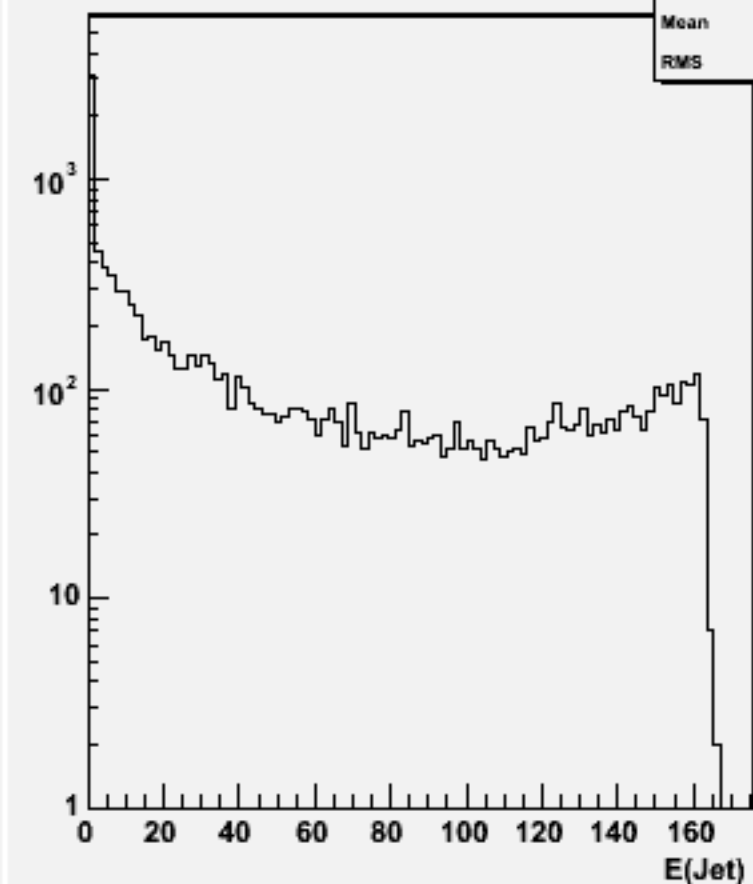
Jet energies(All jets)w102730 n1n1aaa_o
