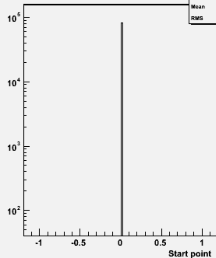
Start point Z : w102730 n1n1aaa_o
