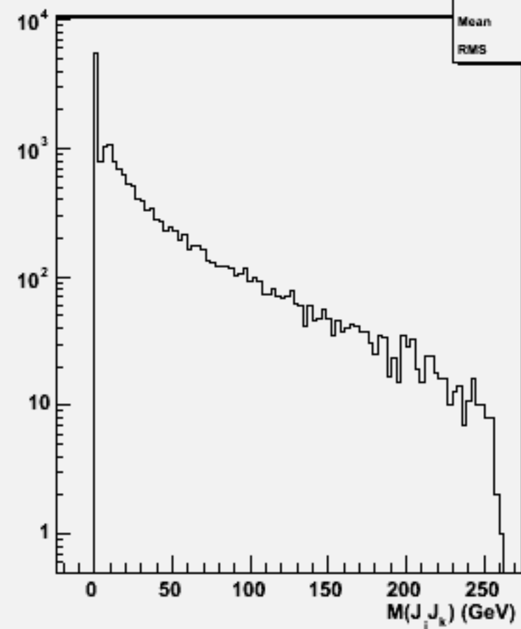
2jets mass(All comb)w102730 n1n1aaa_o
