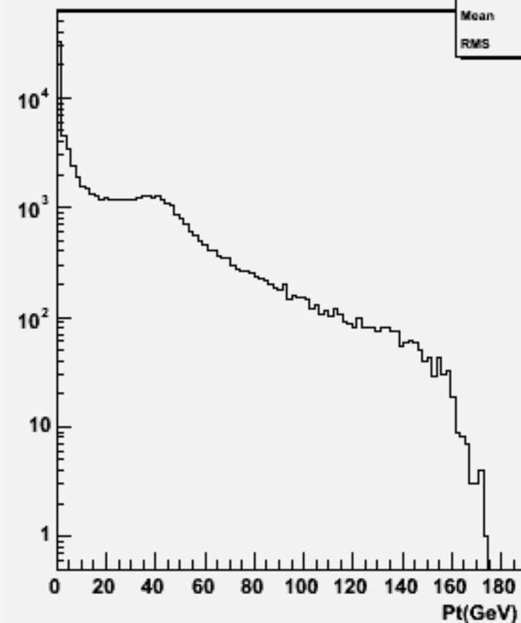
Particle Pt : w102730 n1n1aaa_o
