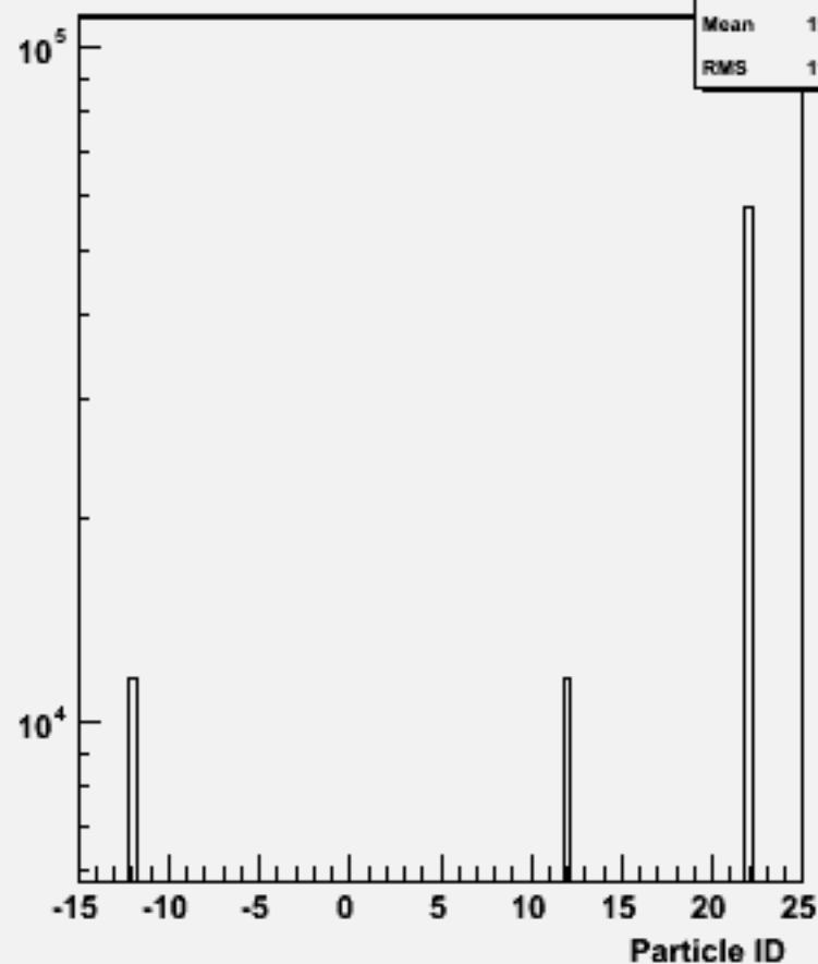
Particle ID : w102730 n1n1aaa_o
