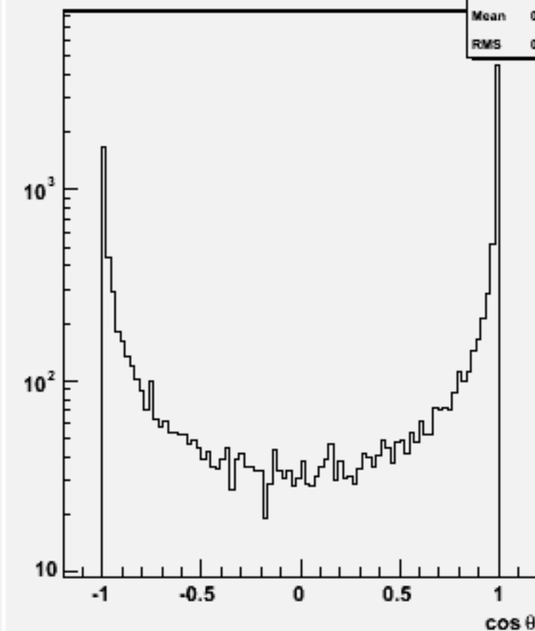
Jet cos \theta (All jets)w102730 n1n1aaa_o
