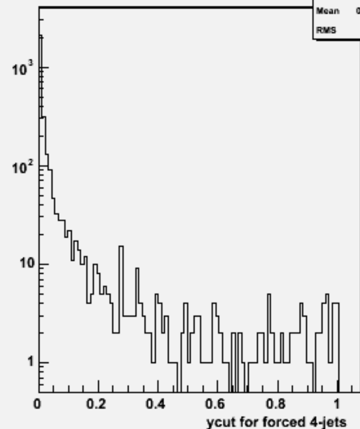
Ycut for 4-jets :w102730 n1n1aaa_o
