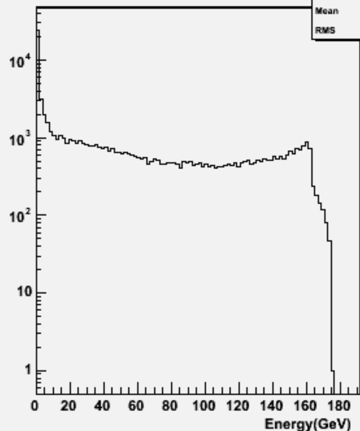
Particle Energy : w102730 n1n1aaa_o
