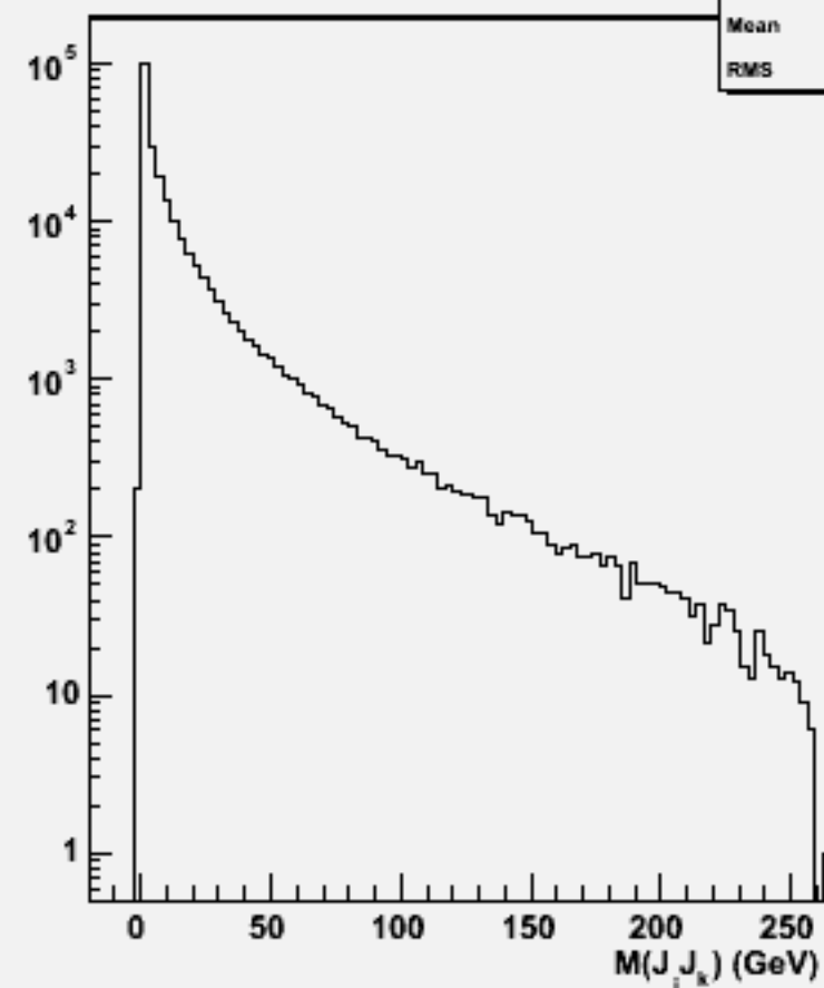
2jets mass(All comb)w102729 n1n1aaa_o
