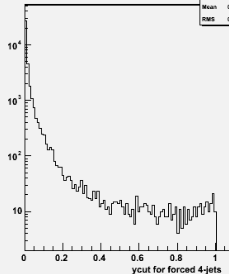
Ycut for 4-jets :w102729 n1n1aaa_o
