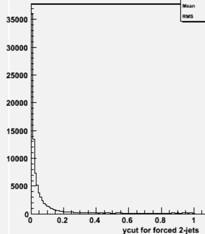
Ycut for 2-jets :w102729 n1n1aaa_o
