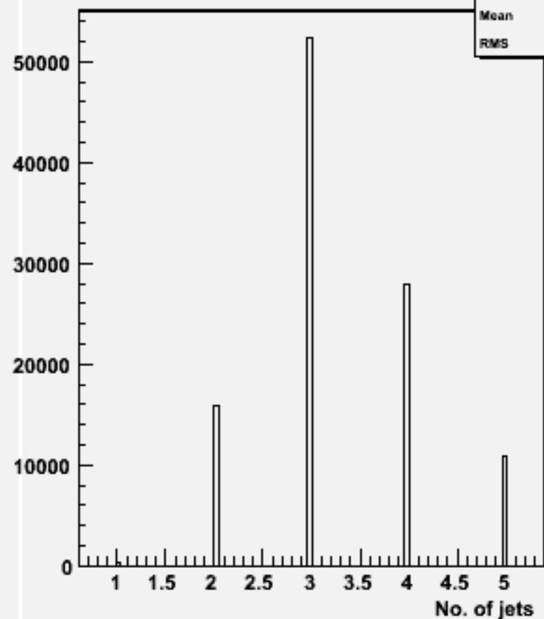
No. jets (ycut=0.001) : w102729 n1n1aaa_o
