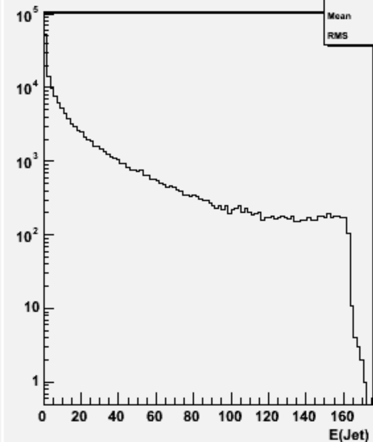
Jet energies(All jets)w102729 n1n1aaa_o
