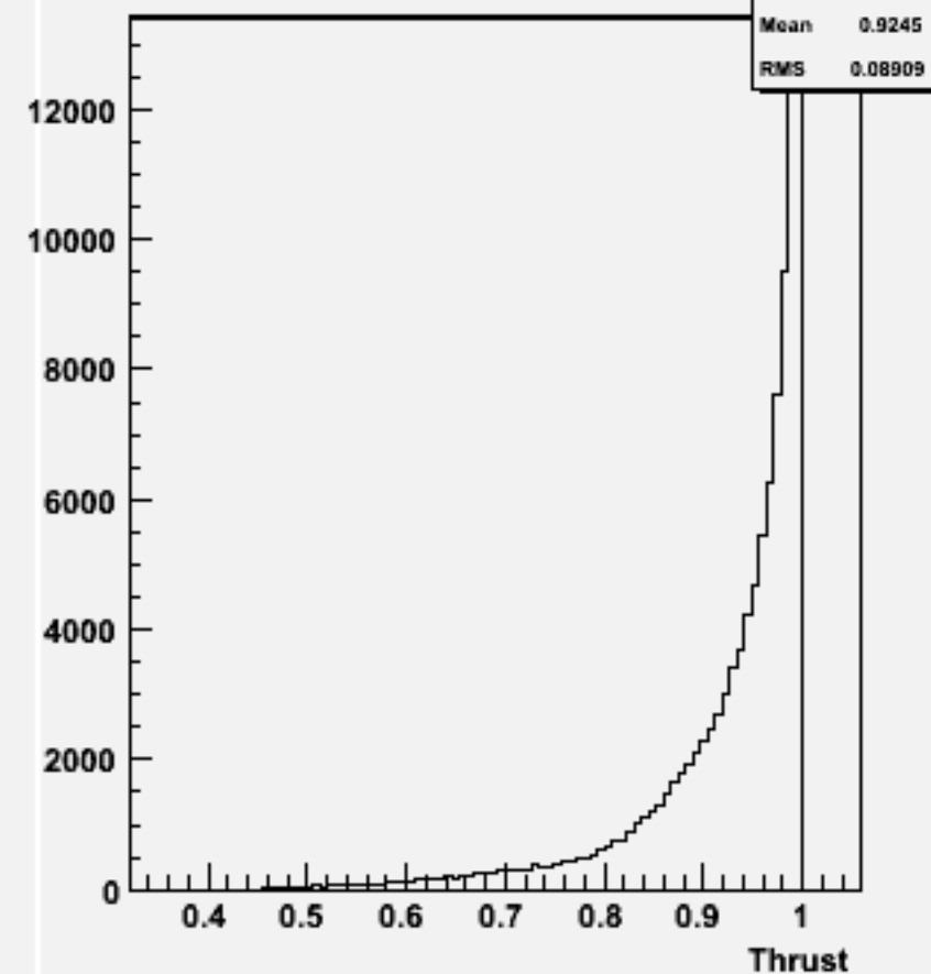
Thrust w102729 n1n1aaa_o
