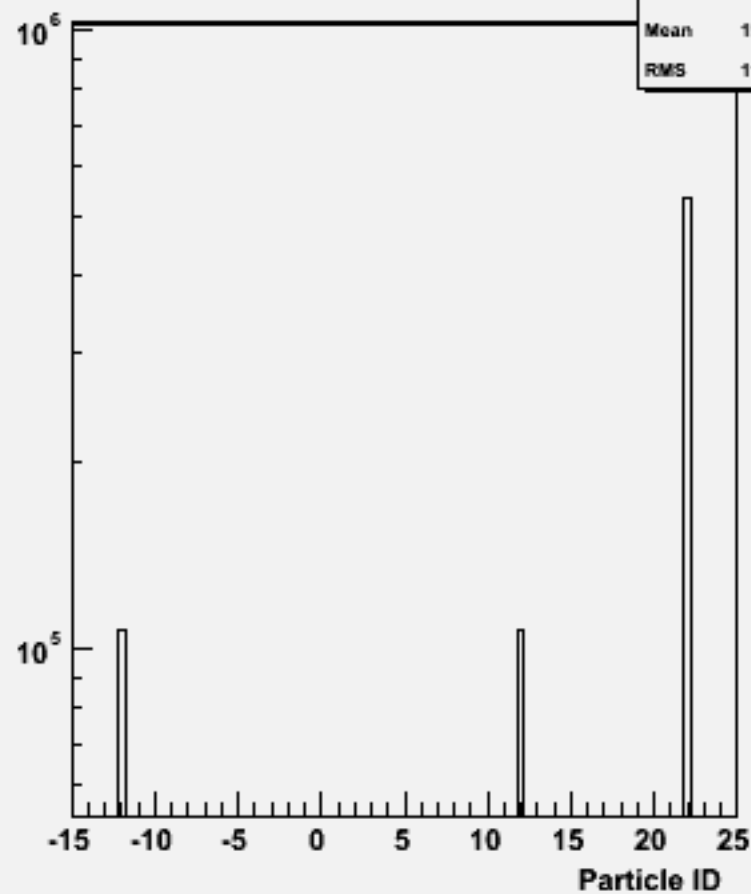
Particle ID : w102729 n1n1aaa_o
