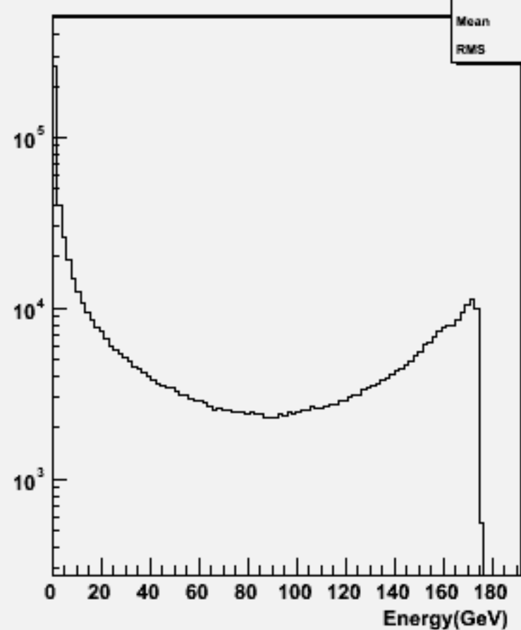
Particle Energy : w102729 n1n1aaa_o
