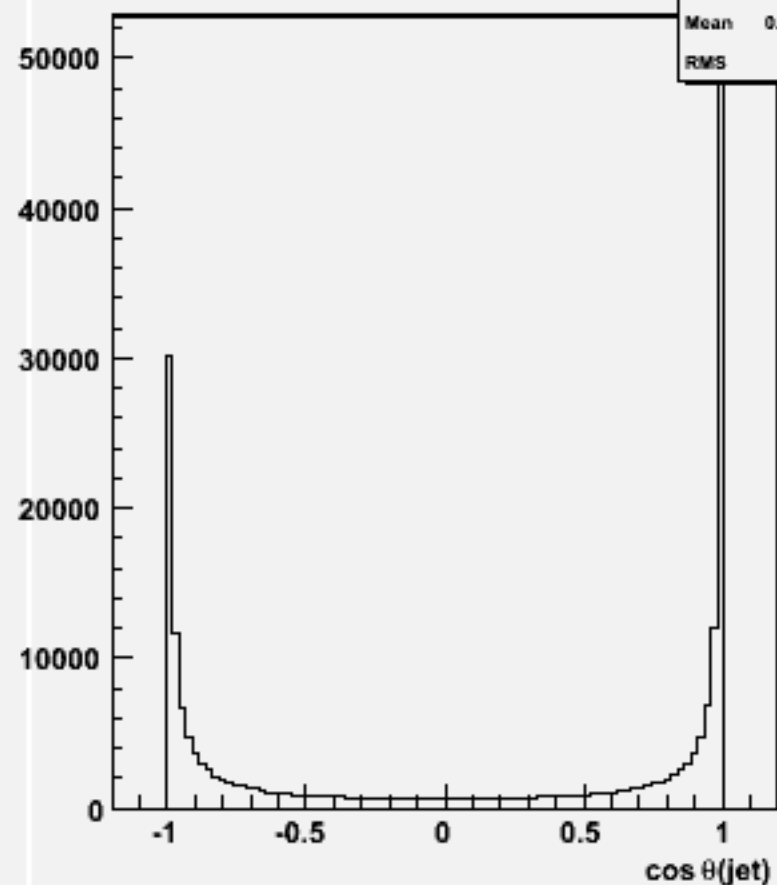
cos \theta for 2-jets :w102729 n1n1aaa_o
