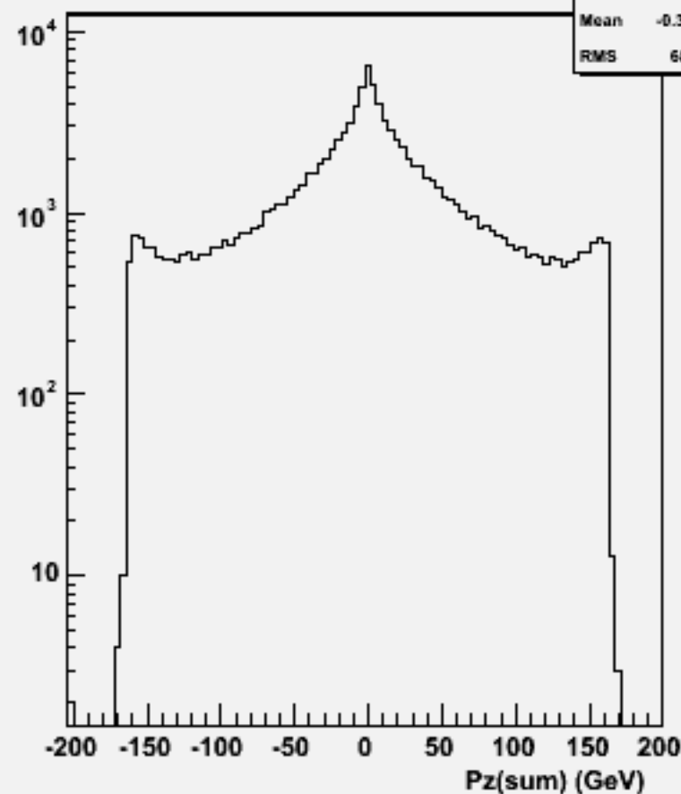
Pz Sum: w102729 n1n1aaa_o
