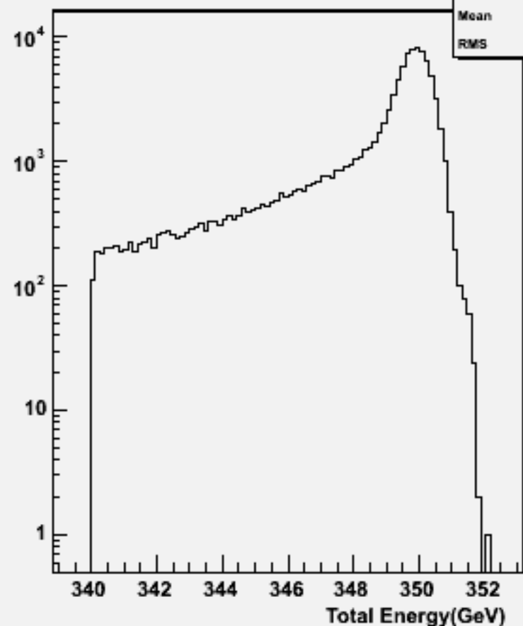
Total Energy (inc. \nu ): w102729 n1n1aaa_o
