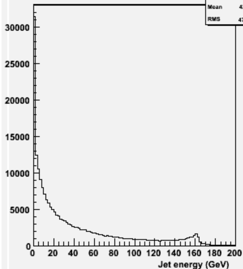
energy for 2-jets :w102729 n1n1aaa_o
