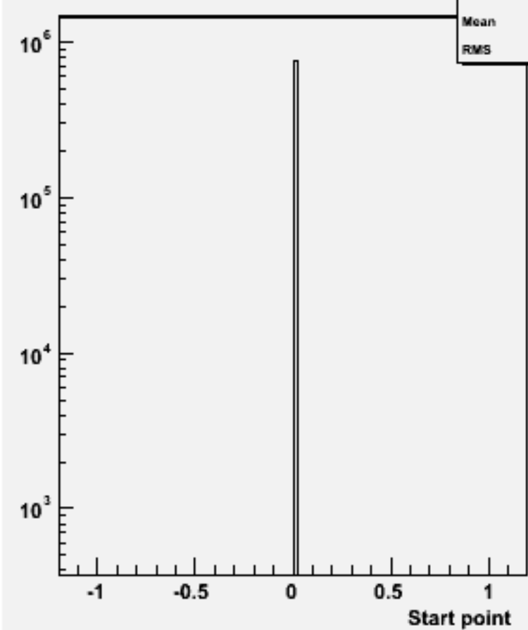
Start point Z : w102729 n1n1aaa_o
