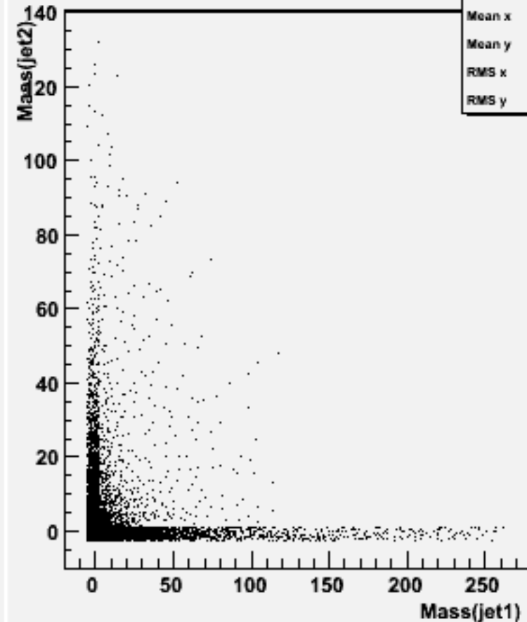
Jet mass for forced 2-jets : w102729 n1n1aaa_o
