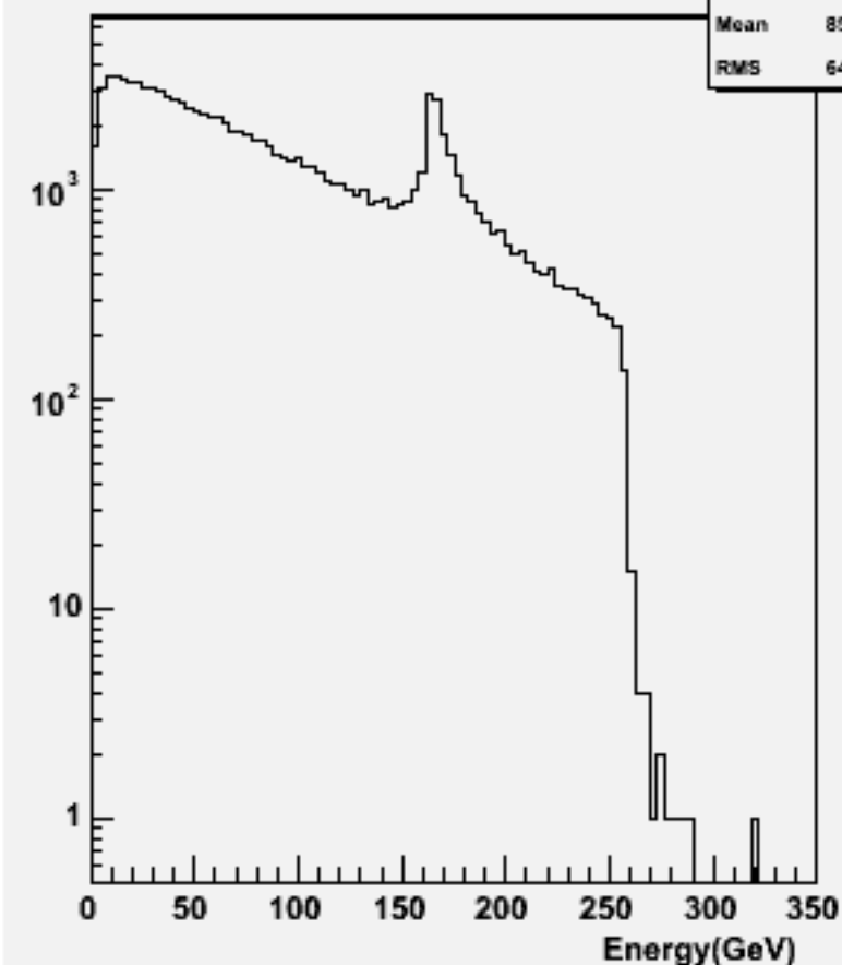
Total Energy (w/o \nu ): w102729 n1n1aaa_o
