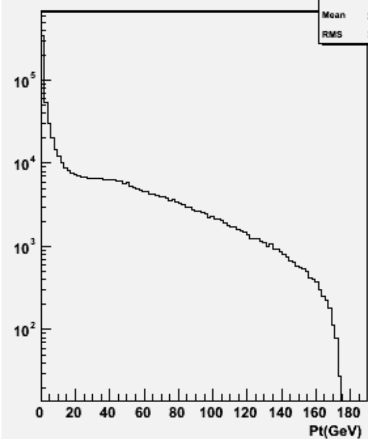
Particle Pt : w102729 n1n1aaa_o
