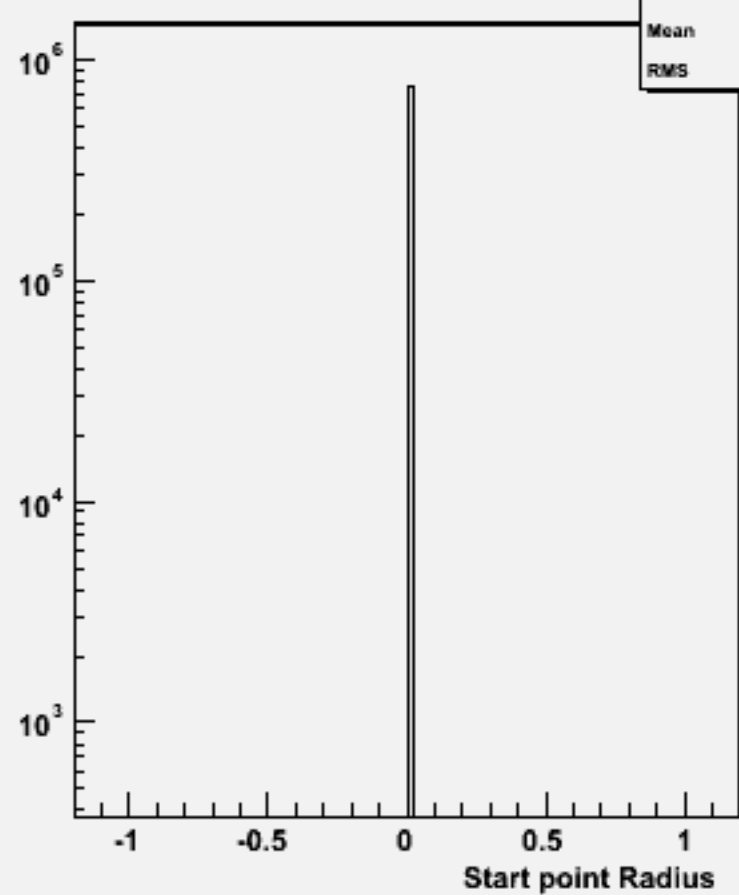
Start point R : w102729 n1n1aaa_o
