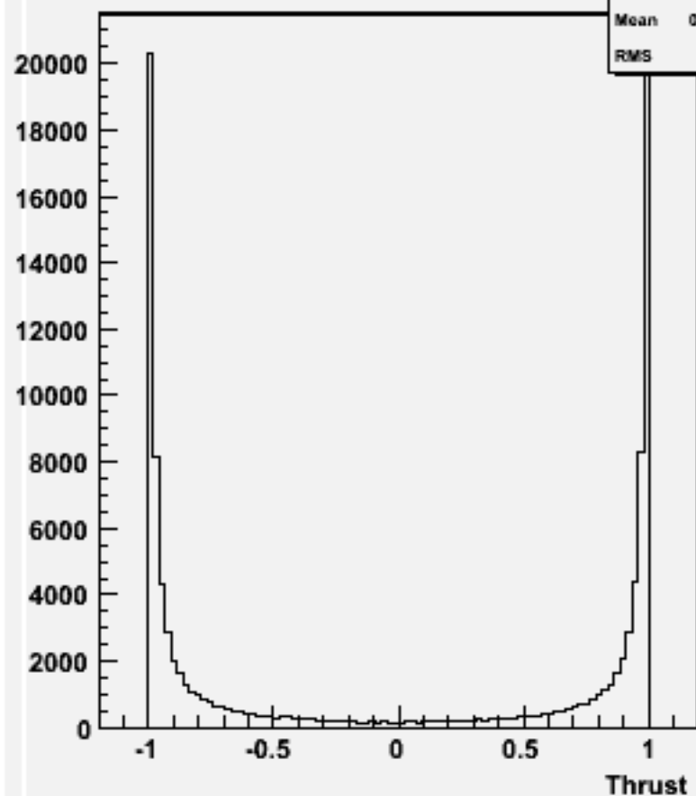
cos \Theta (thrust) w102729 n1n1aaa_o
