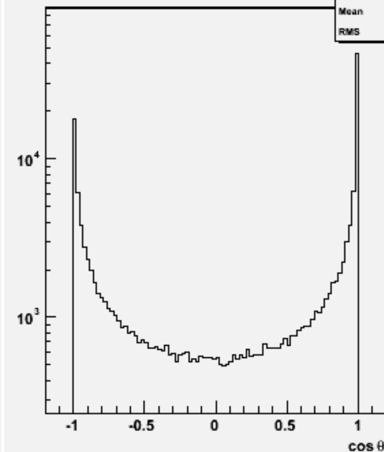
Jet cos \theta (All jets)w102729 n1n1aaa_o
