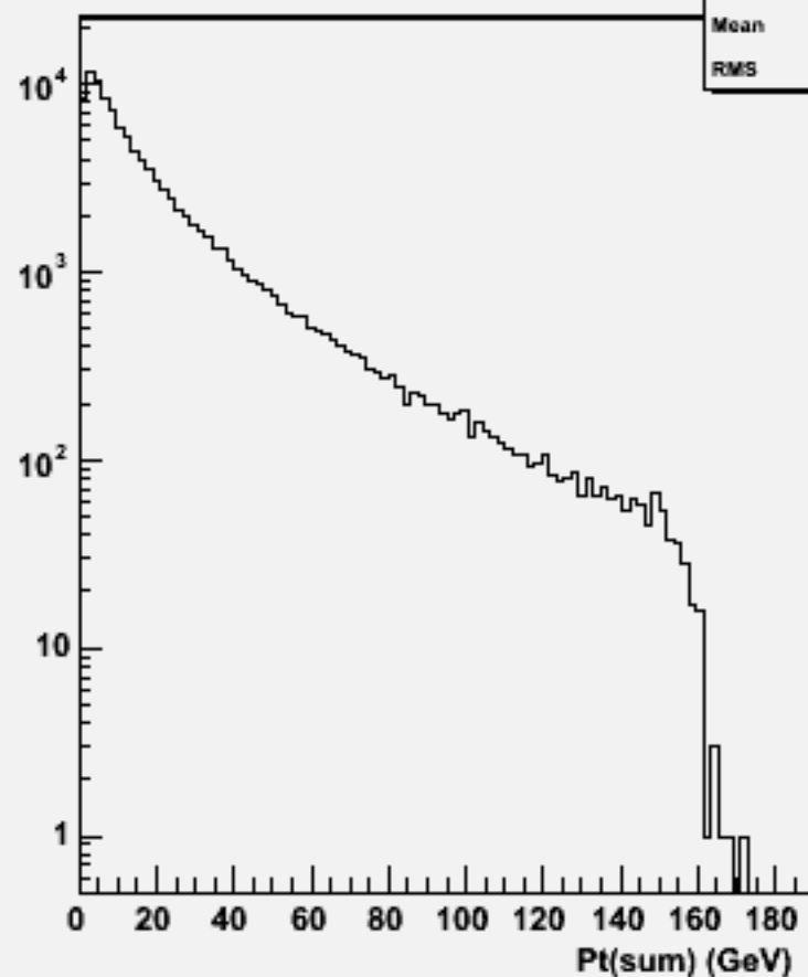
Pt Sum: w102729 n1n1aaa_o
