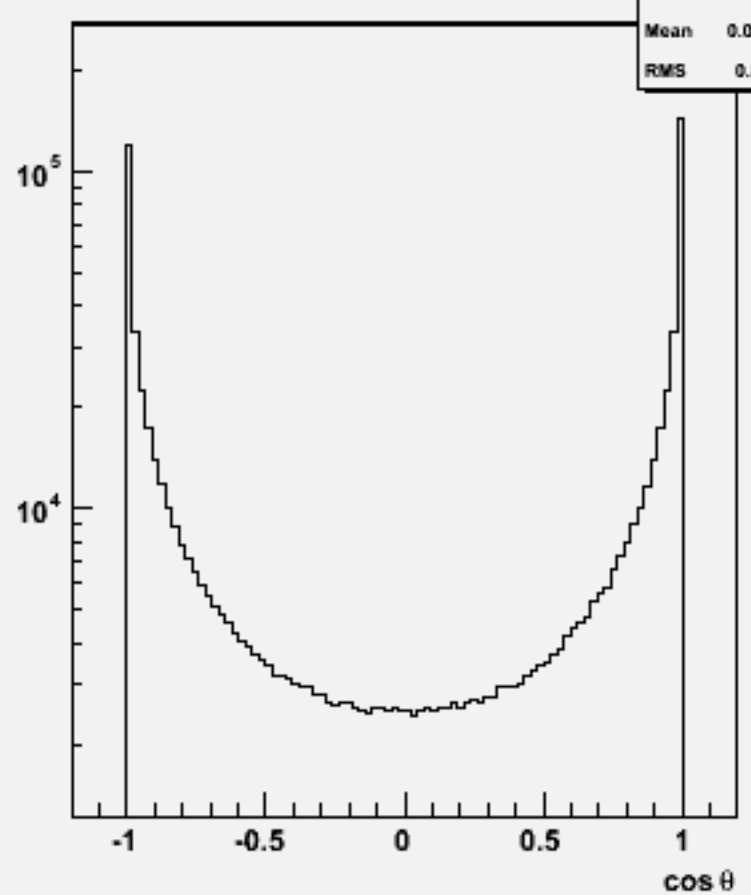
Particle \cos\theta : w102729 n1n1aaa_o
