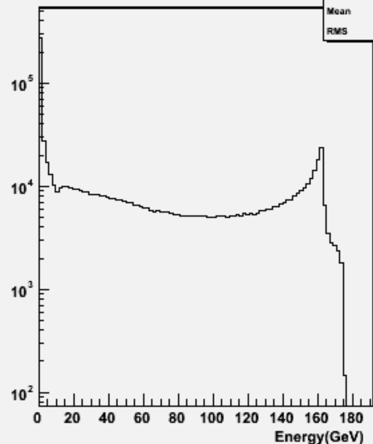
Particle Energy : w102726 n3n3aa_o
