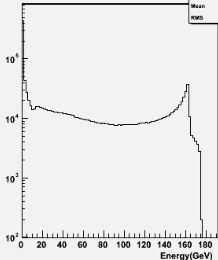
Particle Energy : w102725 n3n3aa_o
