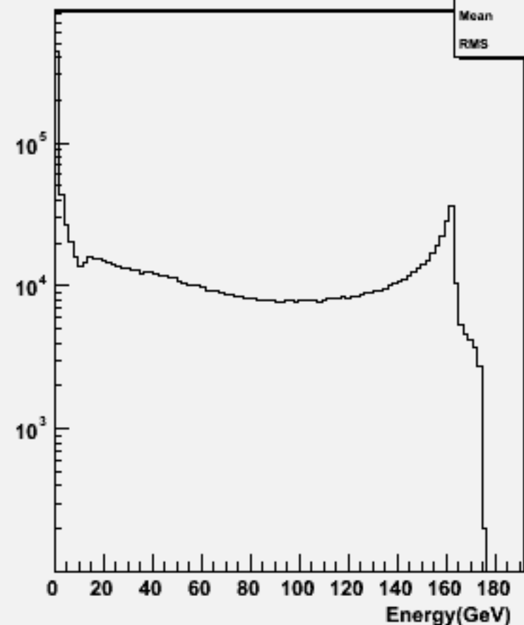
Particle Energy : w102721 n2n2aa_o
