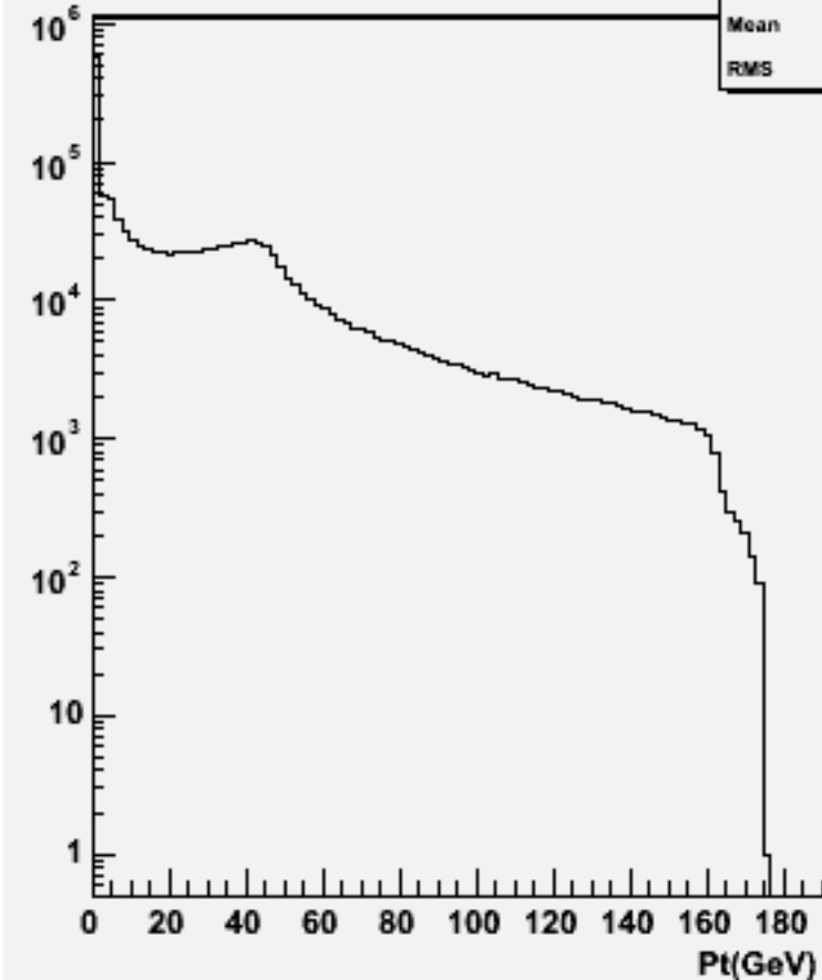
Particle Pt : w102721 n2n2aa_o
