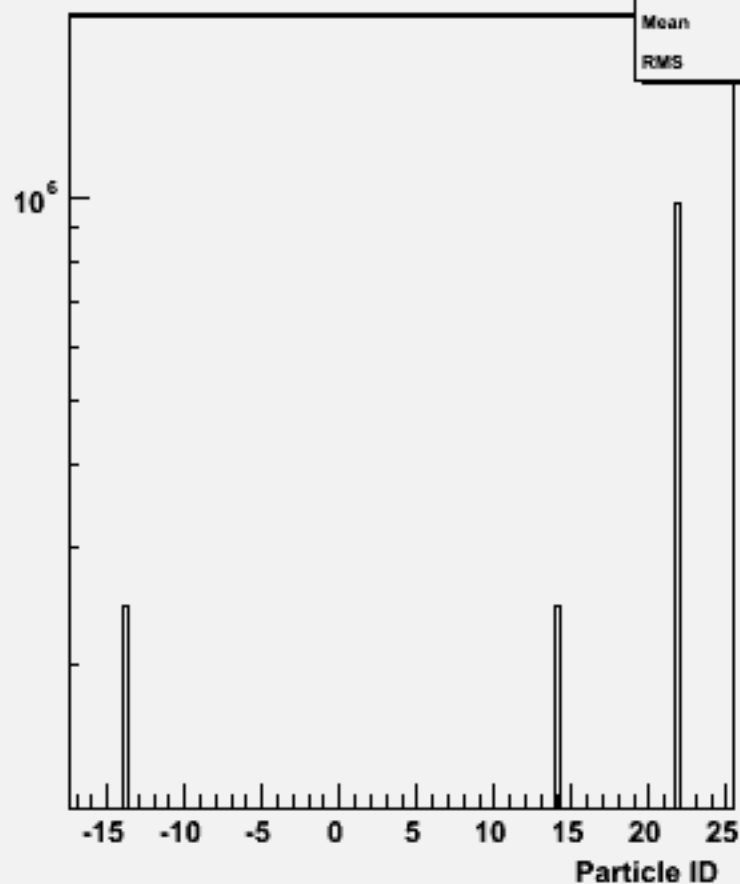
Particle ID : w102721 n2n2aa_o
