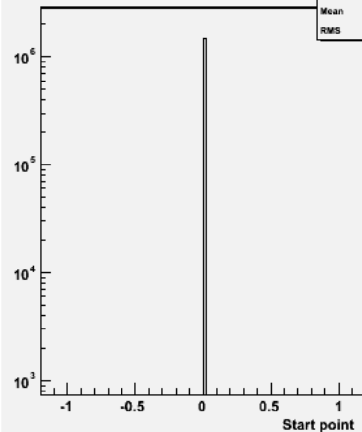
Start point Z : w102721 n2n2aa_o
