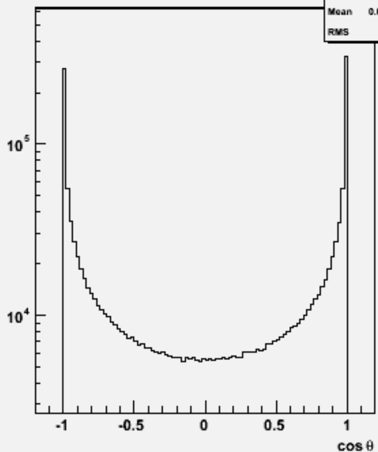
Particle cos \theta : w102721 n2n2aa_o
