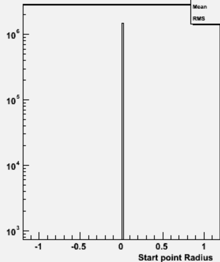
Start point R : w102721 n2n2aa_o
