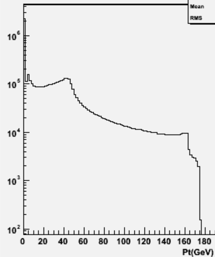
Particle Pt : w102710 n2n2a_o
