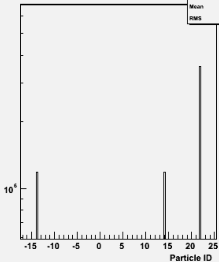
Particle ID : w102710 n2n2a_o
