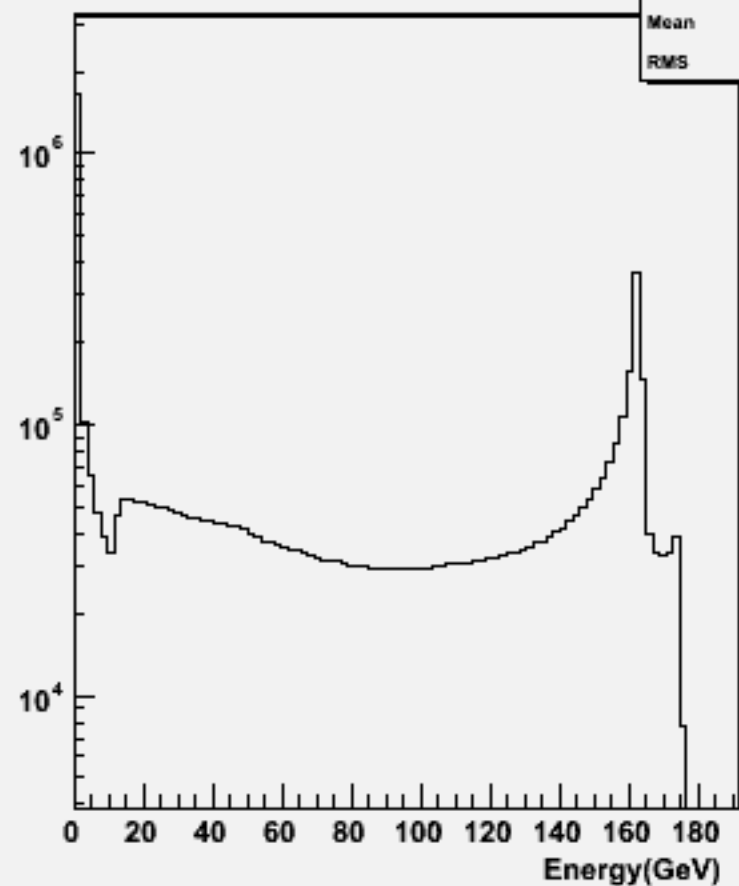
Particle Energy : w102710 n2n2a_o
