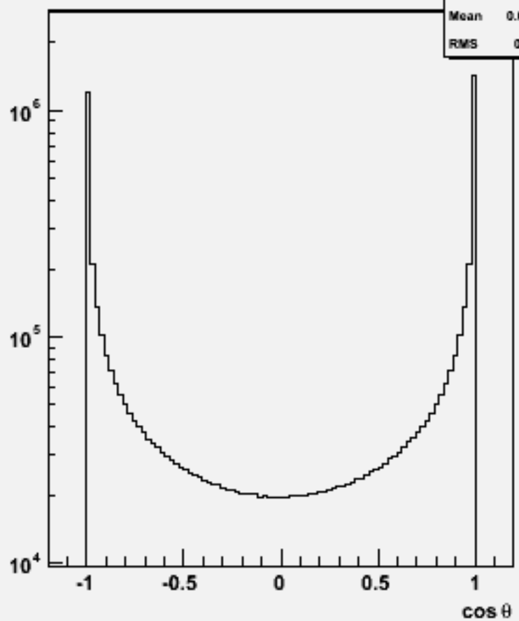
Particle cos \theta : w102710 n2n2a_o
