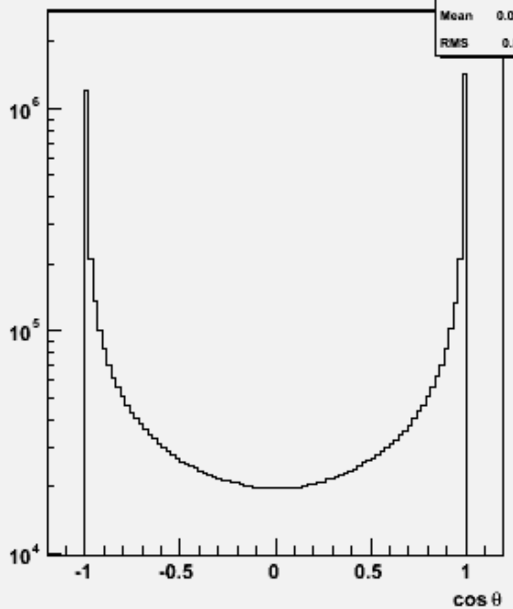
Particle \cos\theta : w102706 n1n1a_o
