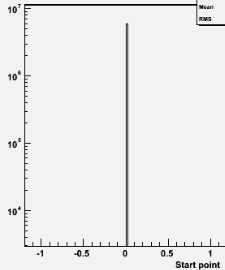
Start point Z : w102706 n1n1a_o
