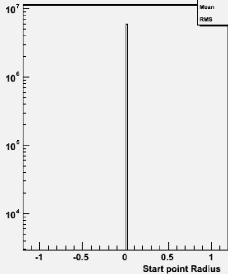
Start point R : w102706 n1n1a_o
