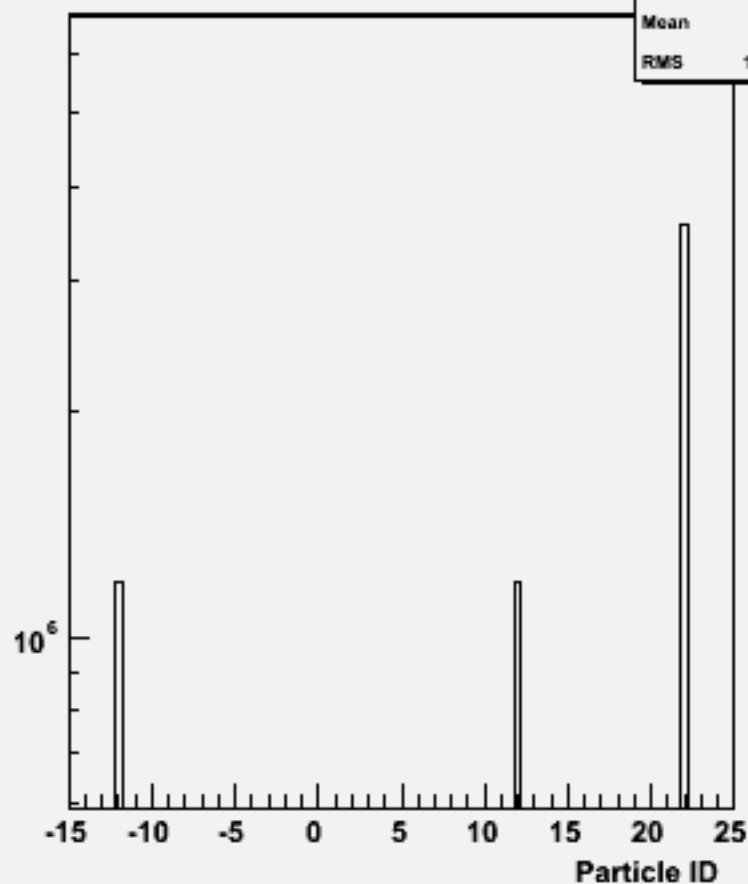
Particle ID : w102706 n1n1a_o
