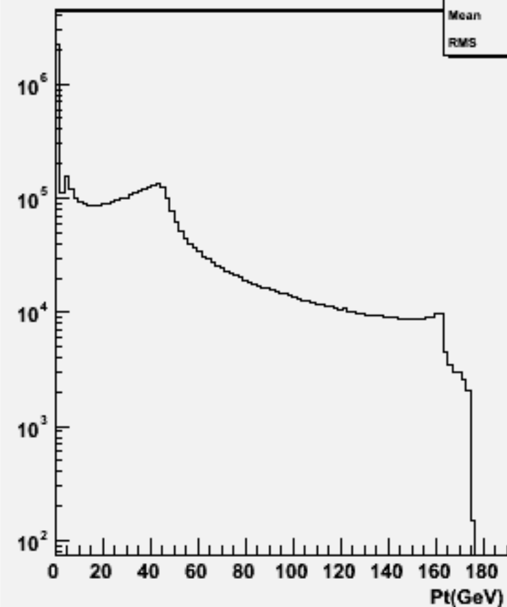
Particle Pt : w102706 n1n1a_o
