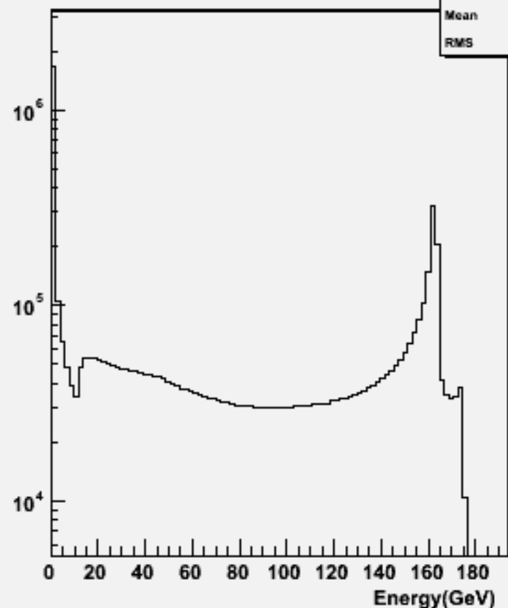
Particle Energy : w102706 n1n1a_o
