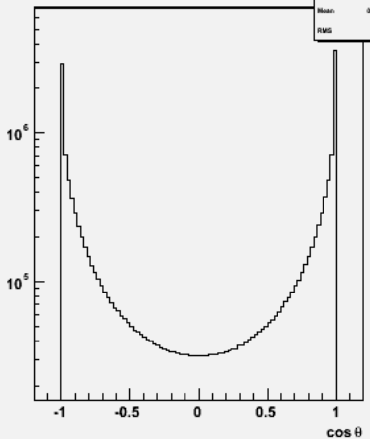
Particle \cos\theta : w102705 n1n1a_o
