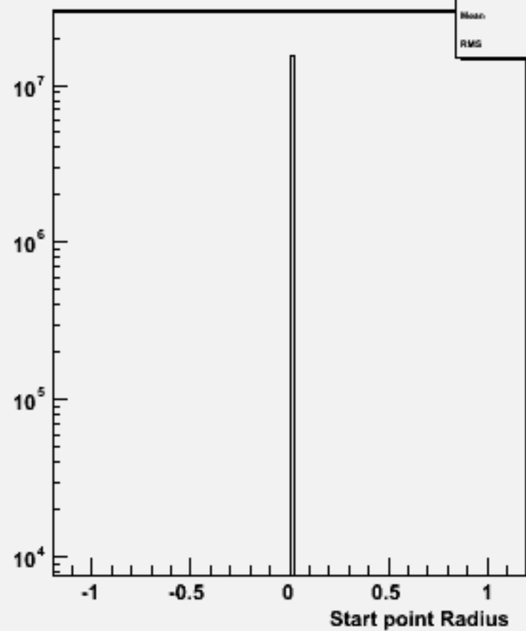
Start point R : w102705 n1n1a_o
