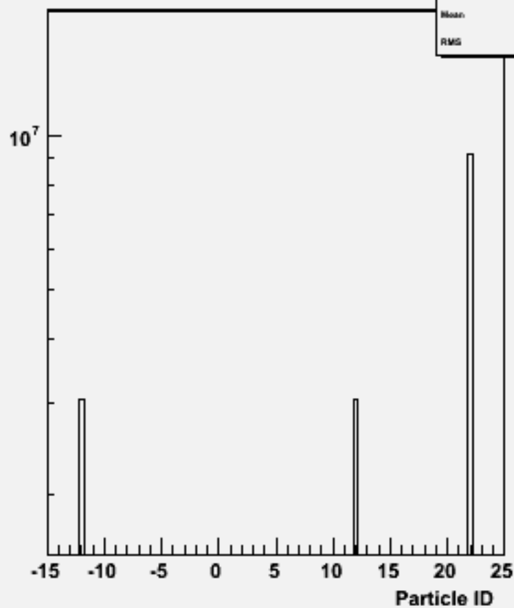
Particle ID : w102705 n1n1a_o
