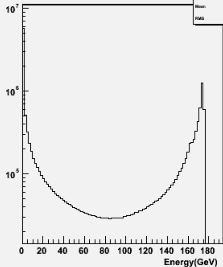
Particle Energy : w102705 n1n1a_o
