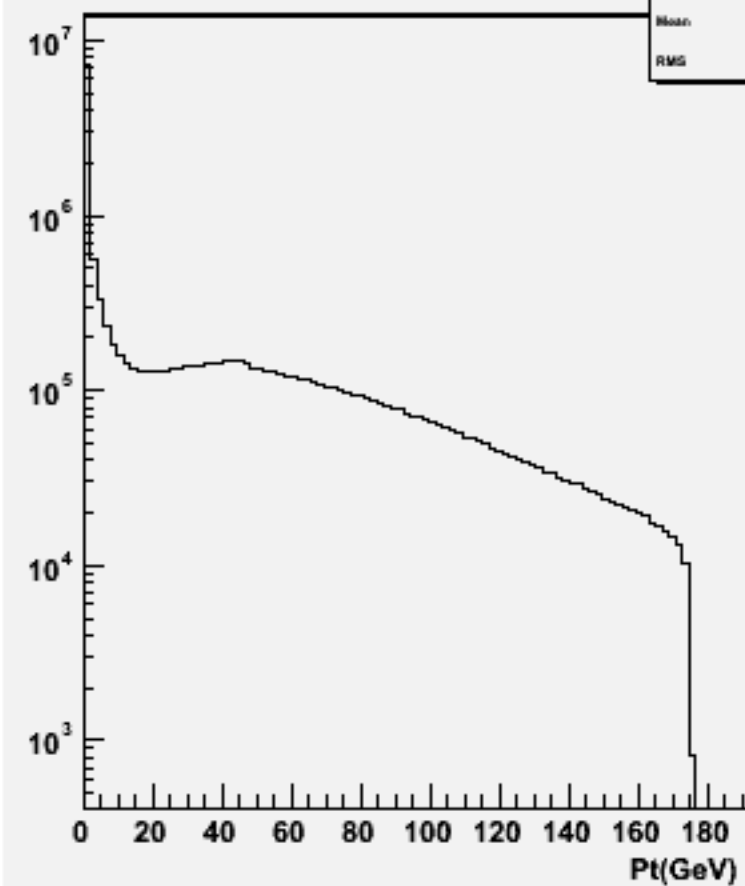
Particle Pt : w102705 n1n1a_o
