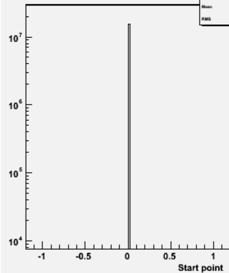
Start point Z : w102705 n1n1a_o
