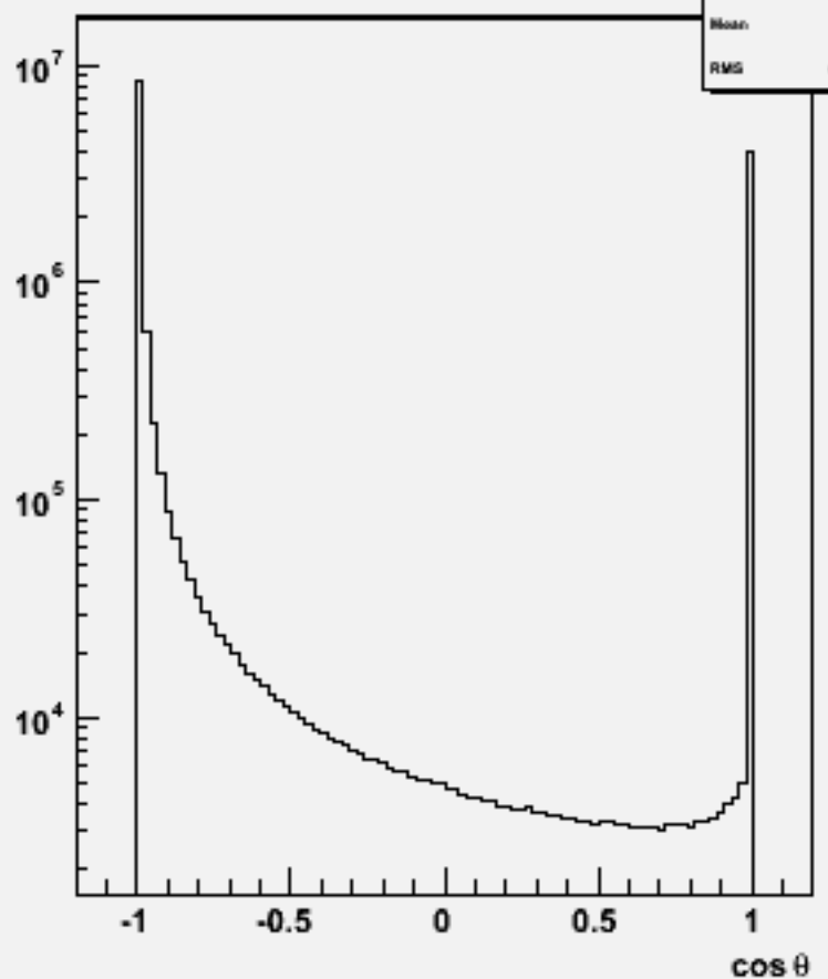
Particle cosθ : w102702 ae1_e1a_o
