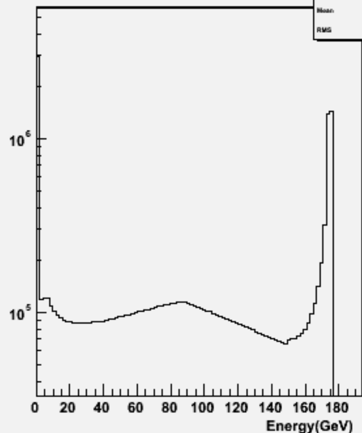
Particle Energy : w102702 ae1_e1a_o
