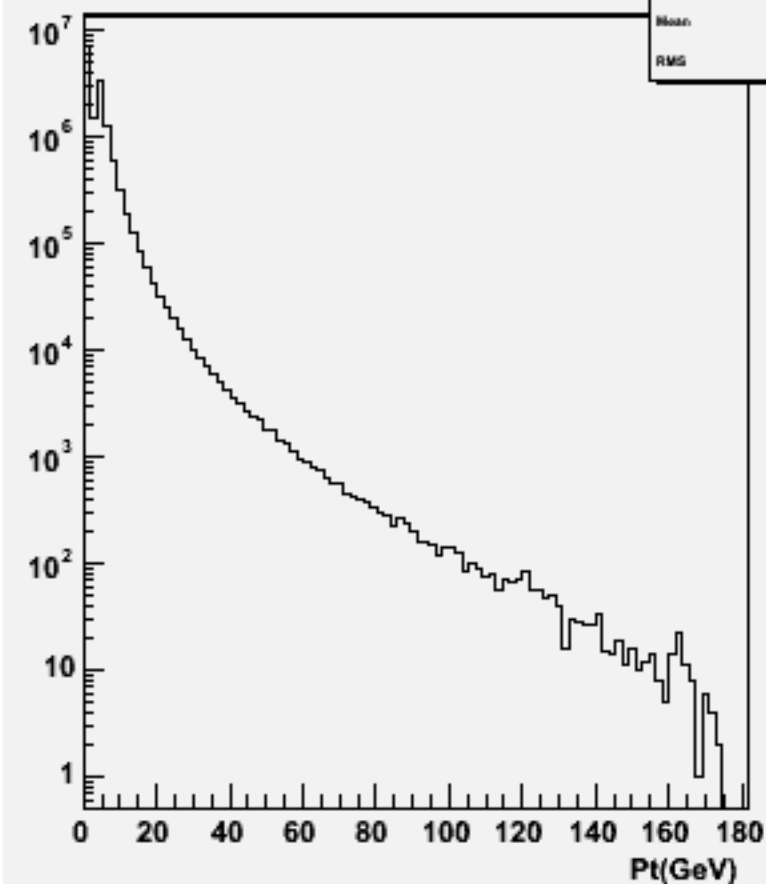
Particle Pt : w102702 ae1_e1a_o
