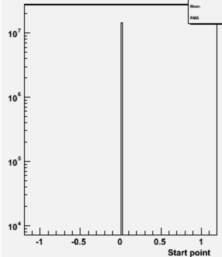
Start point Z : w102702 ae1_e1a_o
