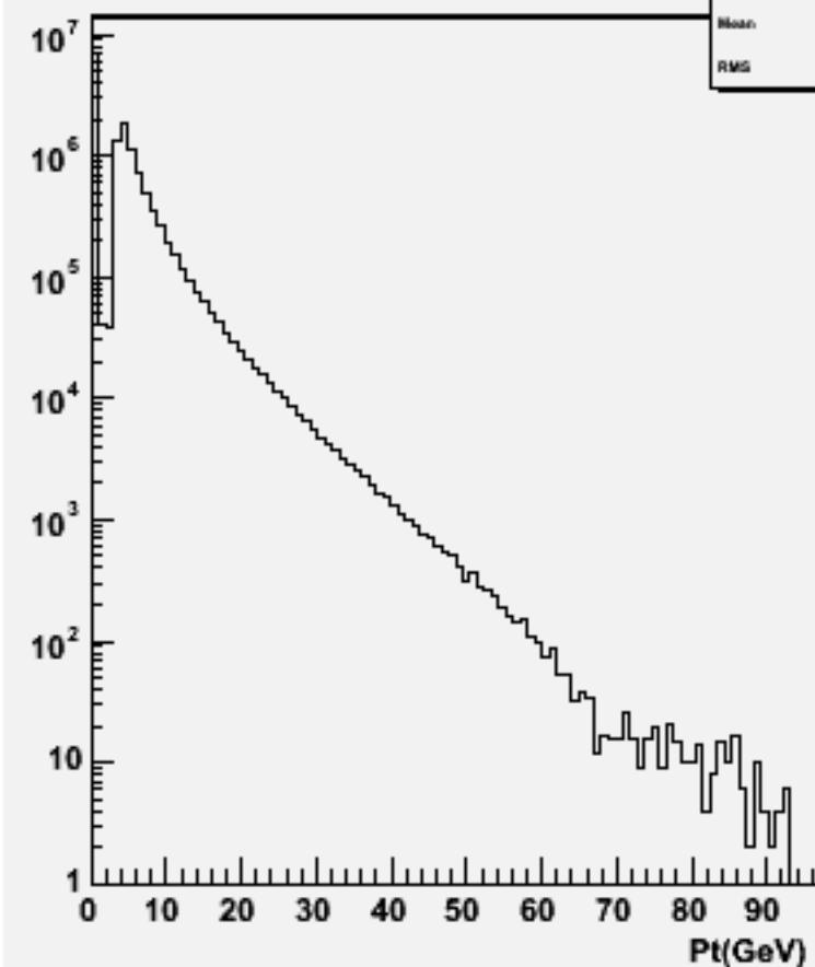
Particle Pt : w102697 e1a_e1a_o
