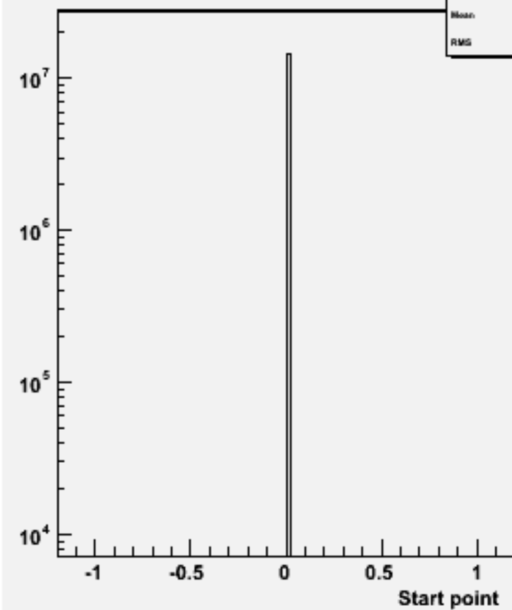
Start point Z : w102697 e1a_e1a_o
