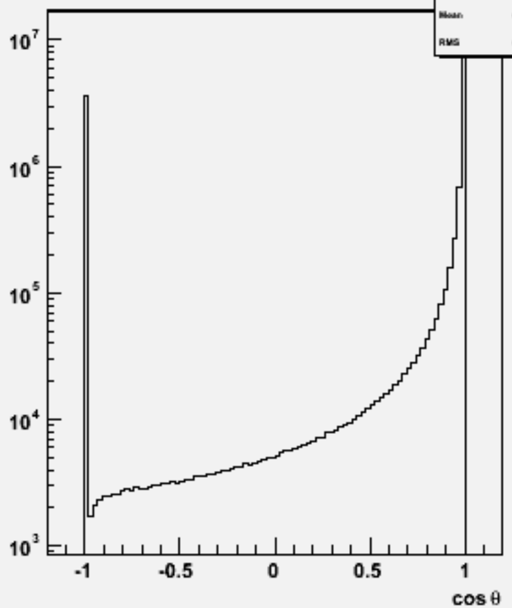
Particle \cos\theta : w102697 e1a_e1a_o
