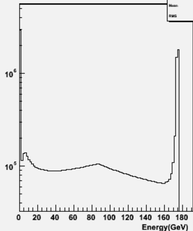
Particle Energy : w102697 e1a_e1a_o
