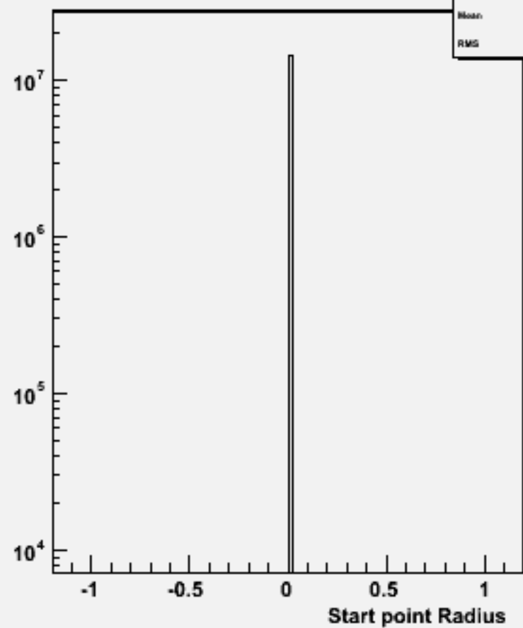
Start point R : w102697 e1a_e1a_o
