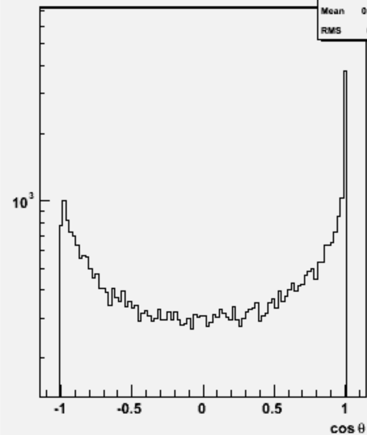
Jet cos \theta (All jets)w102593 e2e2ssbb_o
