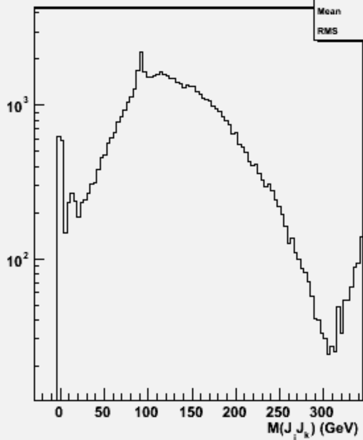
2jets mass(All comb)w102593 e2e2ssbb_o
