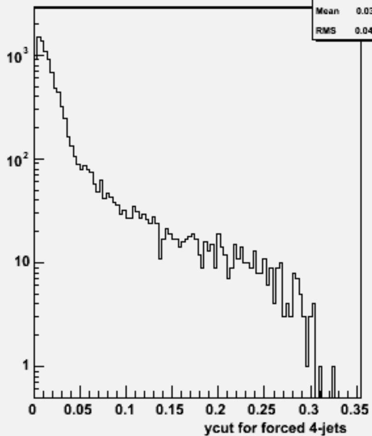
Ycut for 4-jets :w102593 e2e2ssbb_o
