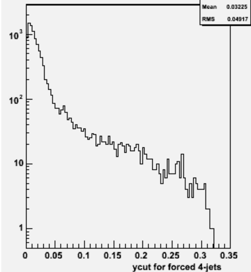
Ycut for 4-jets :w102589 e2e2ssss_o
