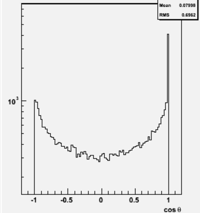
Jet cos \theta (All jets)w102589 e2e2ssss_o
