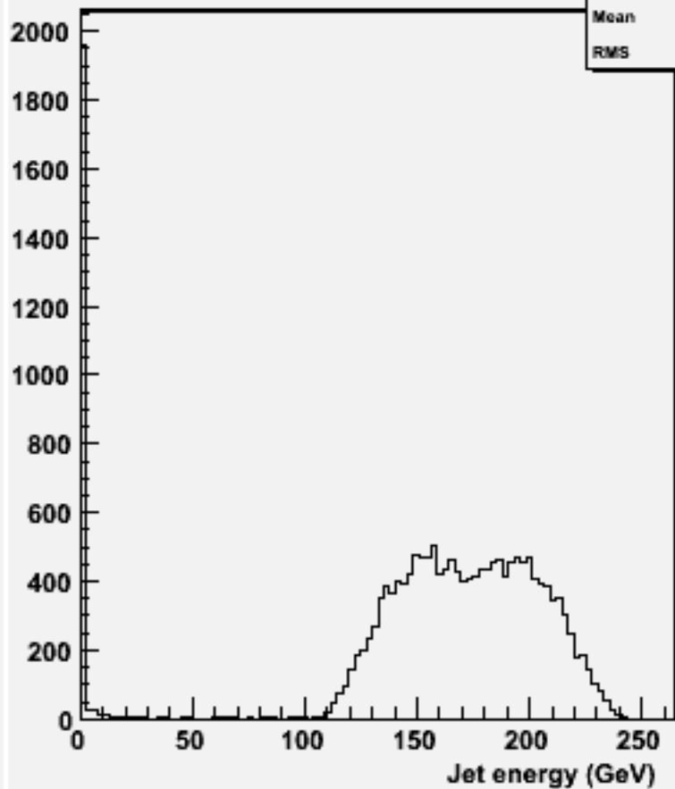
energy for 2-jets :w102589 e2e2ssss_o
