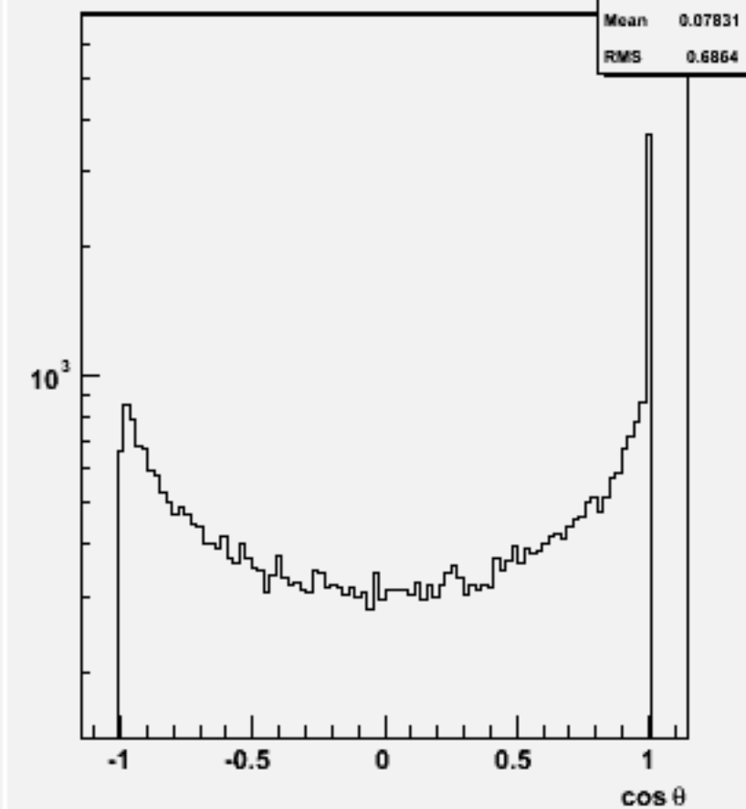
Jet cosθ (All jets)w102588 e2e2ssss_o
