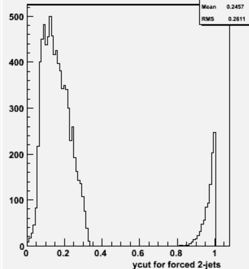
Ycut for 2-jets :w102588 e2e2ssss_o
