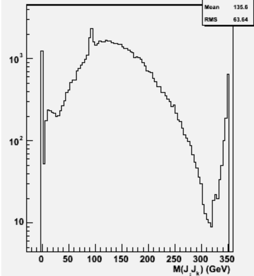
2jets mass(All comb)w102588 e2e2ssss_o
