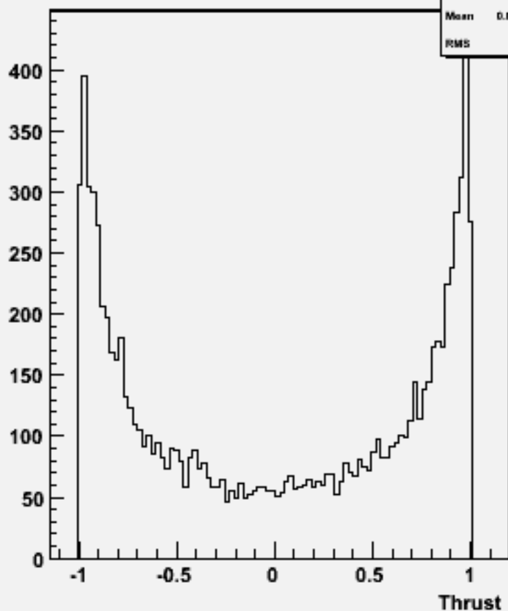
cos \Theta (thrust) w102588 e2e2ssss_o
