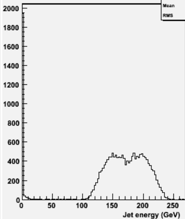
energy for 2-jets :w102588 e2e2ssss_o
