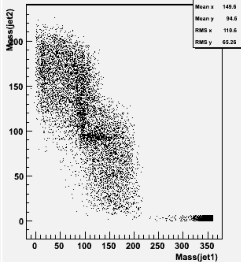
Jet mass for forced 2-jets : w102588 e2e2ssss_o
