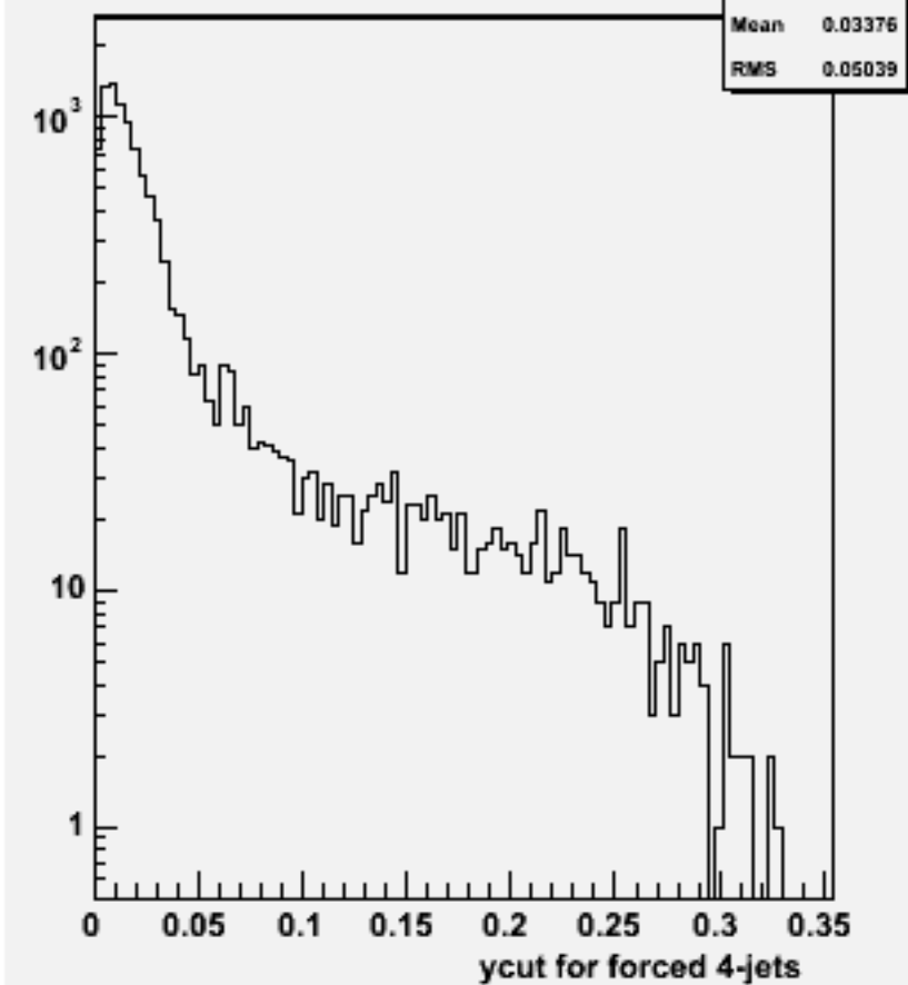
Ycut for 4-jets :w102588 e2e2ssss_o
