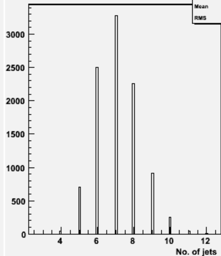
No. jets (ycut=0.001) : w102588 e2e2ssss_o
