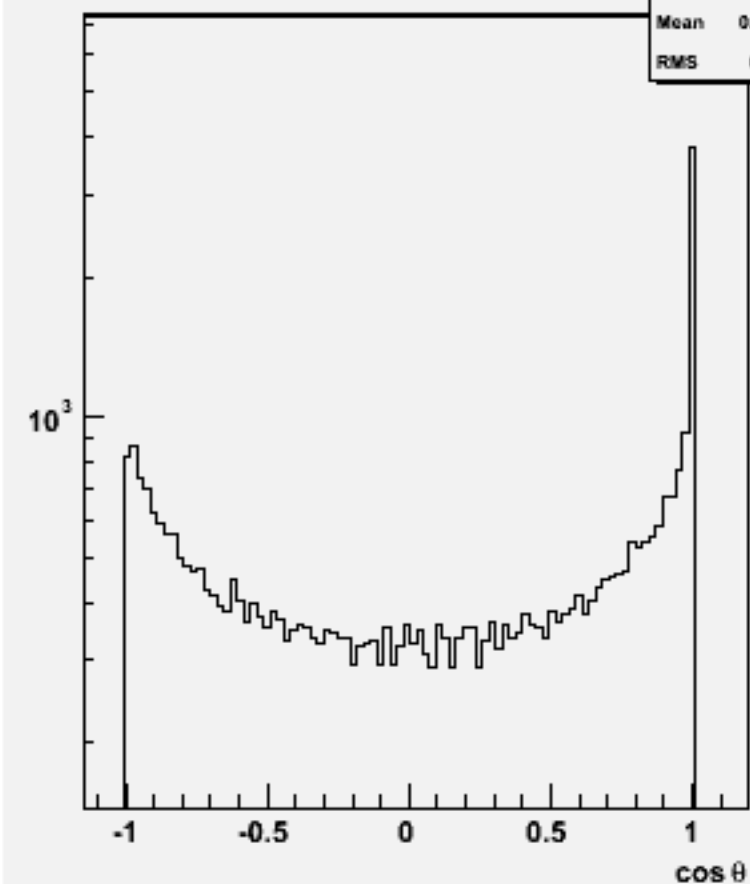
Jet cos \theta (All jets)w102584 e2e2ddb_o
