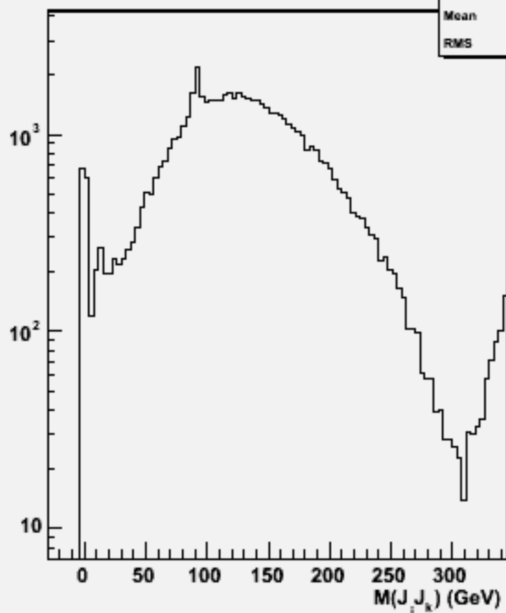
2jets mass(All comb)w102584 e2e2ddb_o
