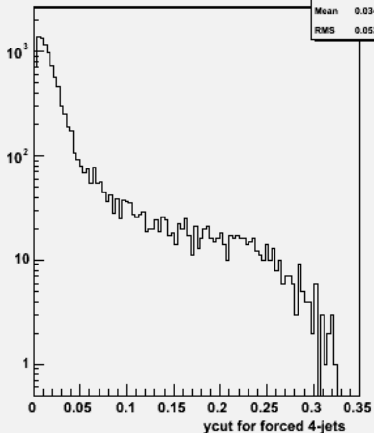
Ycut for 4-jets :w102584 e2e2ddb_o
