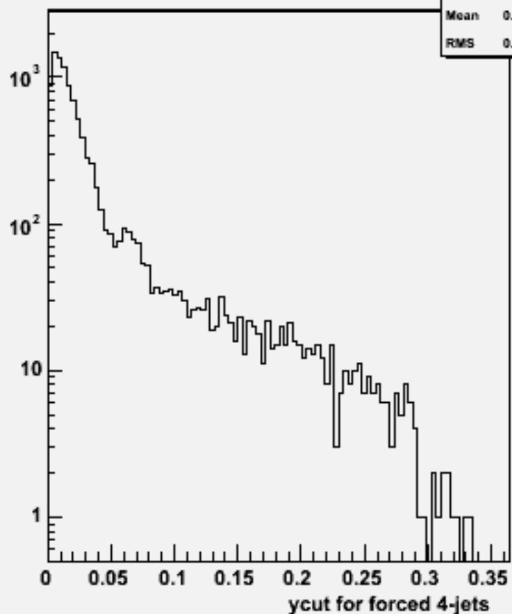
Ycut for 4-jets :w102581 e2e2ddss_o
