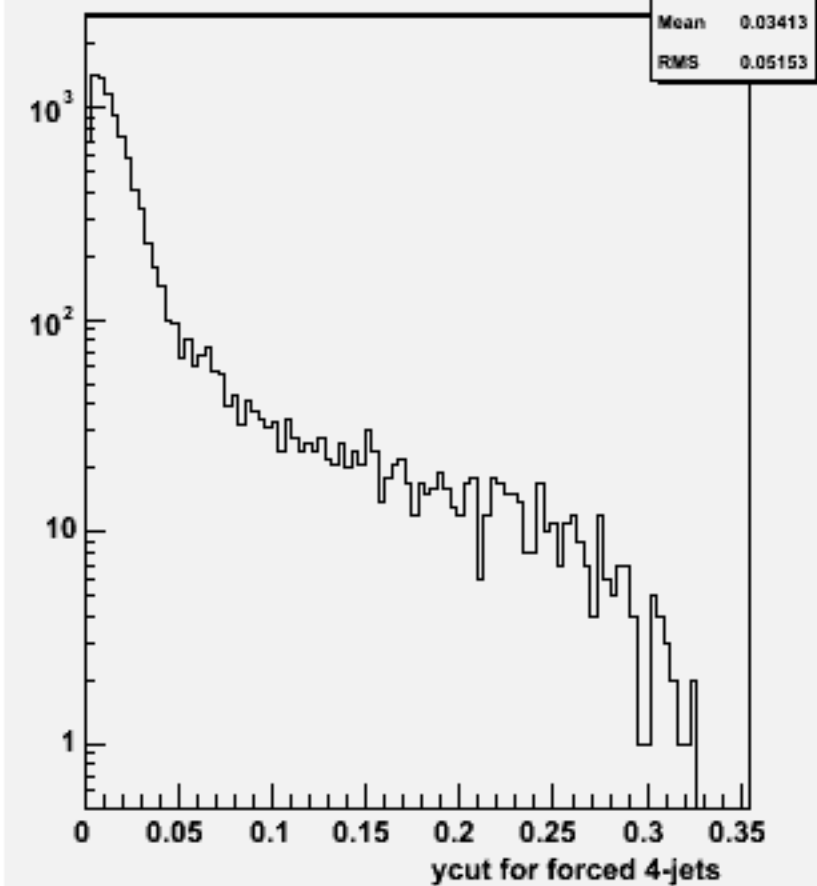
Ycut for 4-jets :w102576 e2e2dddd_o
