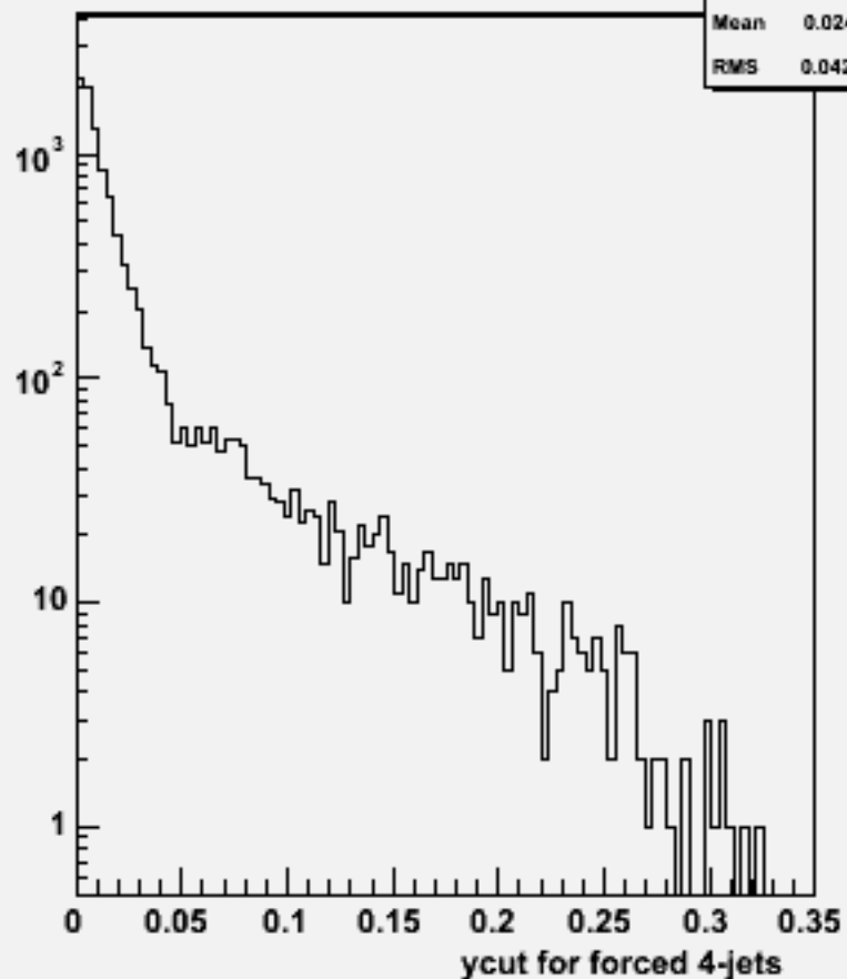
Ycut for 4-jets :w102573 e2e2e3e3bb_o
