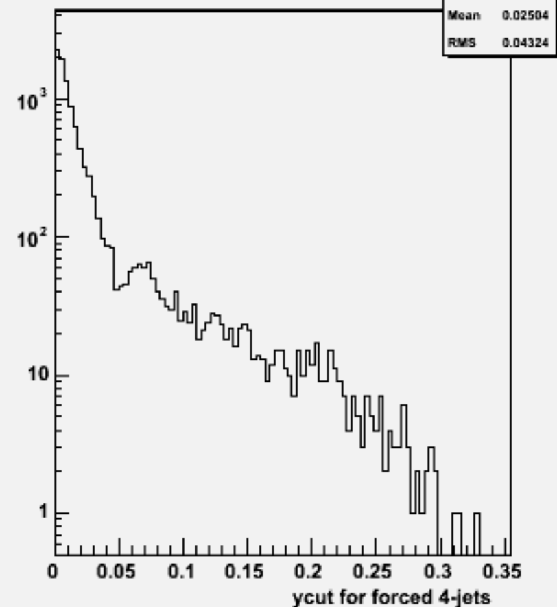
Ycut for 4-jets :w102569 e2e2e3e3ss_o
