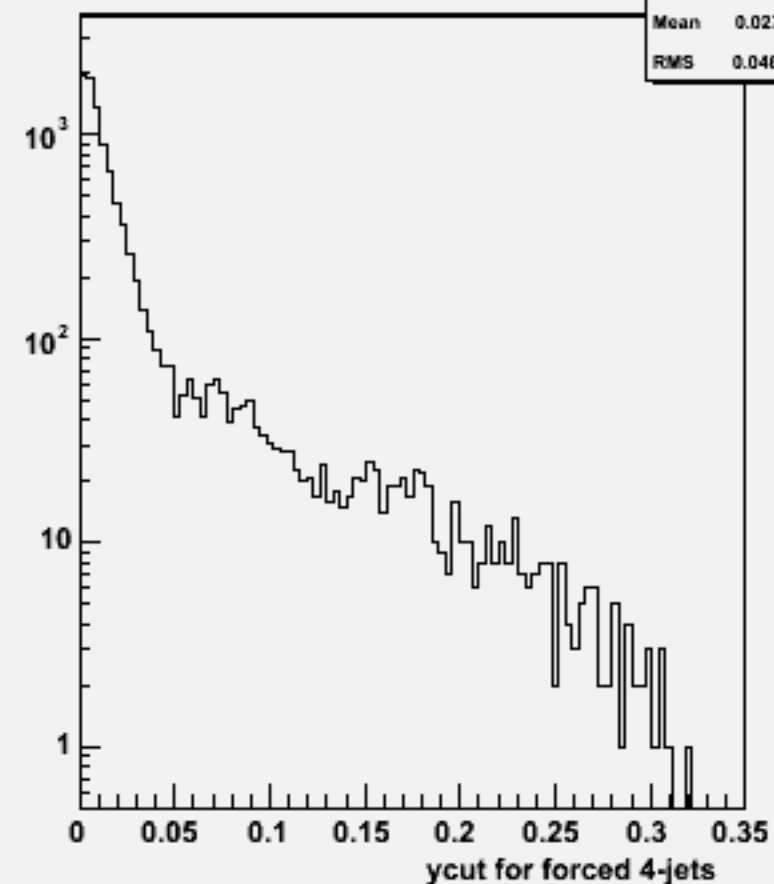
Ycut for 4-jets :w102568 e2e2e3e3ss_o
