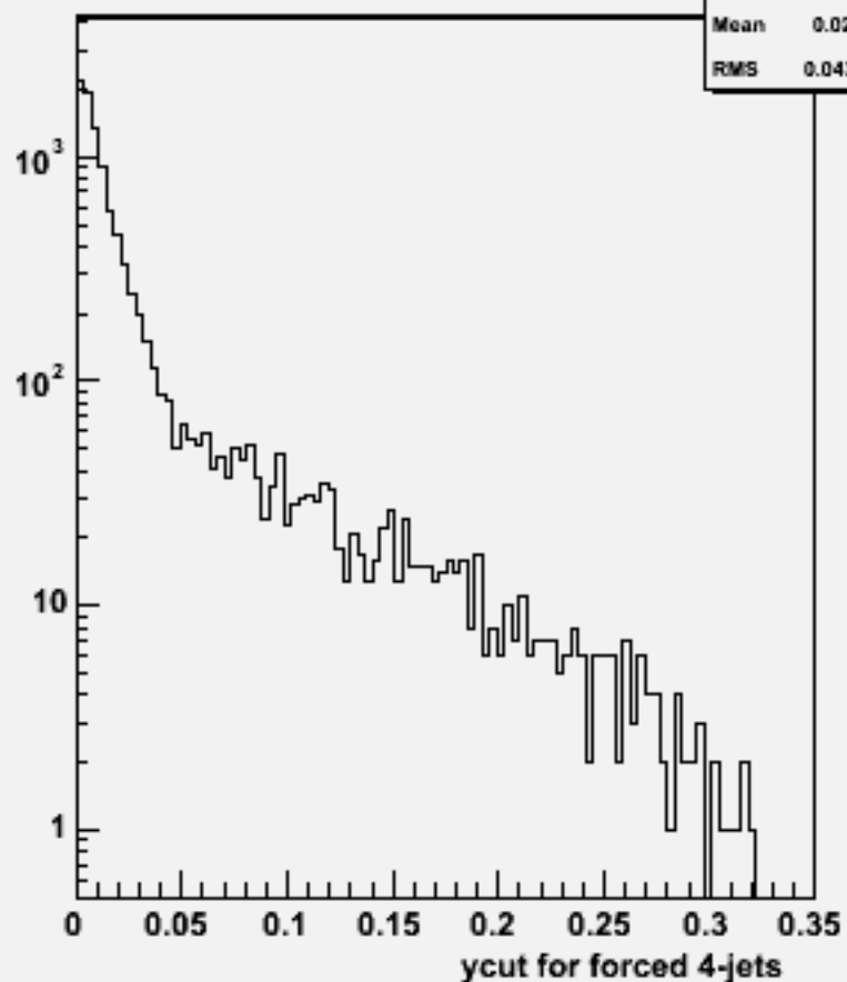
Ycut for 4-jets :w102565 e2e2e3e3dd_o
