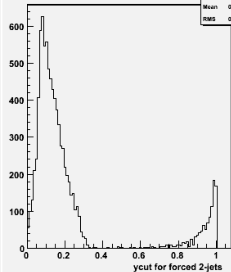
Ycut for 2-jets :w102565 e2e2e3e3dd_o
