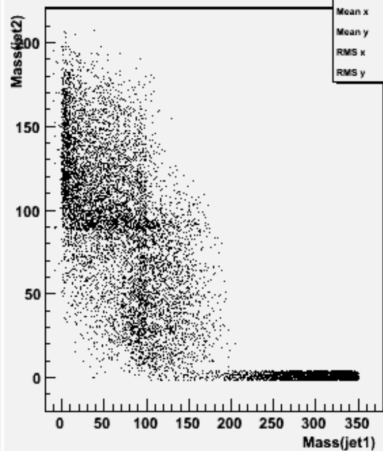
Jet mass for forced 2-jets : w102565 e2e2e3e3dd_o
