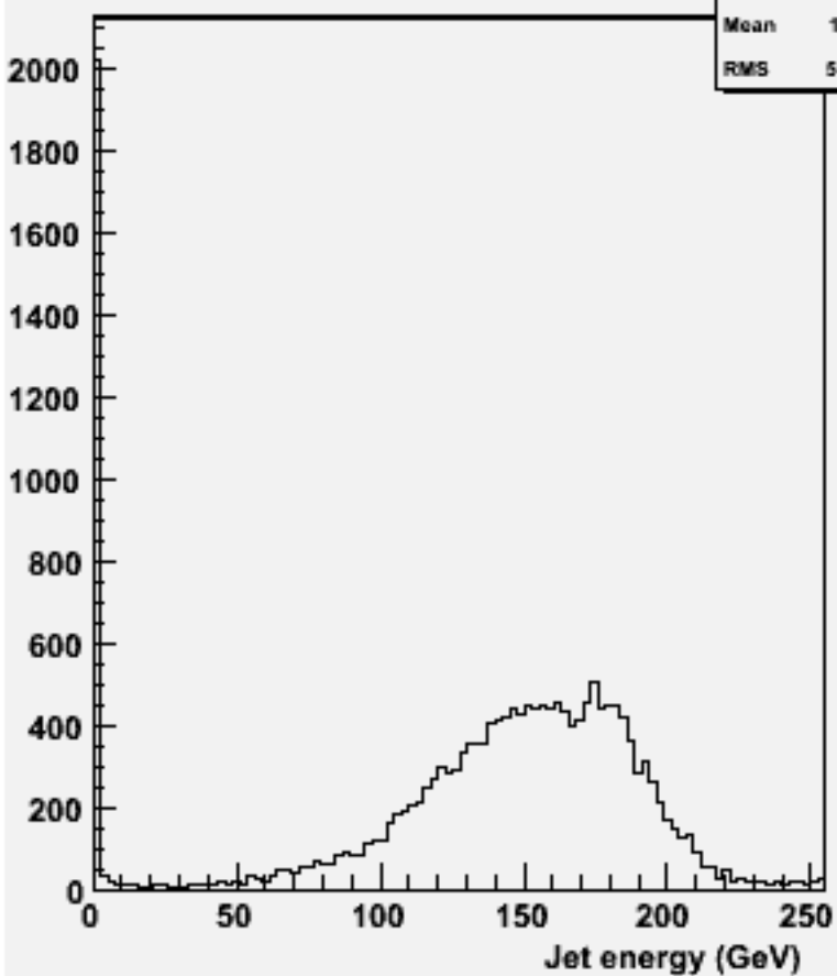
energy for 2-jets :w102565 e2e2e3e3dd_o
