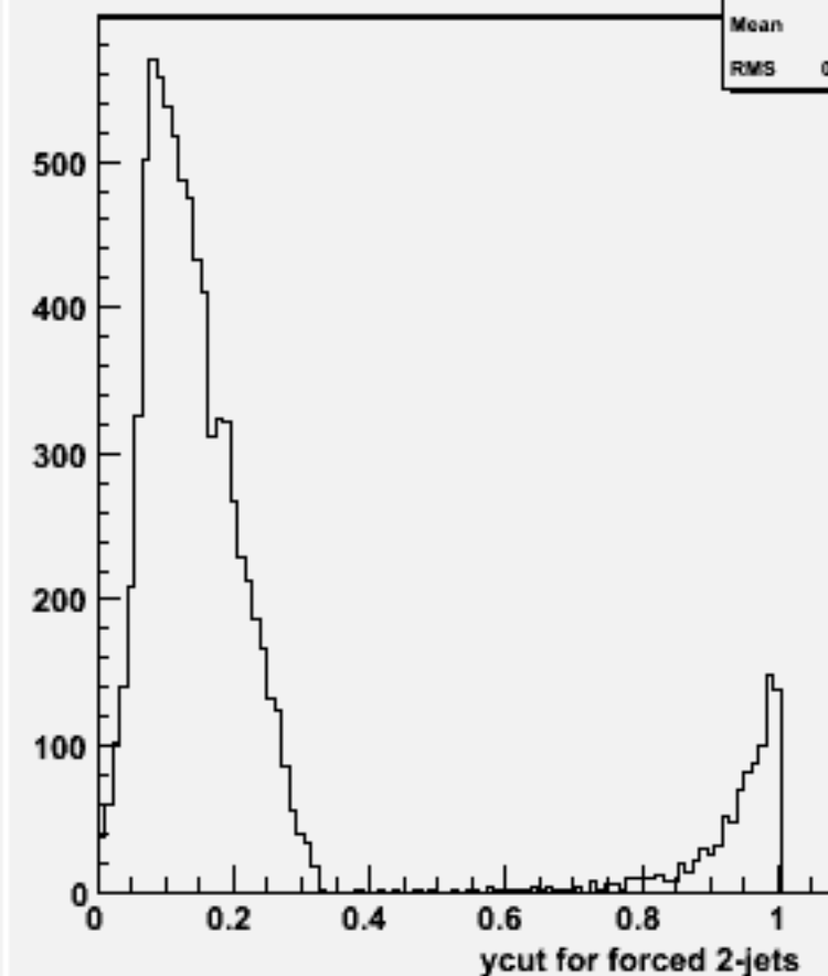
Ycut for 2-jets :w102564 e2e2e3e3dd_o
