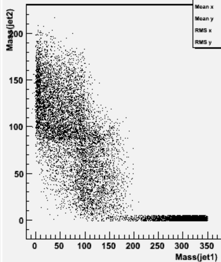
Jet mass for forced 2-jets : w102564 e2e2e3e3dd_o
