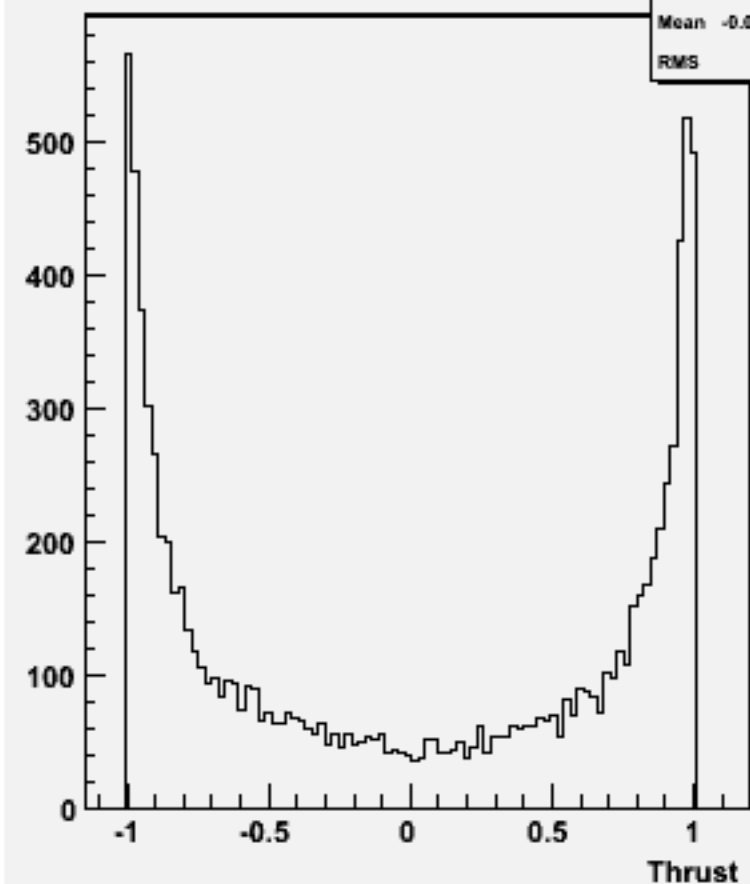
cos \Theta (thrust) w102564 e2e2e3e3dd_o
