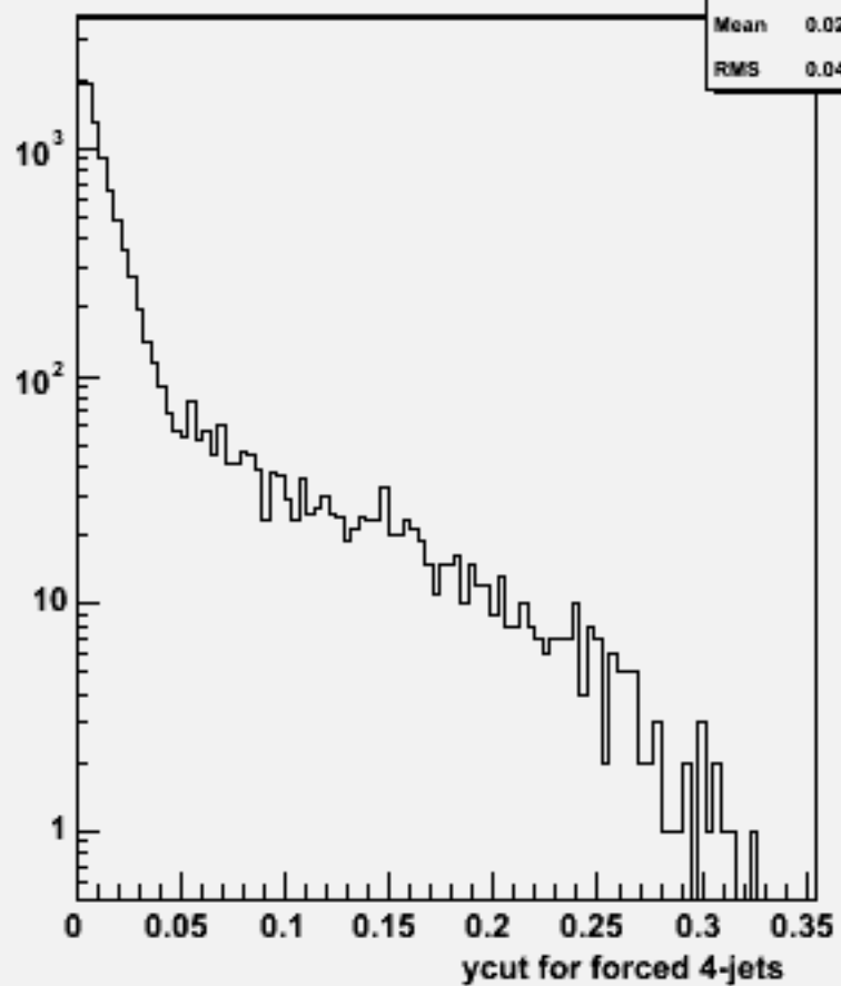
Ycut for 4-jets :w102564 e2e2e3e3dd_o
