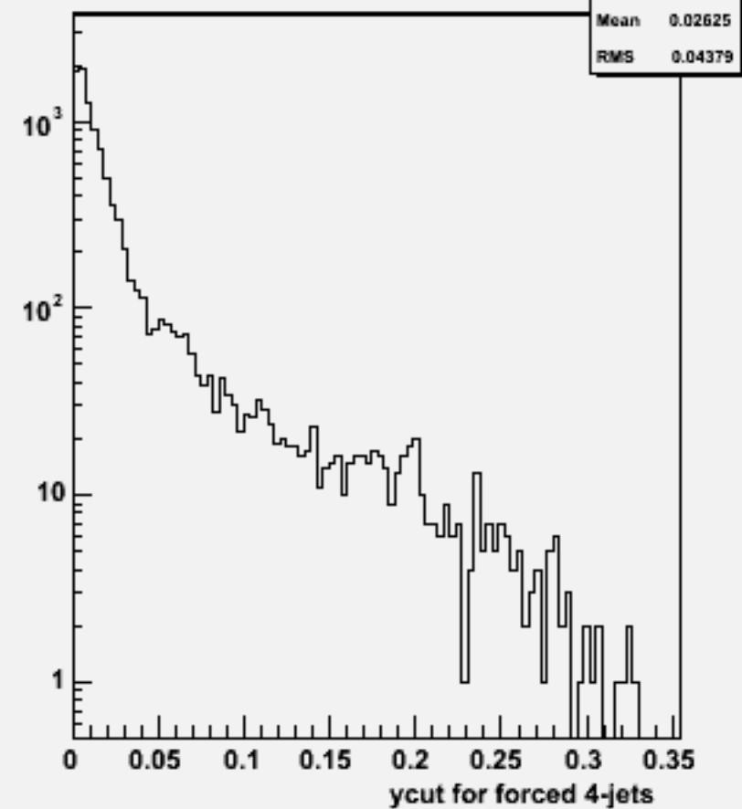
Ycut for 4-jets :w102557 e2e2e2e2bb_o
