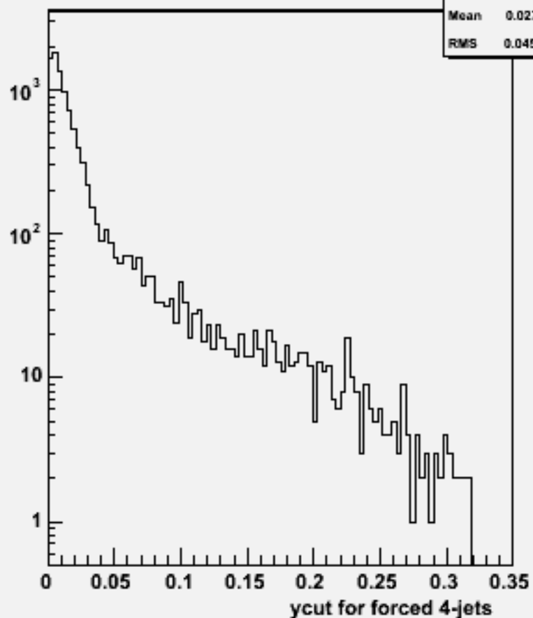
Ycut for 4-jets :w102556 e2e2e2e2bb_o
