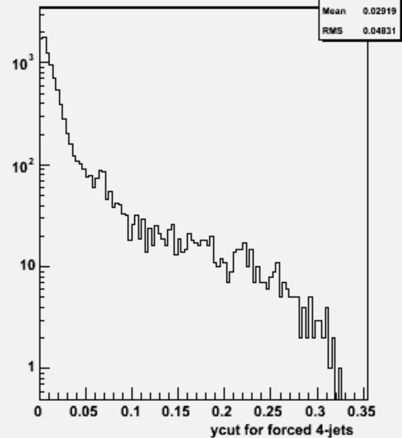
Ycut for 4-jets :w102552 e2e2e2e2ss_o
