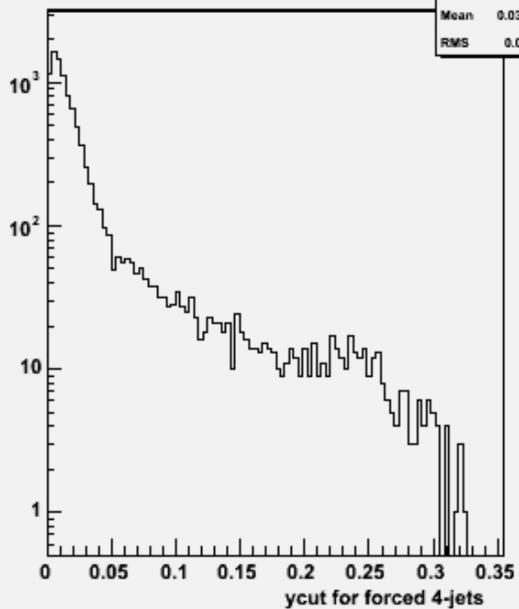
Ycut for 4-jets :w102534 e1e1ssbb_o
