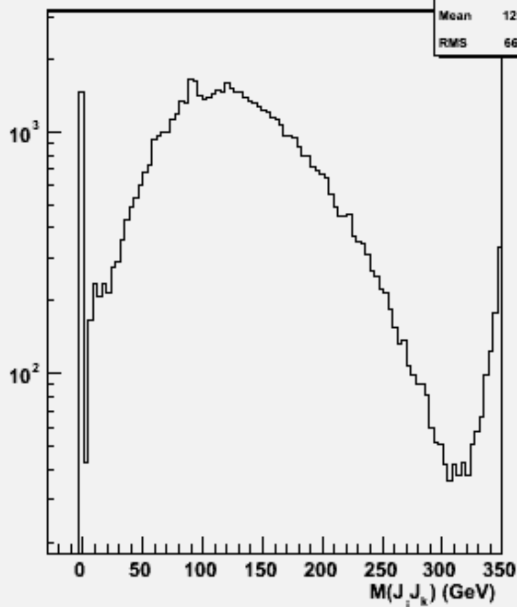
2jets mass(All comb)w102534 e1e1ssbb_o
