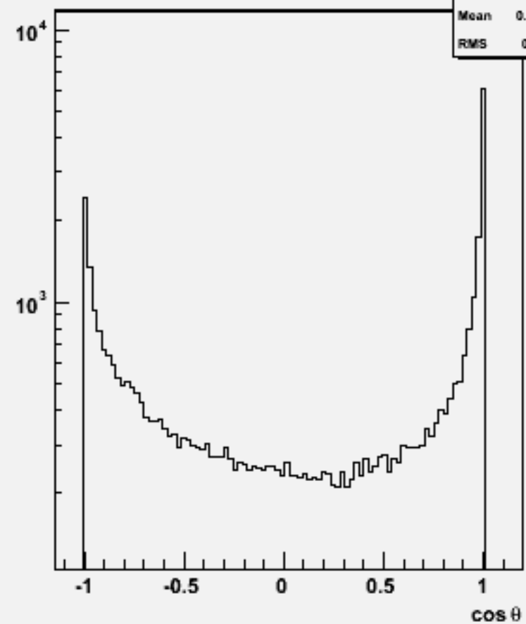
Jet cosθ (All jets)w102534 e1e1ssbb_o
