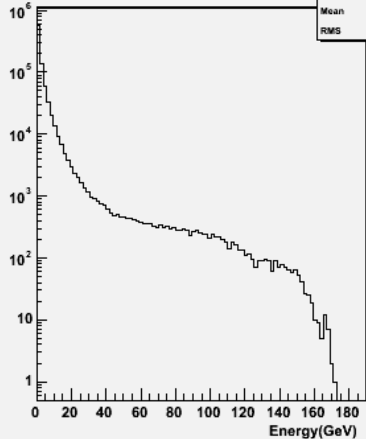
Particle Energy : w102534 e1e1ssbb_o
