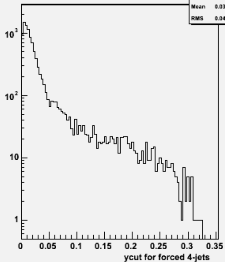
Ycut for 4-jets :w102533 e1e1ssbb_o
