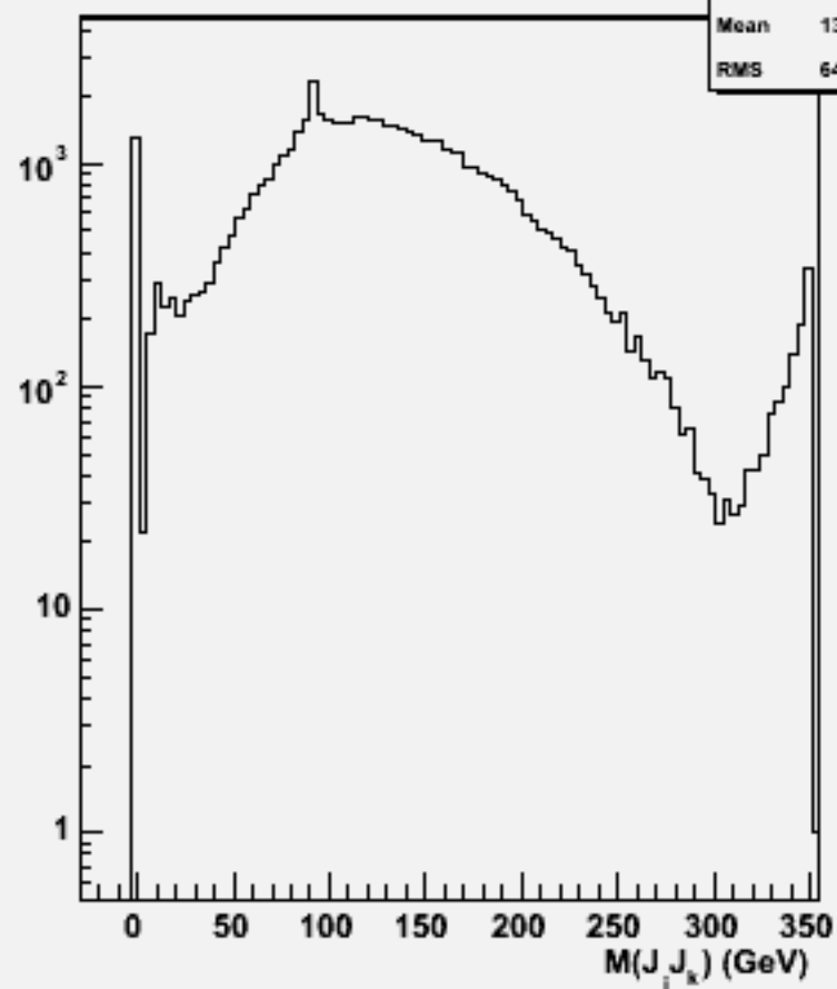
2jets mass(All comb)w102533 e1e1ssbb_o
