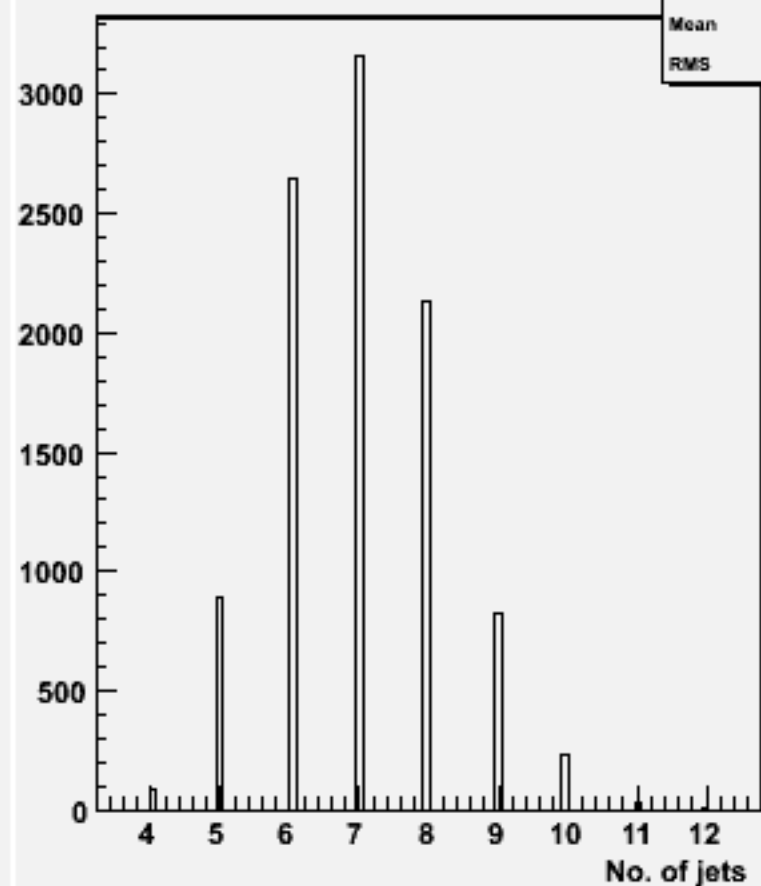
No. jets (ycut=0.001) : w102529 e1e1ssss_o
