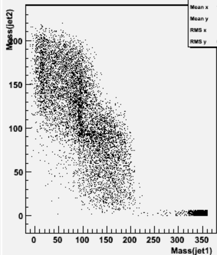
Jet mass for forced 2-jets : w102529 e1e1ssss_o
