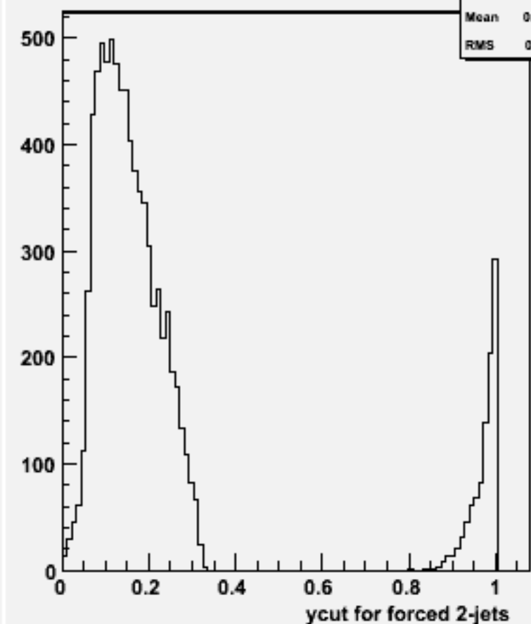
Ycut for 2-jets :w102529 e1e1ssss_o
