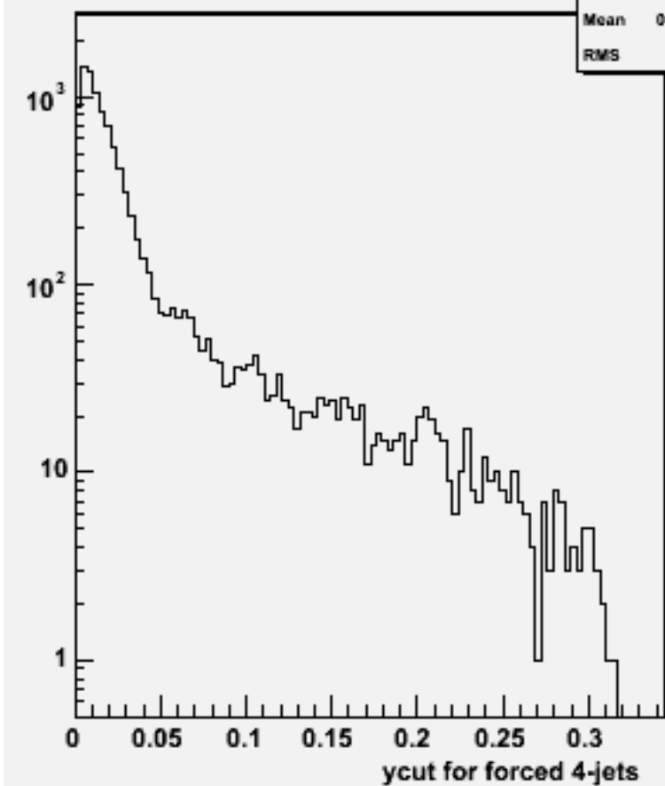
Ycut for 4-jets :w102529 e1e1ssss_o
