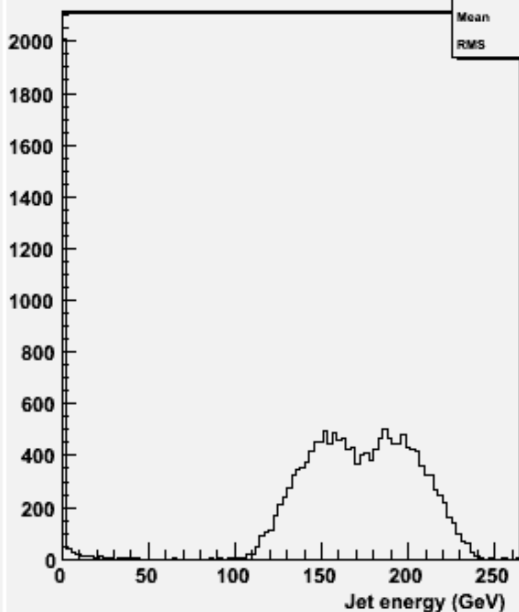
energy for 2-jets :w102529 e1e1ssss_o
