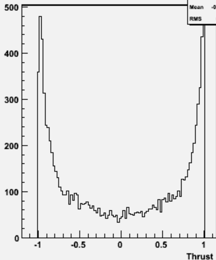
cos \Theta (thrust) w102529 e1e1ssss_o
