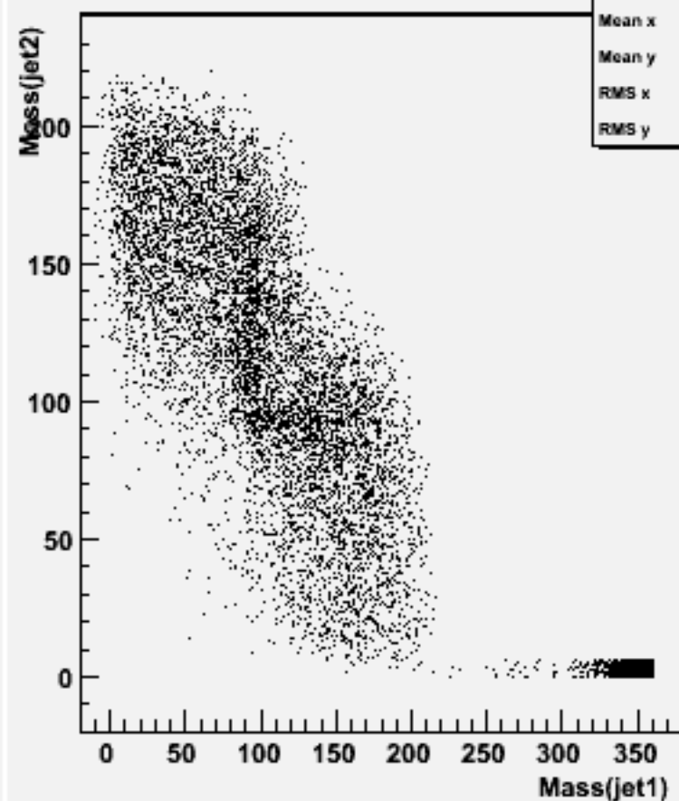
Jet mass for forced 2-jets : w102528 e1e1ssss_o
