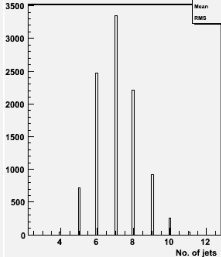
No. jets (ycut=0.001) : w102528 e1e1ssss_o
