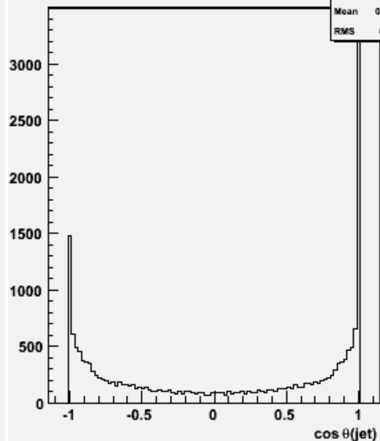
cos \theta for 2-jets :w102528 e1e1ssss_o
