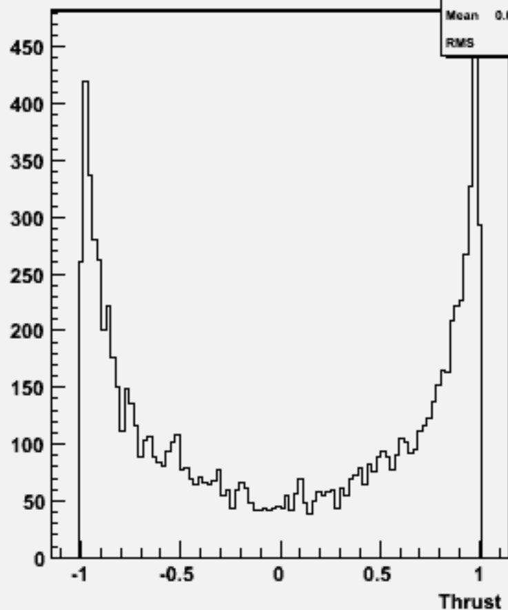
cos \Theta (thrust) w102528 e1e1ssss_o
