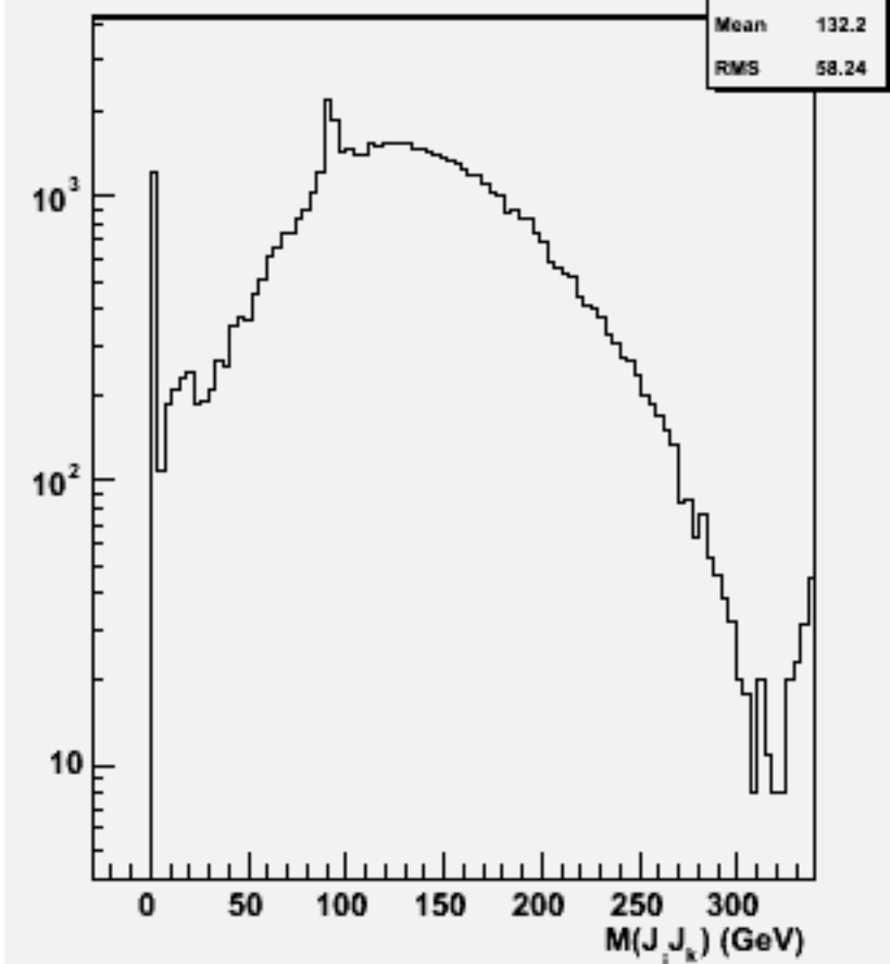
2jets mass(All comb)w102528 e1e1ssss_o
