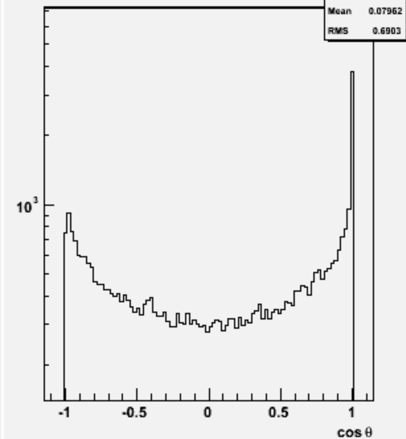
Jet cosθ (All jets)w102528 e1e1ssss_o
