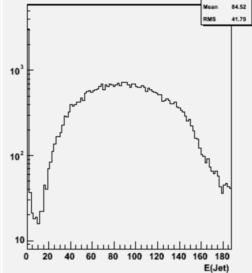
Jet energies(All jets)w102528 e1e1ssss_o
