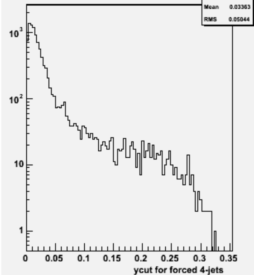
Ycut for 4-jets :w102528 e1e1ssss_o
