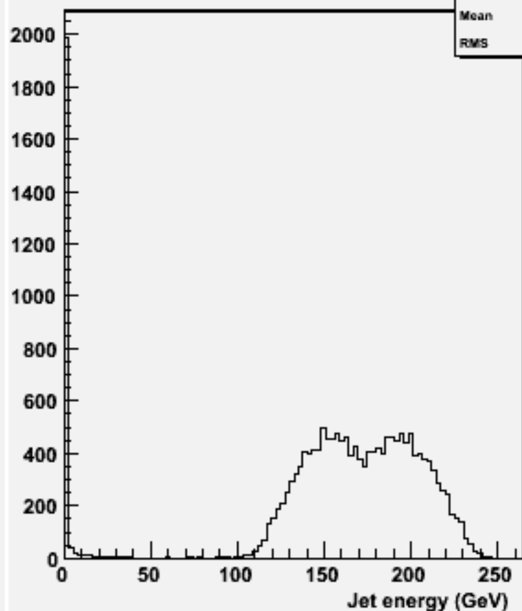
energy for 2-jets :w102528 e1e1ssss_o
