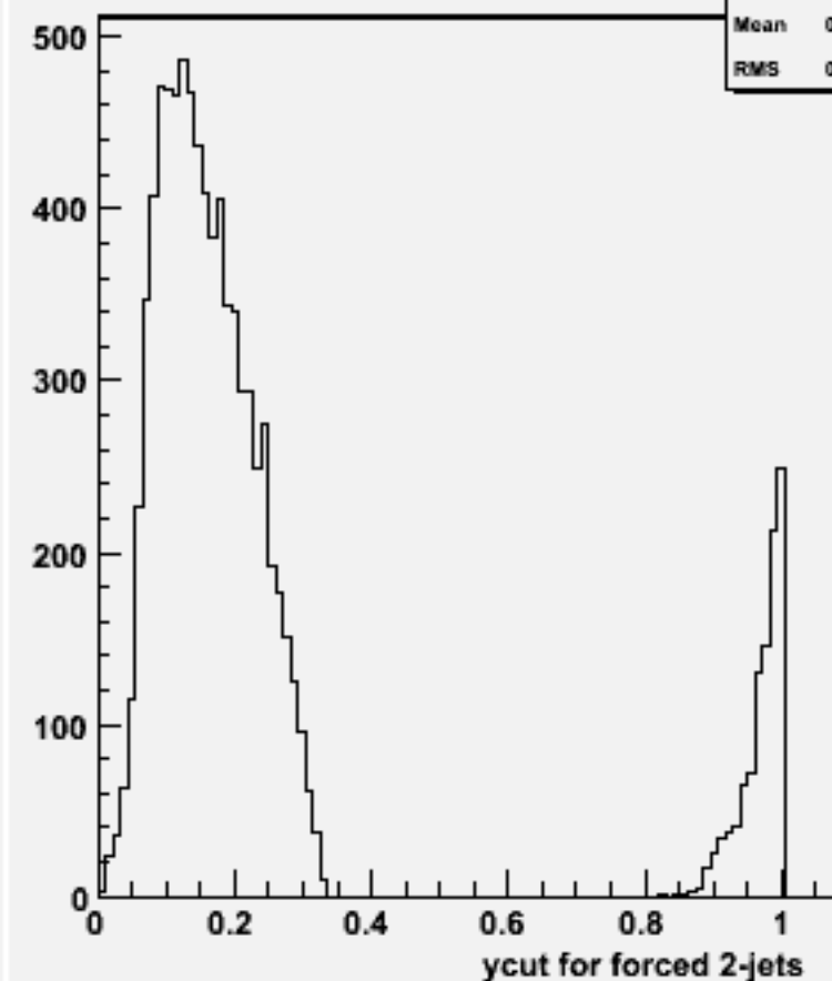
Ycut for 2-jets :w102528 e1e1ssss_o
