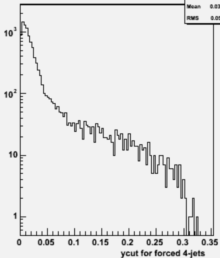
Ycut for 4-jets :w102525 e1e1ddb_o
