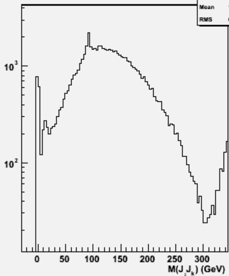
2jets mass(All comb)w102525 e1e1ddb_o
