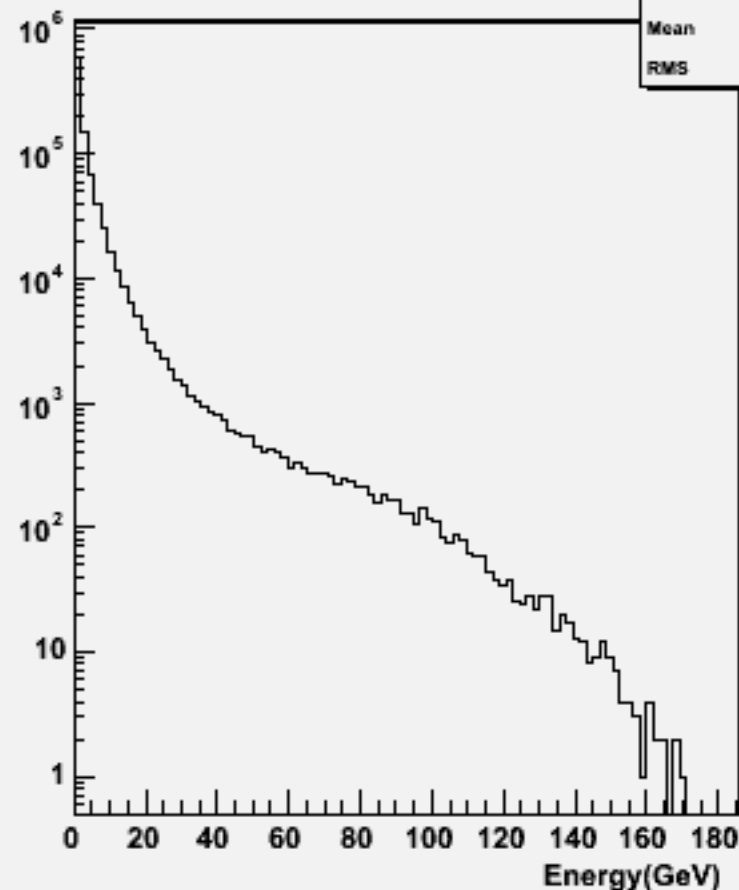
Particle Energy : w102525 e1e1ddb_o
